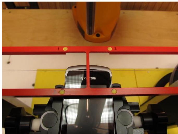
Figure 1b – HAC T-Coil Test Setup
