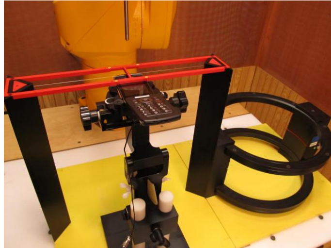
Figure 1a – HAC T-Coil Test Setup
