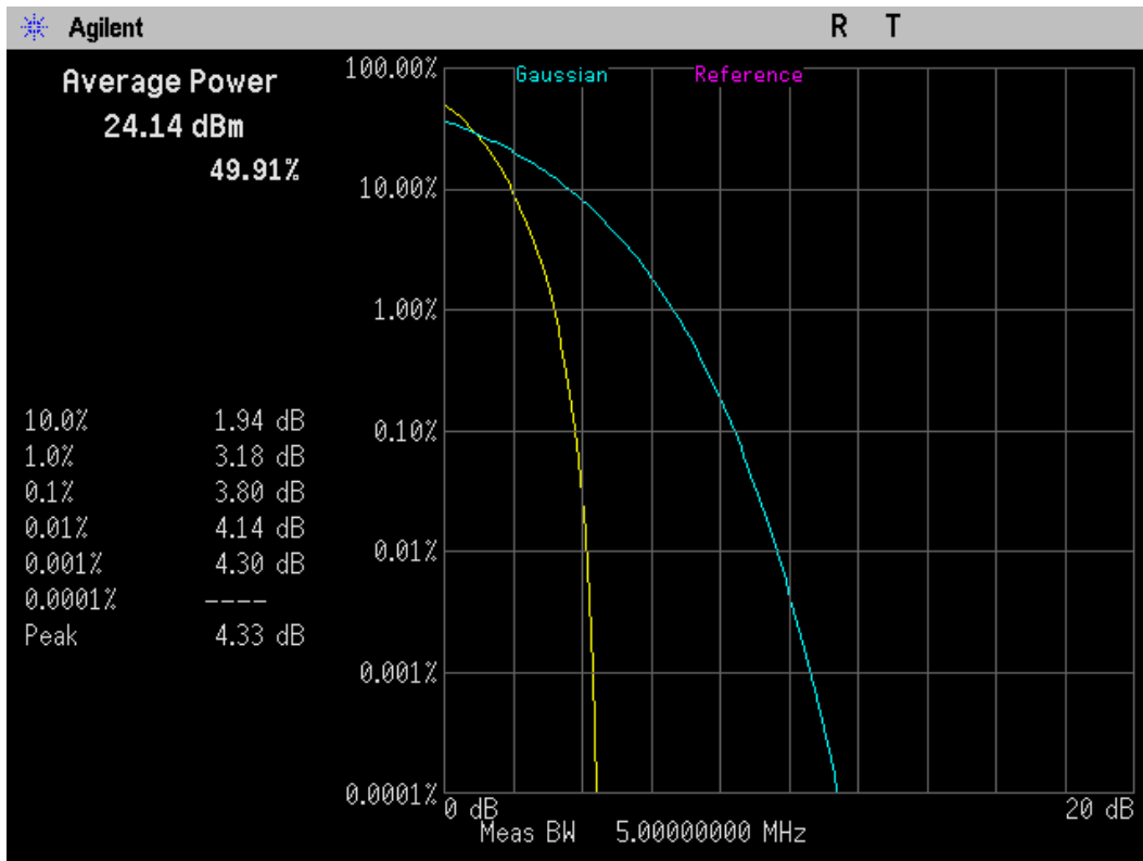
Figure 8-2 CCDF @ CH 600
