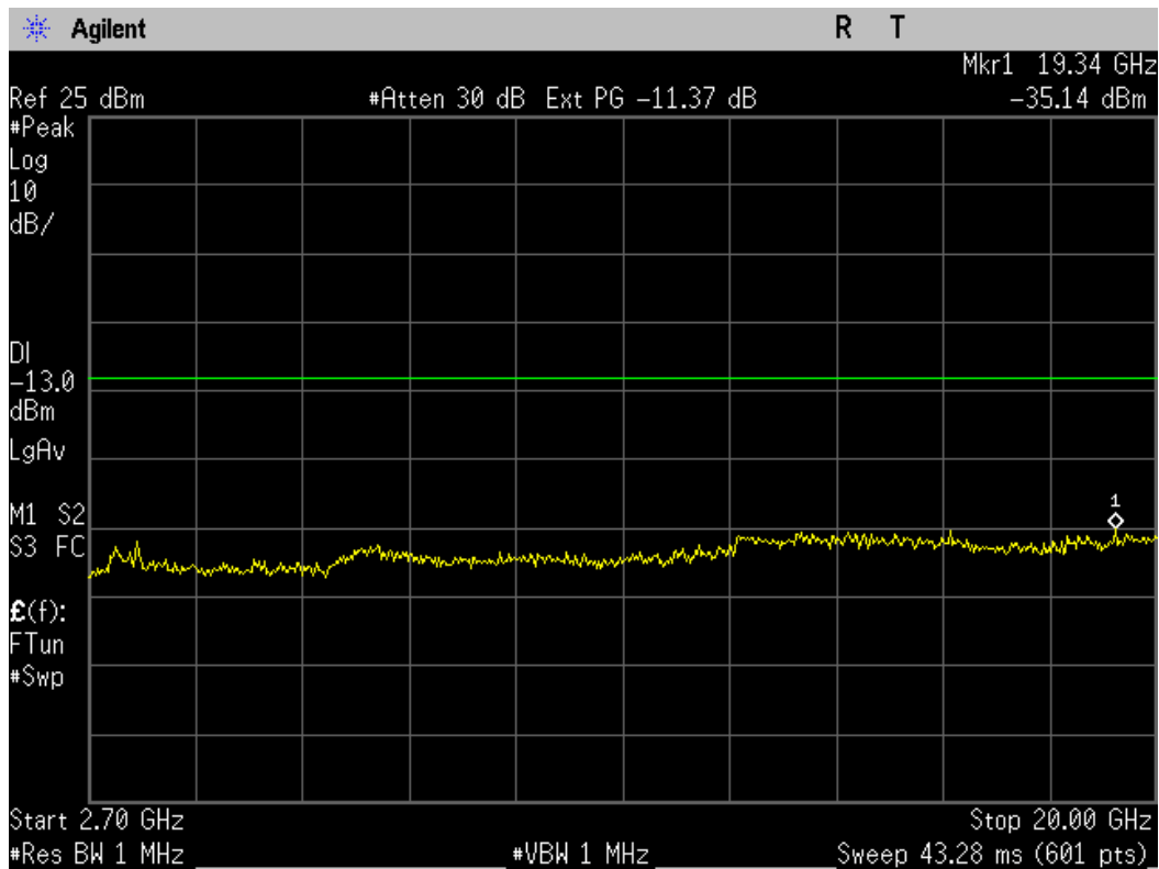
Figure 10-5b AWS 1700 - Conducted Spurious Emission (CH 450)
