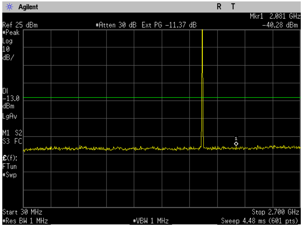
Figure 10-6a AWS 1700 - Conducted Spurious Emission (CH 875)
