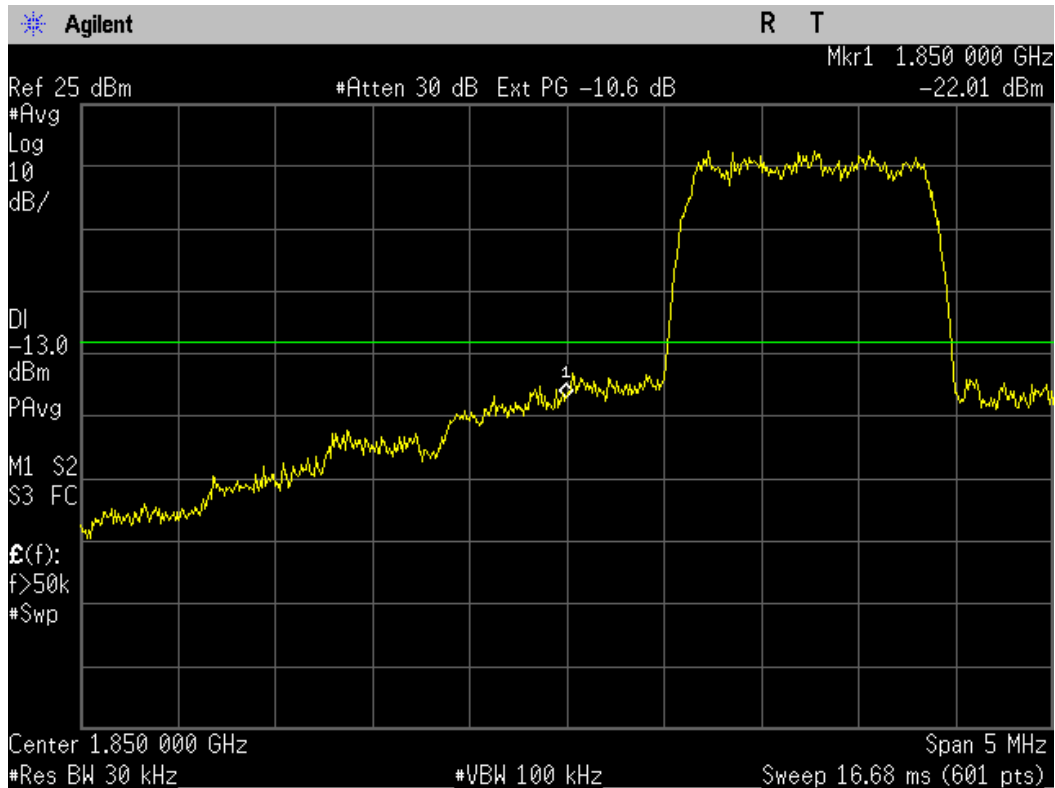
-Figure 9-8 CDMA 1900 Lower Band Edge @ CH 25
