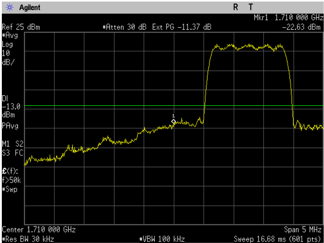
Figure 9-5 AWS 1700 Lower Band Edge @ CH 25
