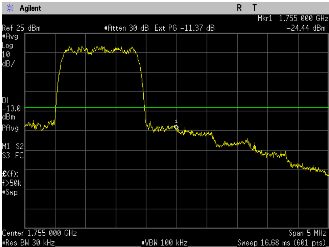
Figure 9-6 AWS 1700 Upper Band Edge @ CH 875
