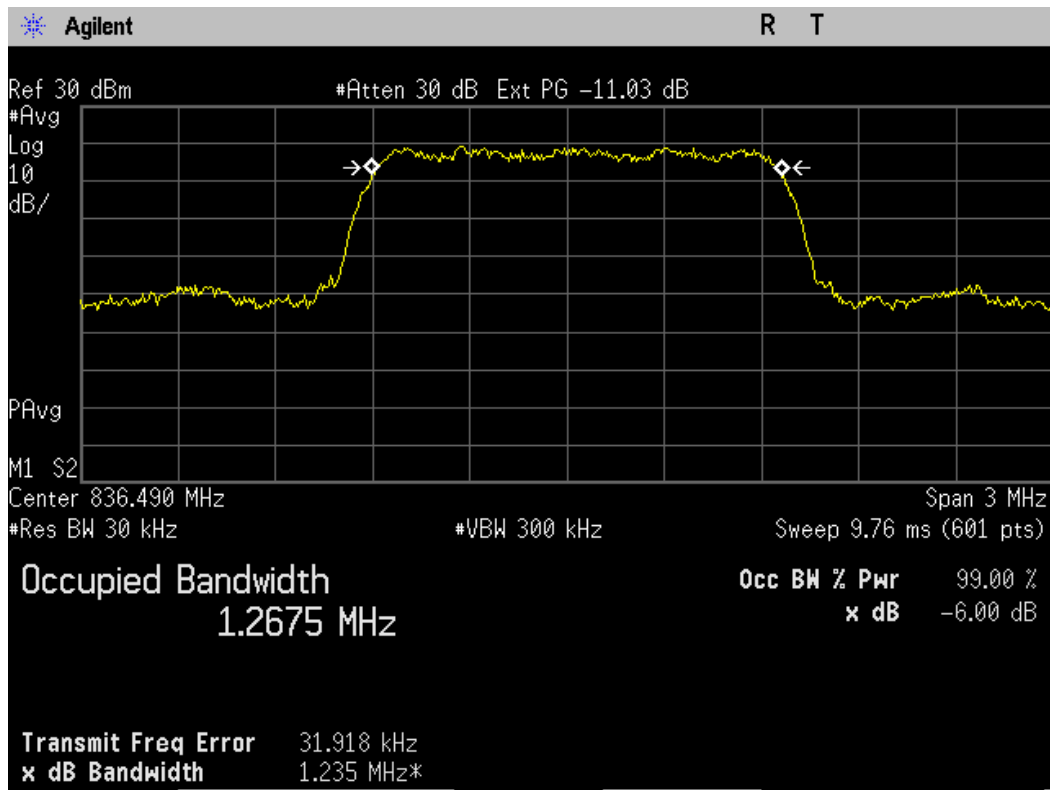
Figure 9-1 CDMA 800 @ CH 384
