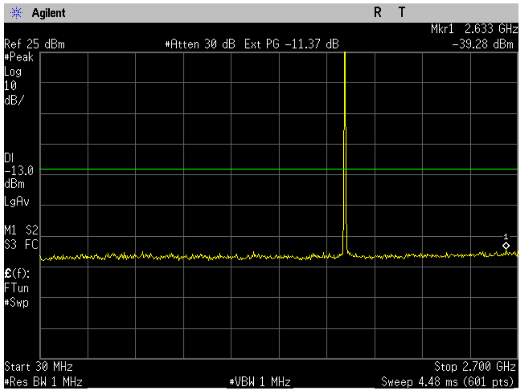
Figure 10-5a AWS 1700 - Conducted Spurious Emission (CH 450)
