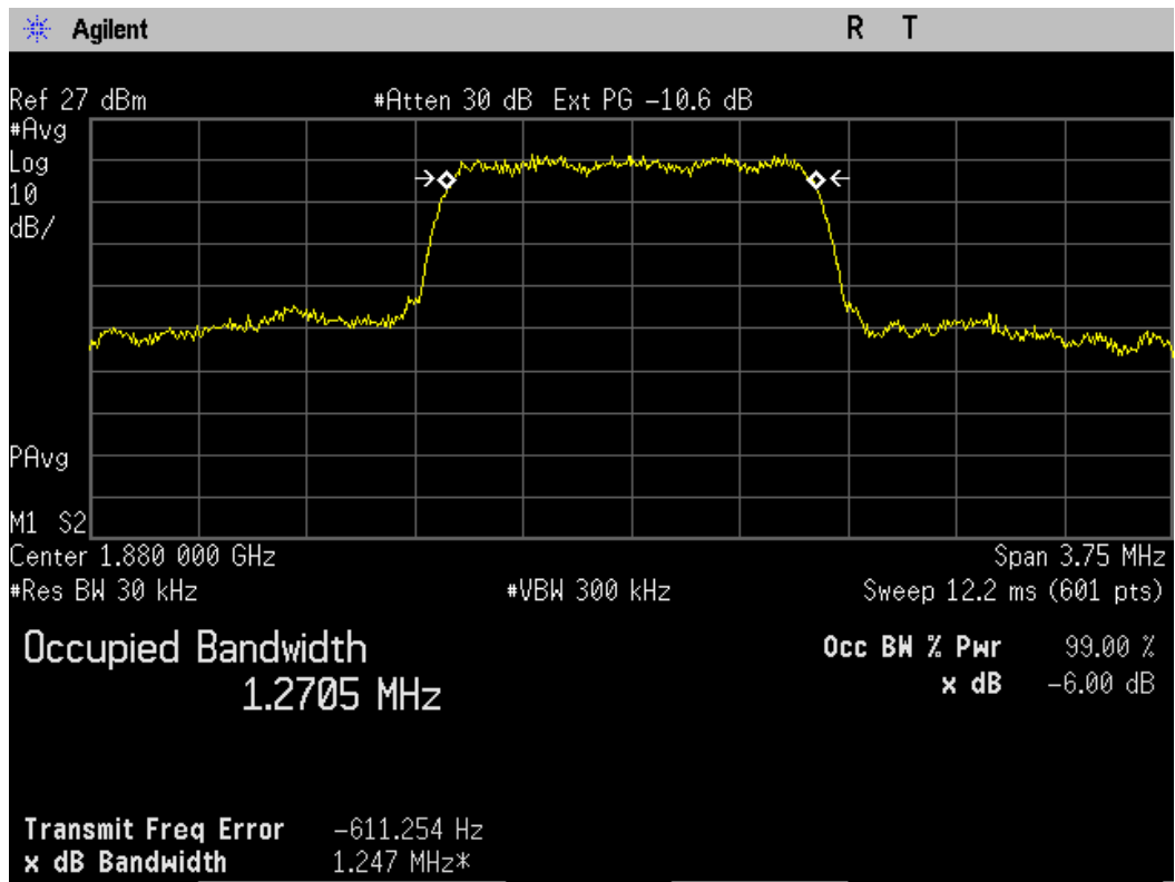
Figure 9-7 CDMA 1900 @ CH 600
