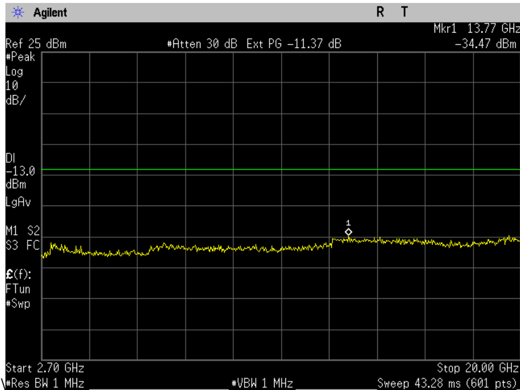
Figure 10-4b AWS 1700 - Conducted Spurious Emission (CH 25)
