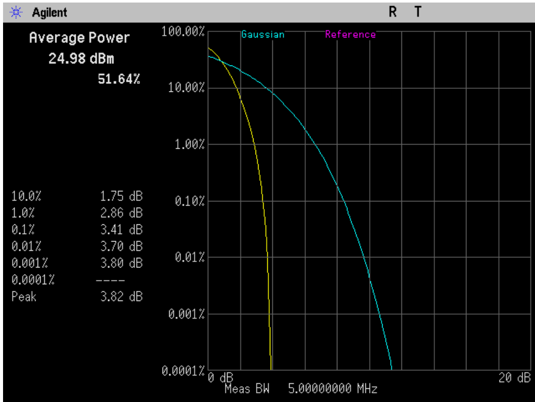
Figure 8-1 CCDF @ CH 450
