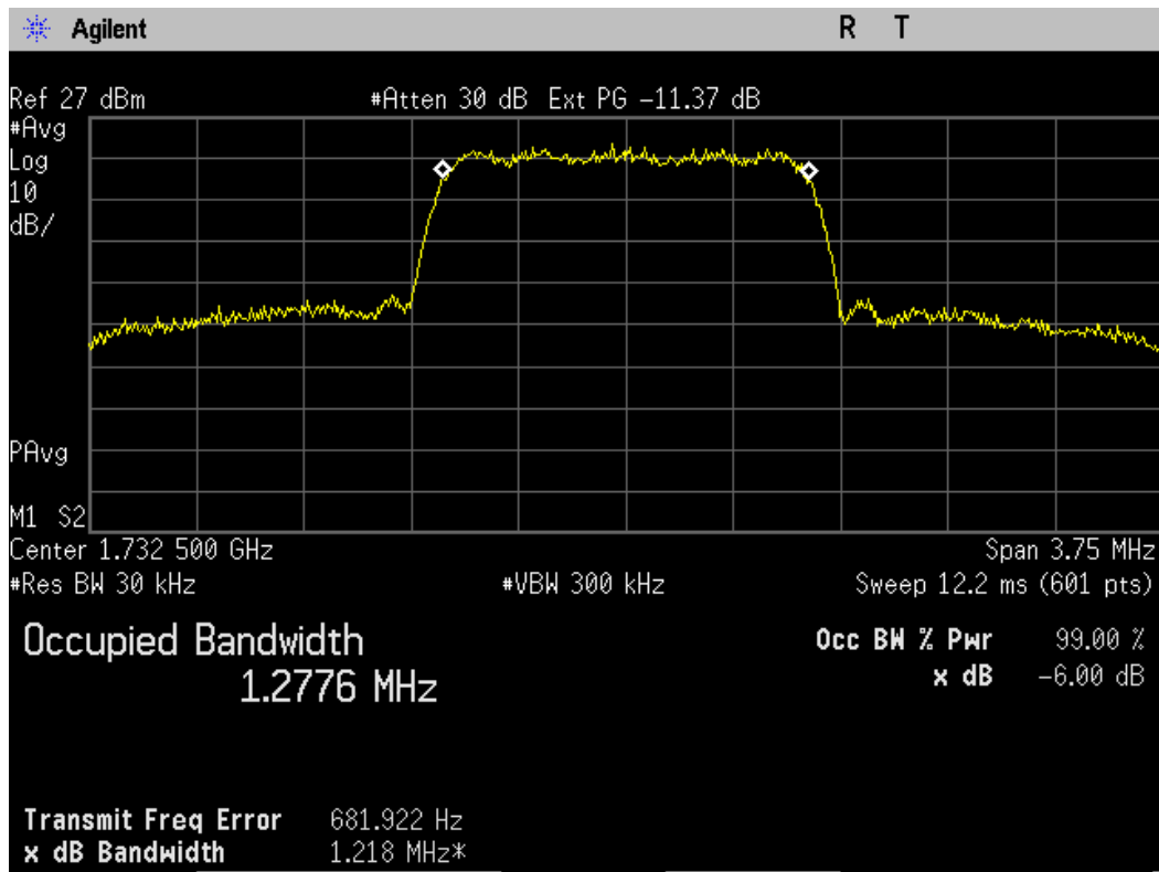
Figure 9-4 AWS 1700 @ CH 450
