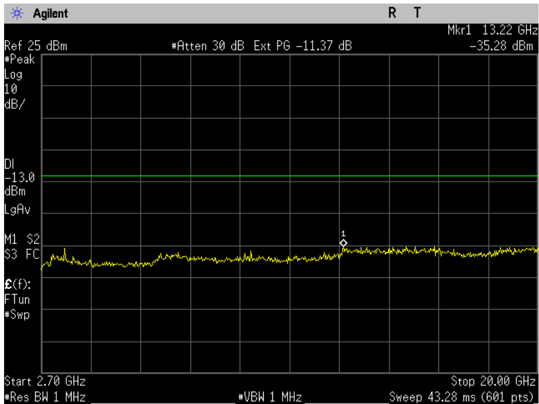
Figure 10-6b AWS 1700 - Conducted Spurious Emission (CH 875)
