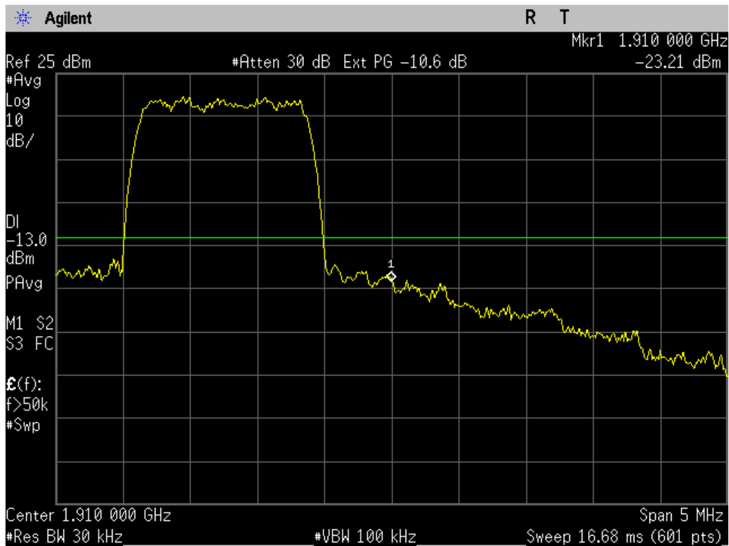
Figure 9-9 CDMA 1900 Upper Band Edge @ CH 1175
