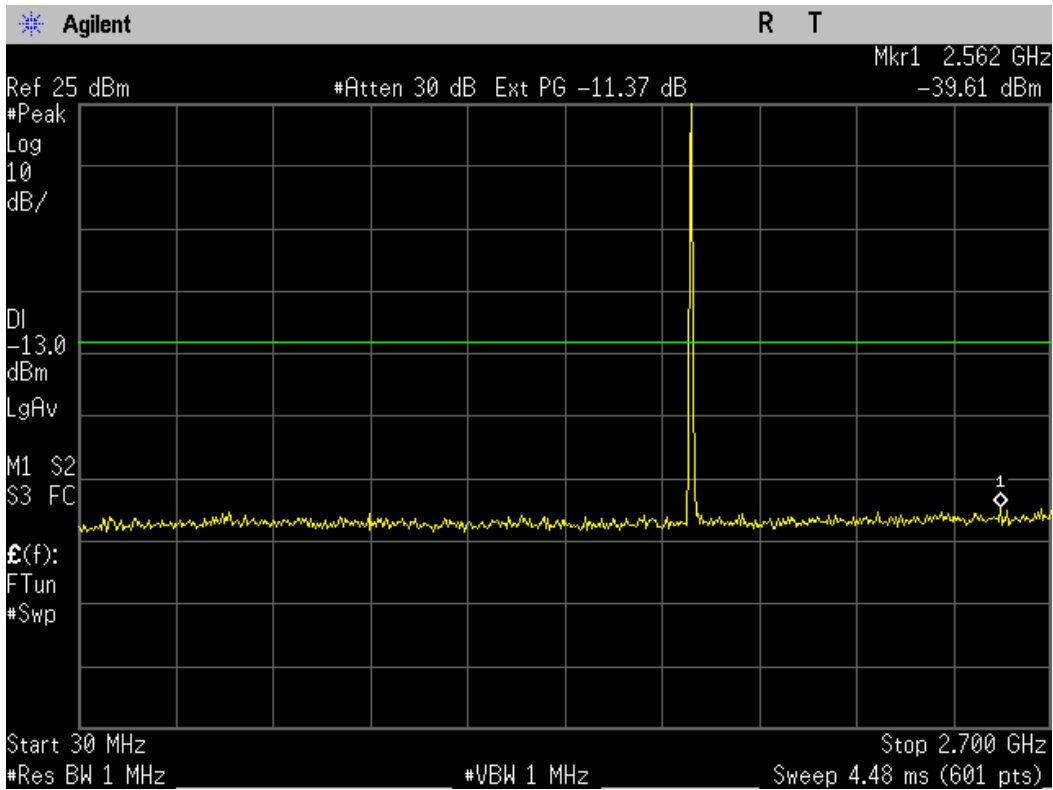
Figure 10-4a AWS 1700 - Conducted Spurious Emission (CH 25)
