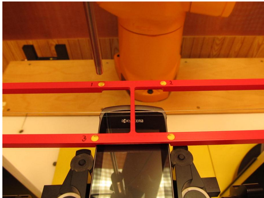
Figure 1b – HAC T-Coil Test Setup
