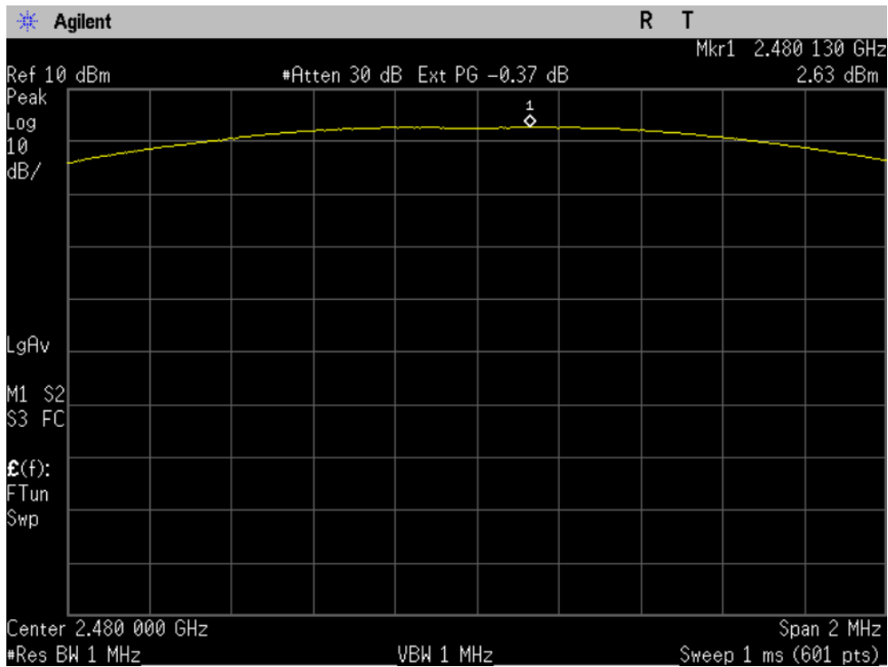
Figure 5-3a: Peak Output Power, EDR DQPSK Channel 78.
