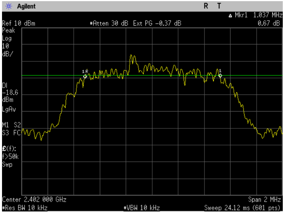
Figure 6-1c: 20dB Bandwidth EDR D8PSK, Channel 0.
