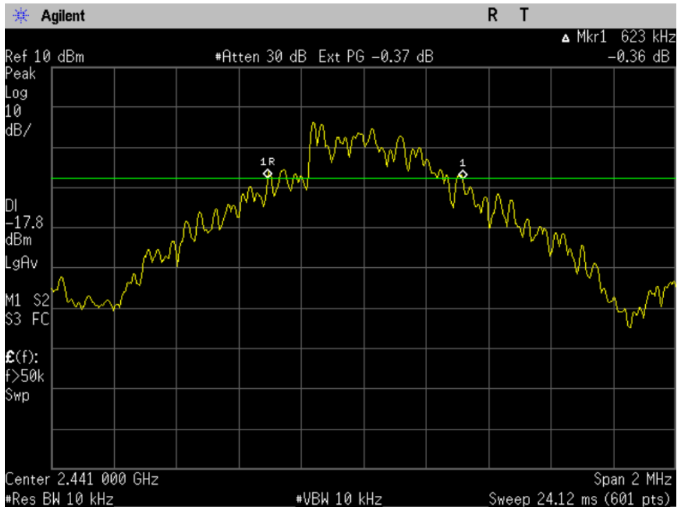
Figure 6-2a: 20dB Bandwidth Basic rate, Channel 39.
