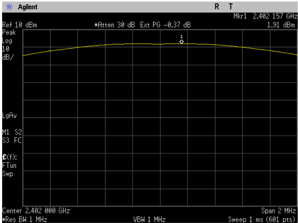
Figure 5-1a: Peak Output Power, EDR DQPSK Channel 0.
