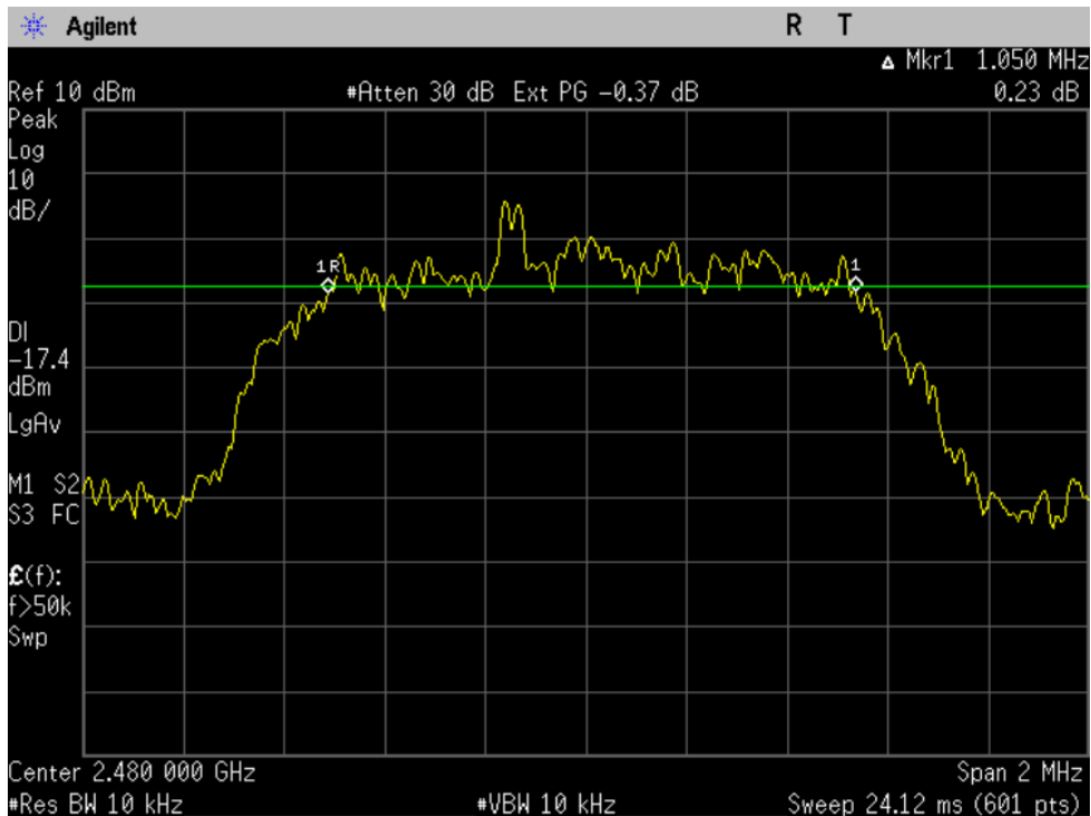
Figure 6-3b: 20dB Bandwidth EDR DQPSK, Channel 78.
