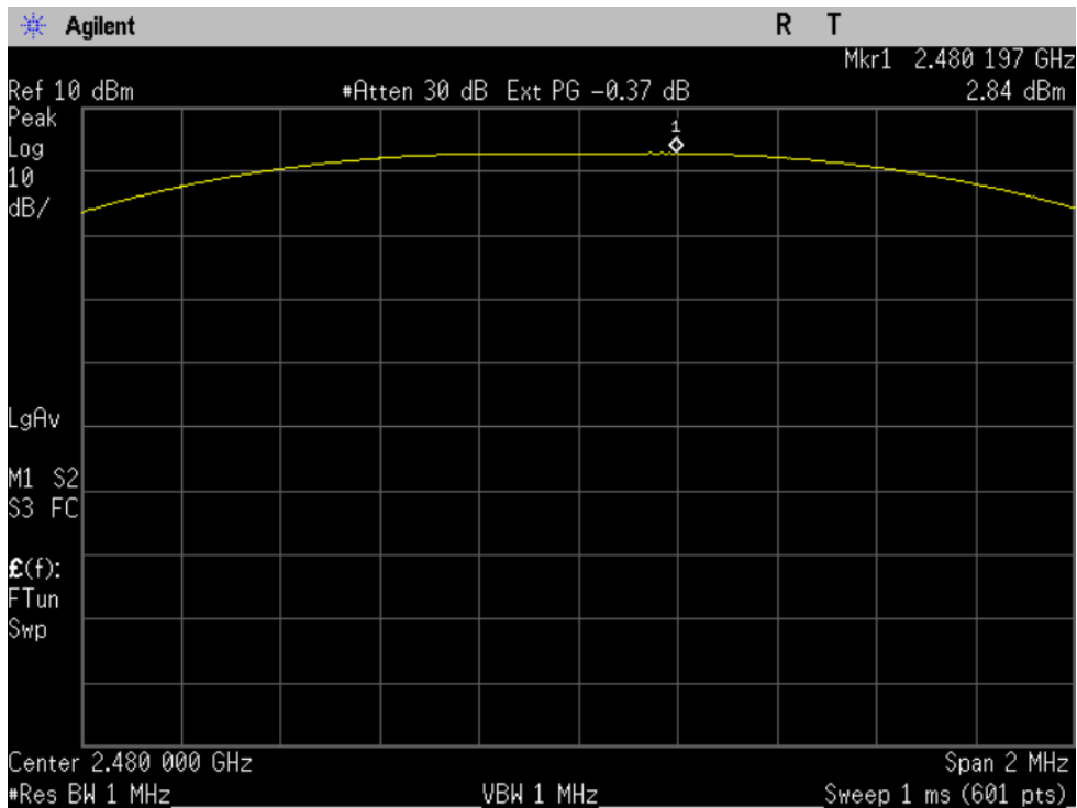
Figure 5-3: Peak Output Power, Channel 78.
