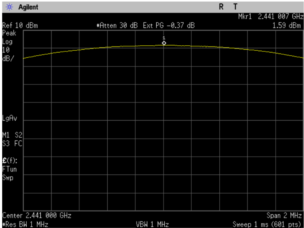
Figure 5-2b: Peak Output Power, EDR D8PSK Channel 39.
