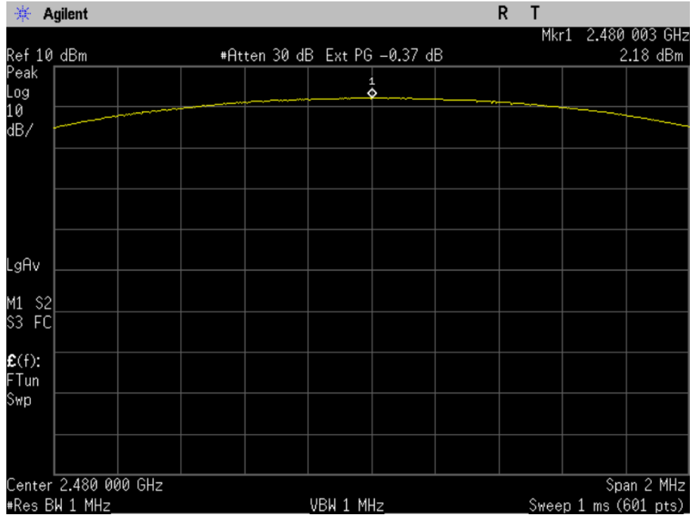
Figure 5-3b: Peak Output Power, EDR D8PSK Channel 78.
