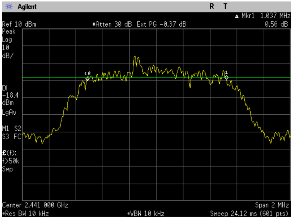
Figure 6-2c: 20dB Bandwidth EDR D8PSK, Channel 39.
