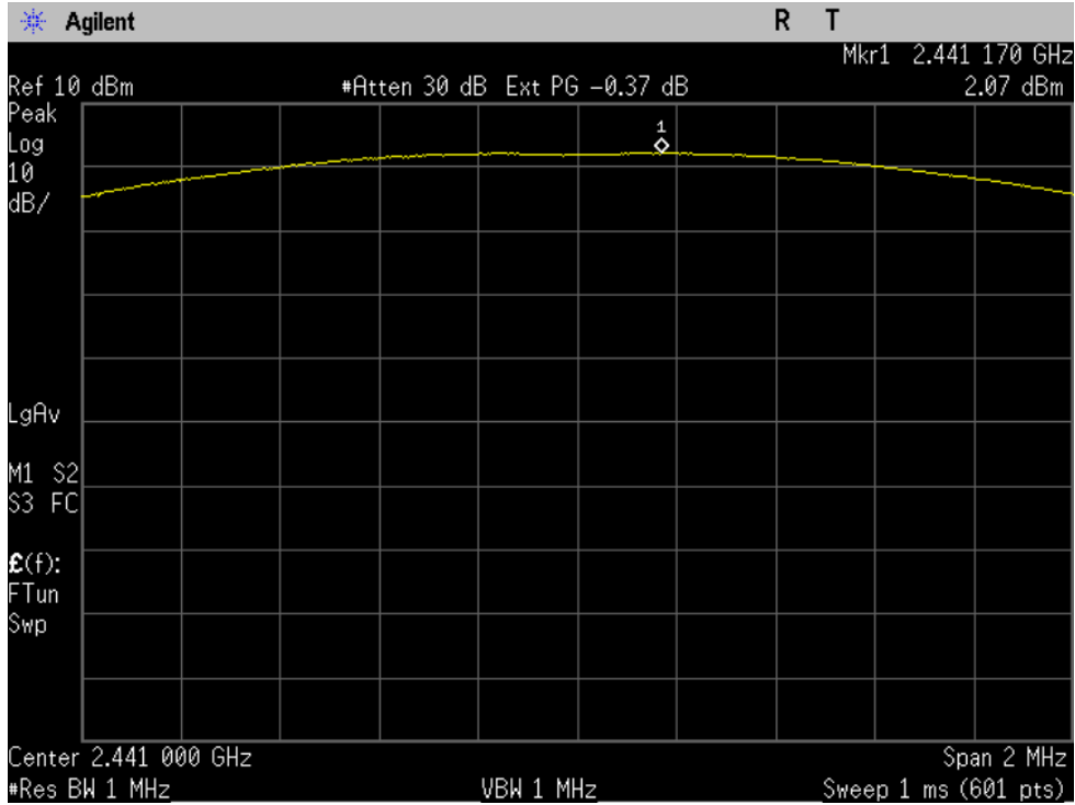
Figure 5-2a: Peak Output Power, EDR DQPSK Channel 39.
