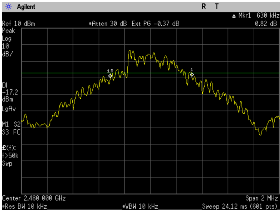
Figure 6-3a: 20dB Bandwidth Basic rate, Channel 78.
