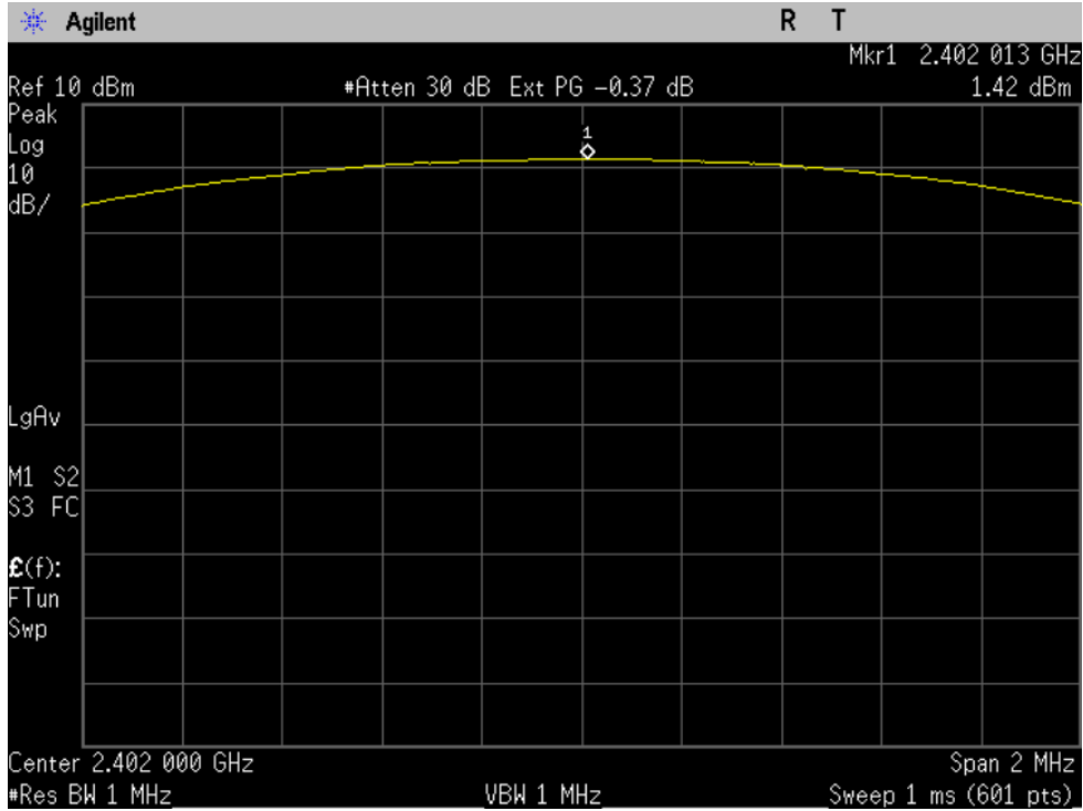
Figure 5-1b: Peak Output Power, EDR D8PSK Channel 0.
