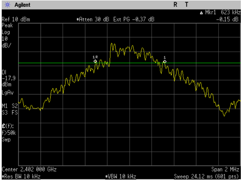
Figure 6-1a: 20dB Bandwidth Basic rate, Channel 0.
