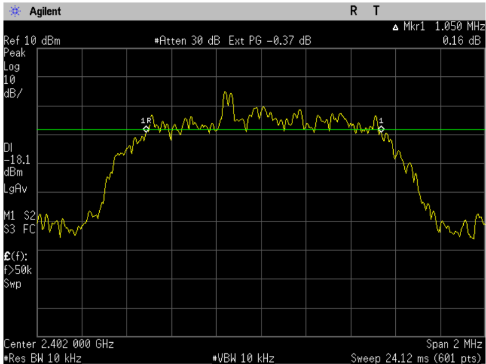
Figure 6-1b: 20dB Bandwidth EDR DQPSK, Channel 0.
