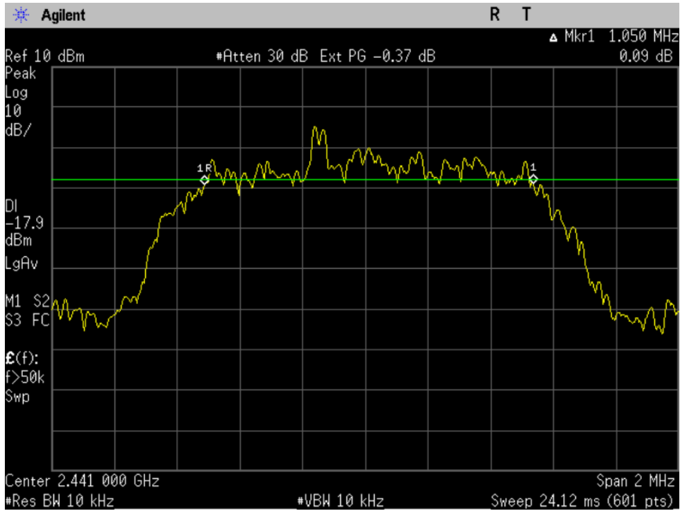
Figure 6-2b: 20dB Bandwidth EDR DQPSK, Channel 39.
