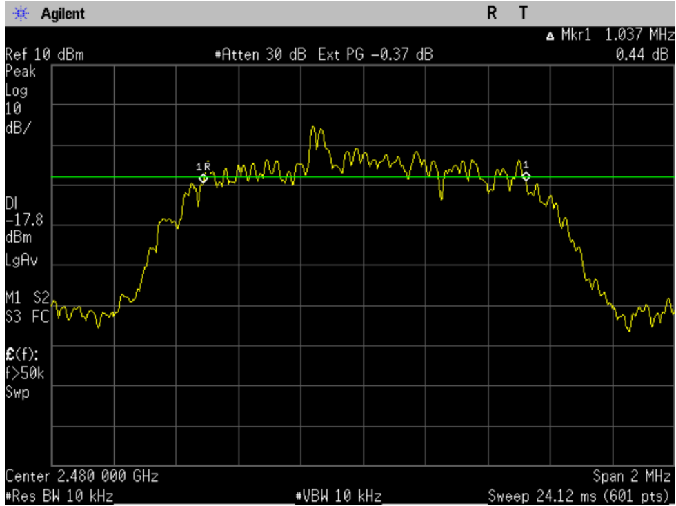
Figure 6-3c: 20dB Bandwidth EDR D8PSK, Channel 78.
