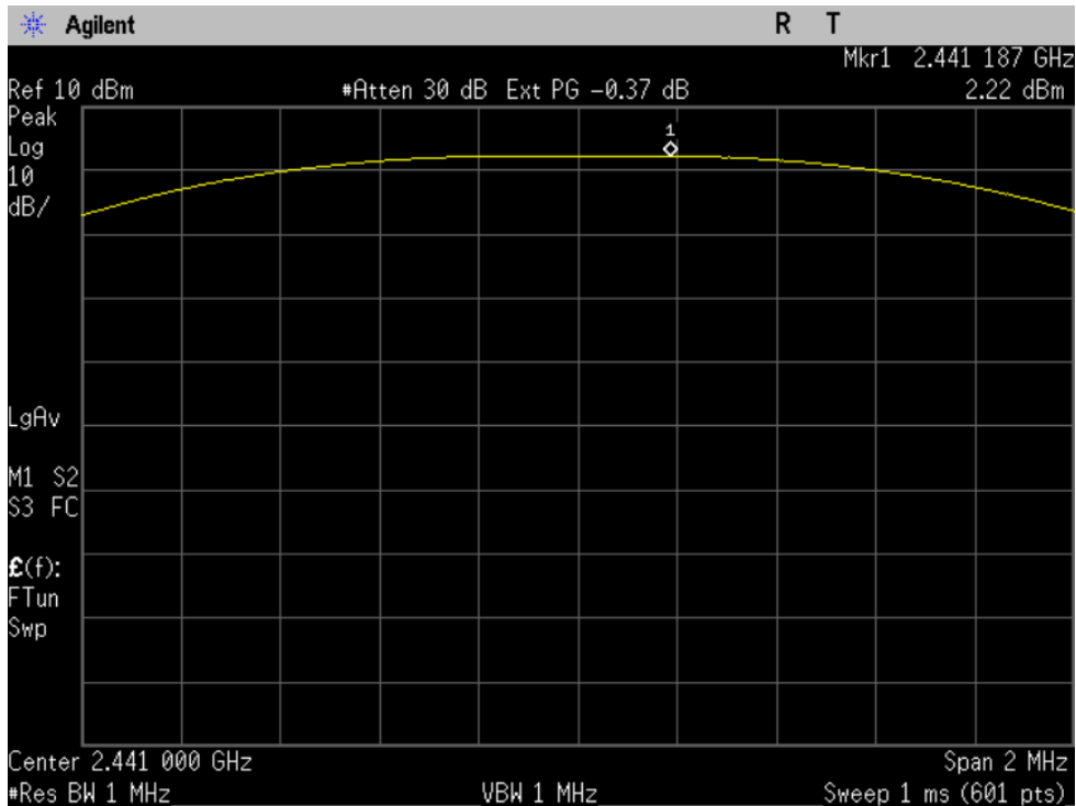
Figure 5-2: Peak Output Power, Channel 39.
