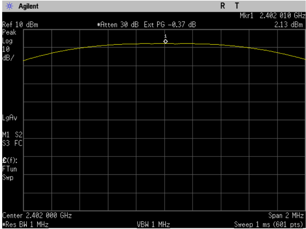
Figure 5-1: Peak Output Power, Basic Rate Channel 0.
