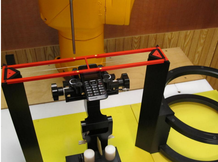
Figure 1a – HAC Tcoil Emission Test Setup
