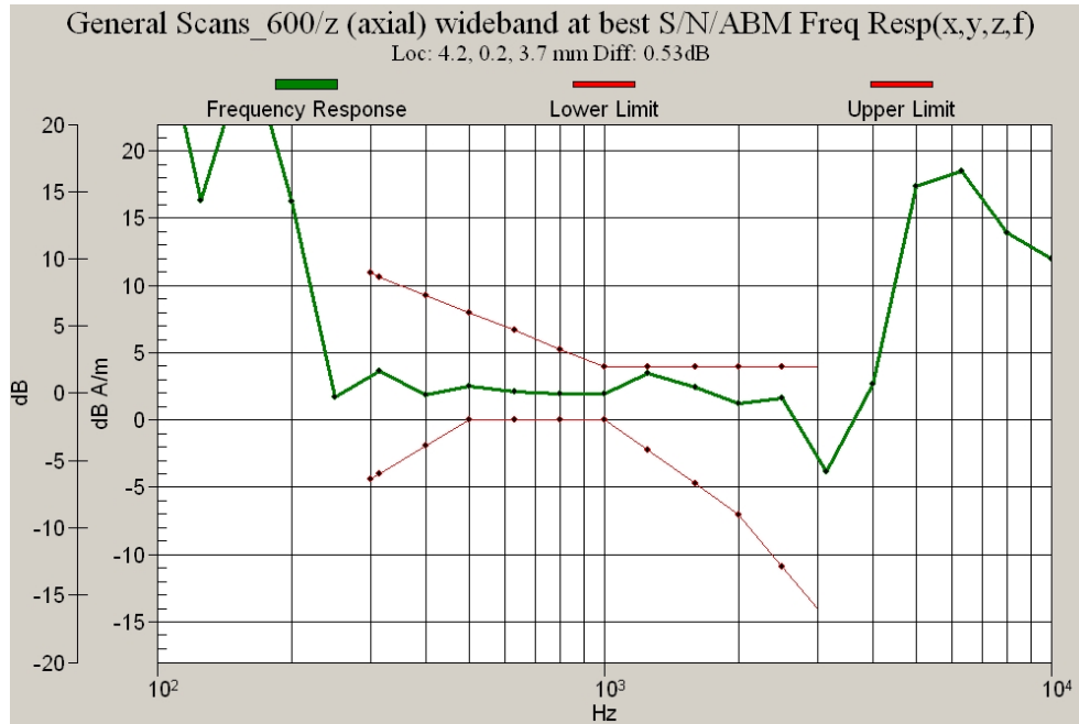
Figure 9.2a CDMA 1900 BC-1, Frequency Response
