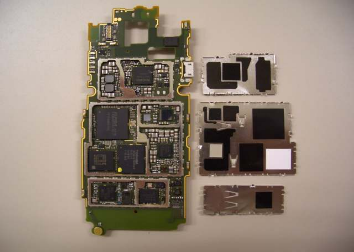
MAIN PCB L1 without Shield
