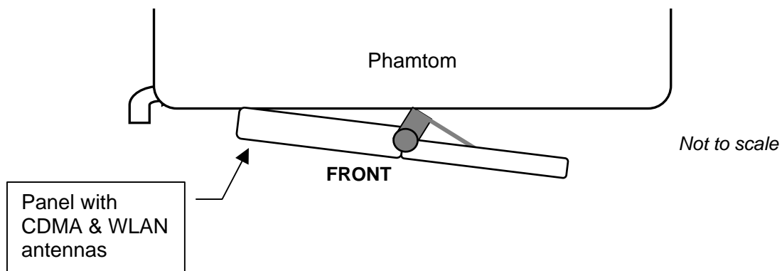
Figure 4.8 SAR Hand setup
