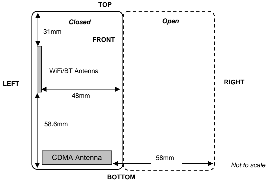
Figure 4.7 Antenna Distance to device edges
