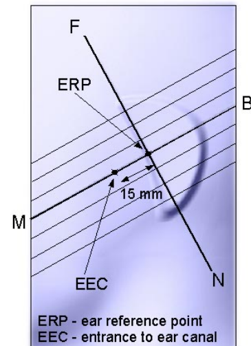
Figure 7-1b - Close up side view of phantom showing the ear region.
