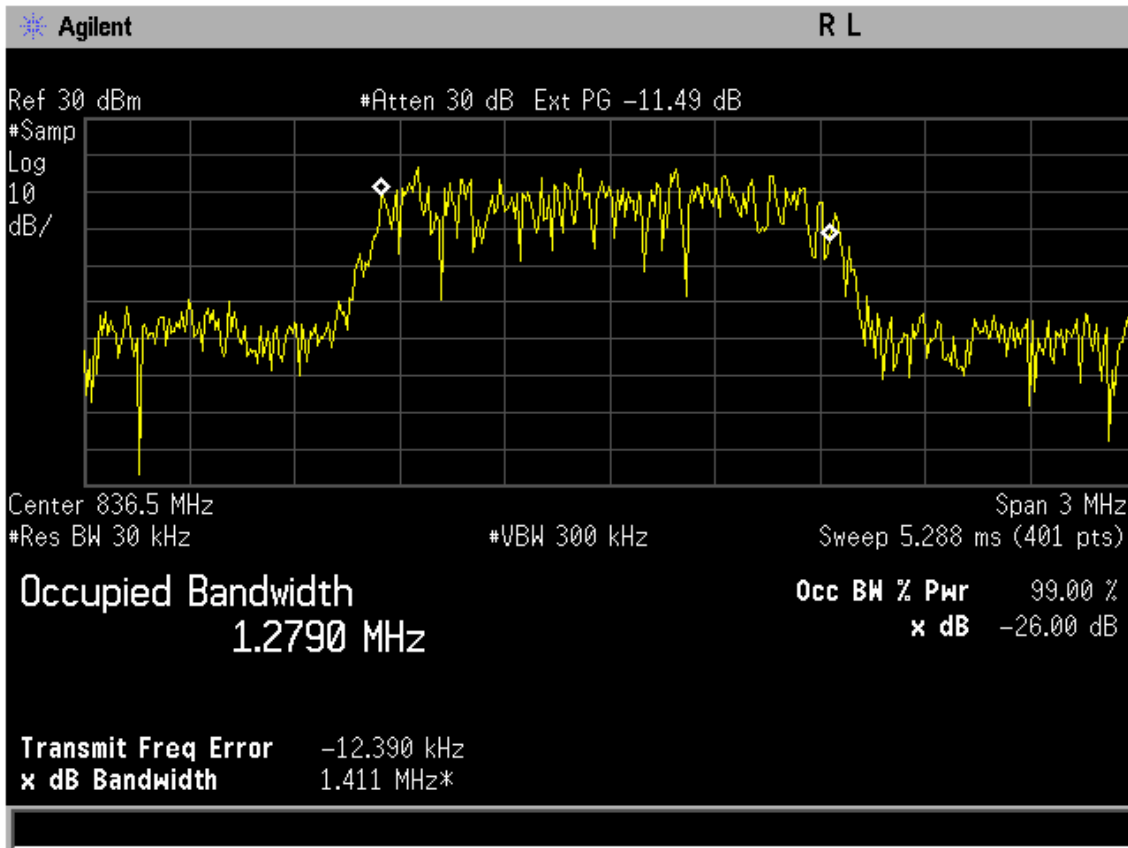
Figure 8-1 CDMA 800 @ CH 383
