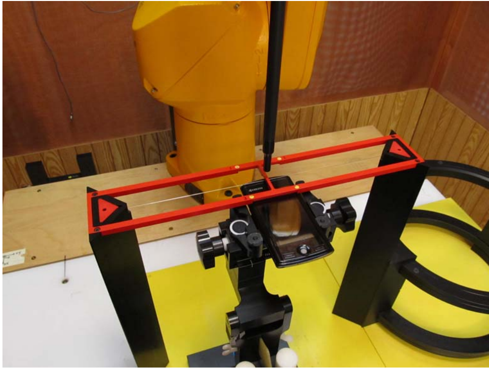
Figure 12D.1 HAC RF
