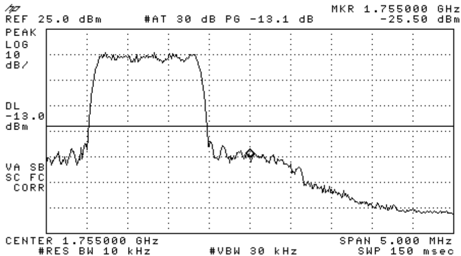
Figure 8-6 CDMA 1700 Upper Band Edge @ CH 875
