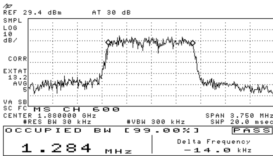
Figure 8-7 CDMA 1900 @ CH 600
