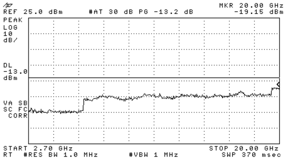
Figure 9-7b CDMA 1900 - Conducted Spurious Emission (CH 25)
