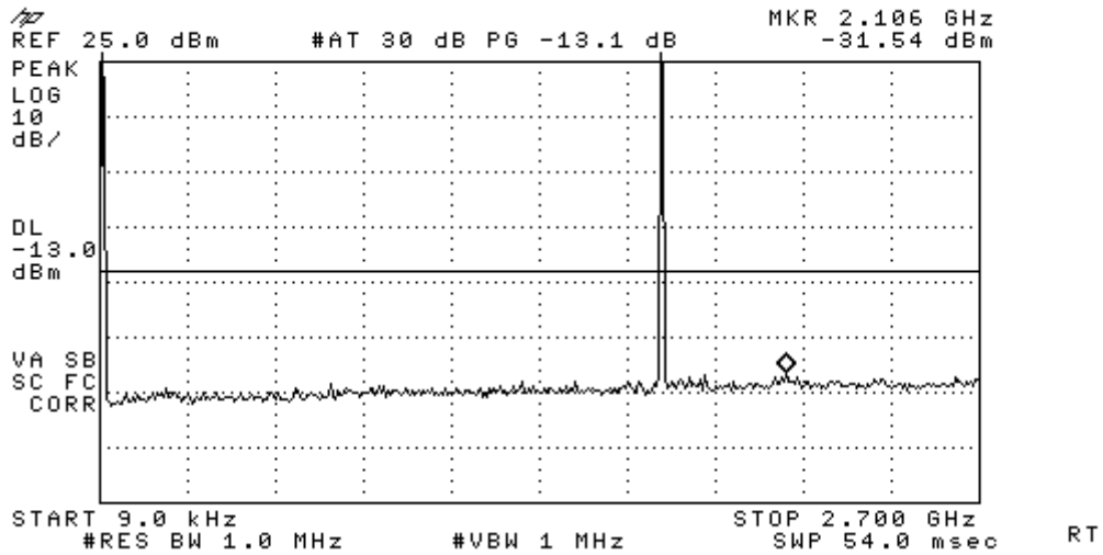
Figure 9-4a CDMA 1700 - Conducted Spurious Emission (CH 25)
