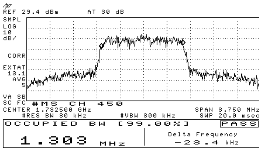
Figure 8-4 CDMA 1700 @ CH 450
