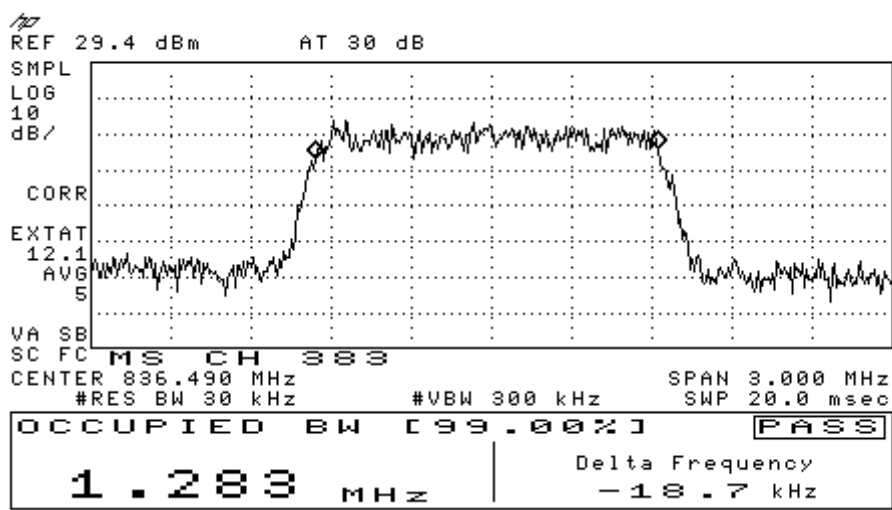
Figure 8-1 CDMA 800 @ CH 383
