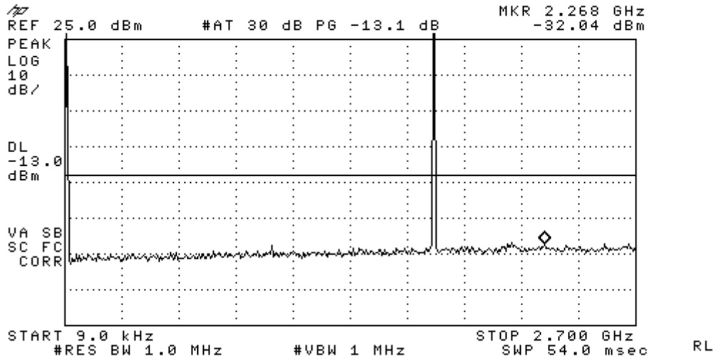
Figure 9-5a CDMA 1700 - Conducted Spurious Emission (CH 450)
