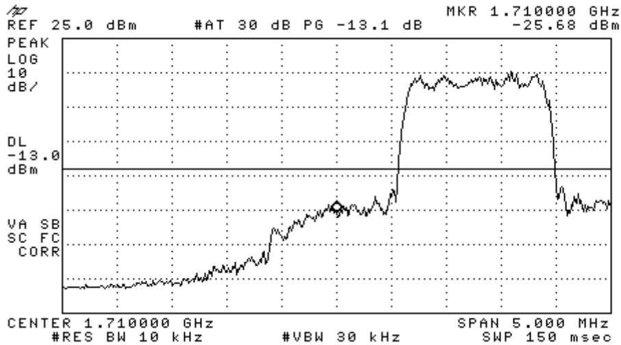
Figure 8-5 CDMA 1700 Lower Band Edge @ CH 25
