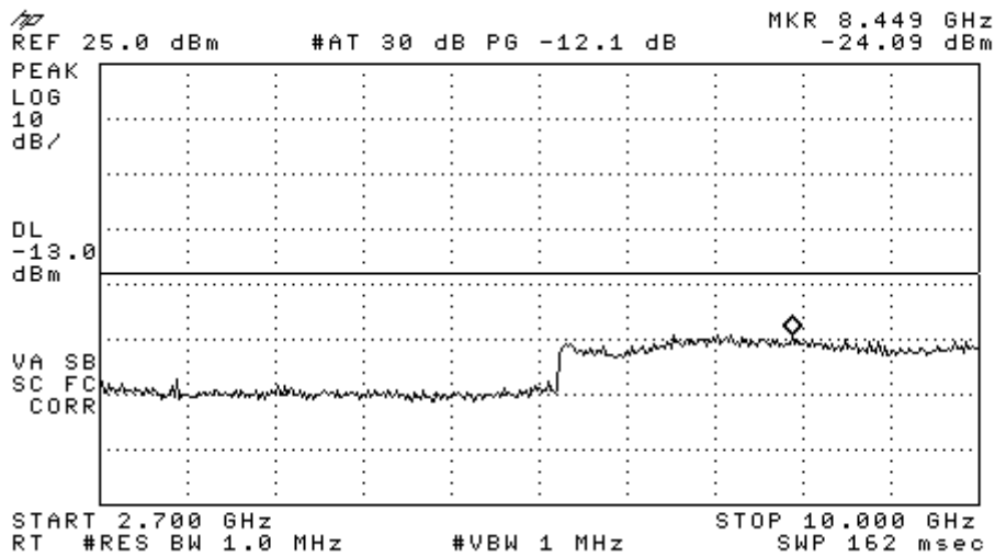
Figure 9-2b CDMA 800 – Conducted Spurious Emission (CH 383)
