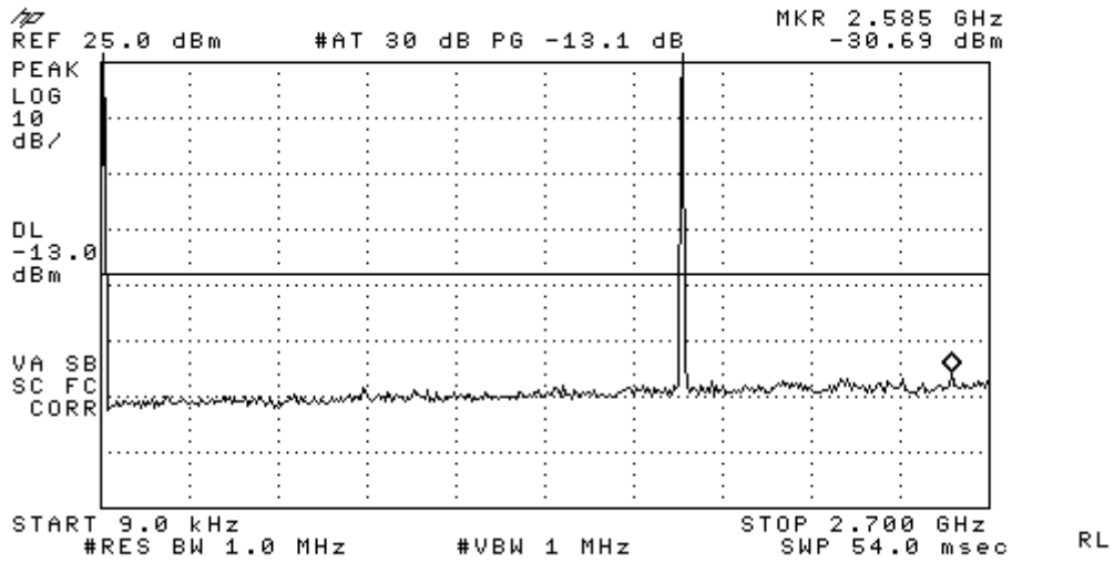
Figure 9-6a CDMA 1700 - Conducted Spurious Emission (CH 875)
