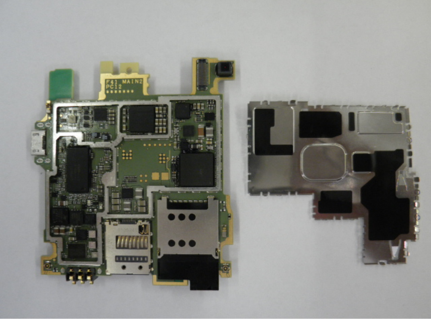
MAIN PCB L1 without Shield
