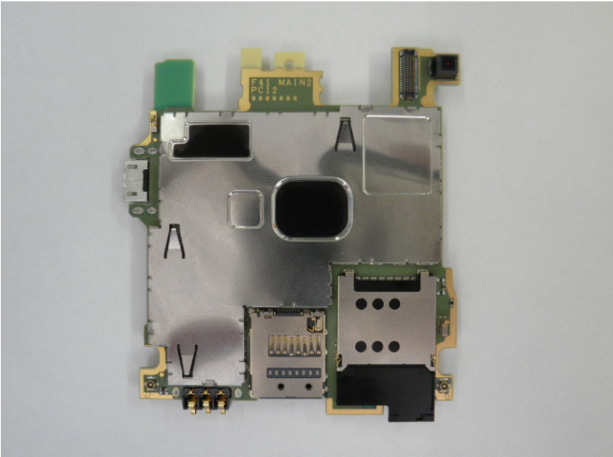
MAIN FPC L1 with shield
