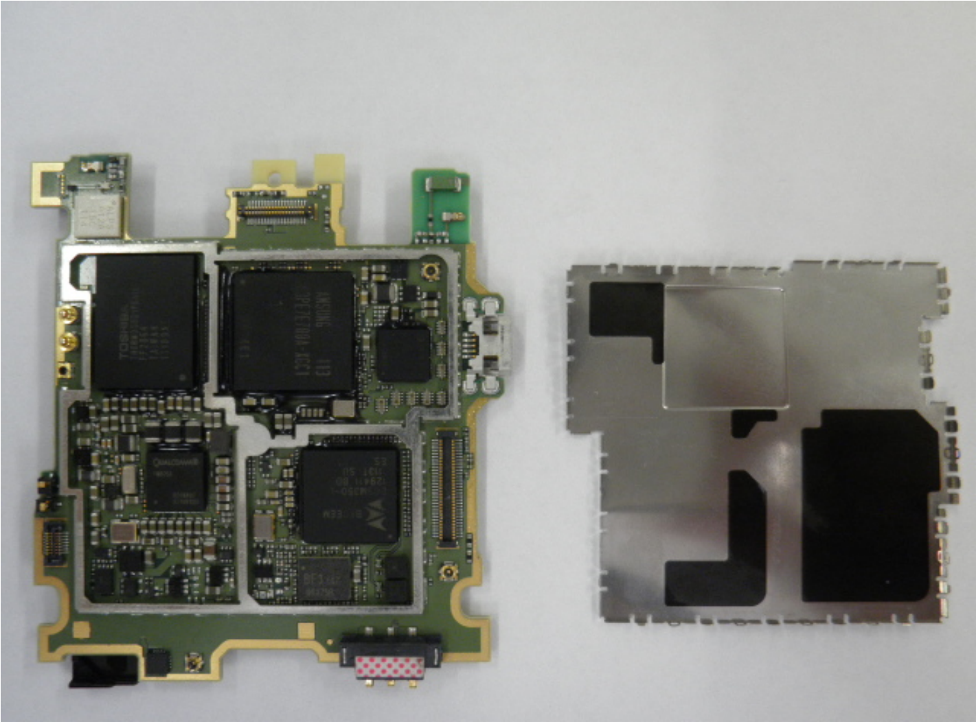
MAIN PCB L12 without Shield
