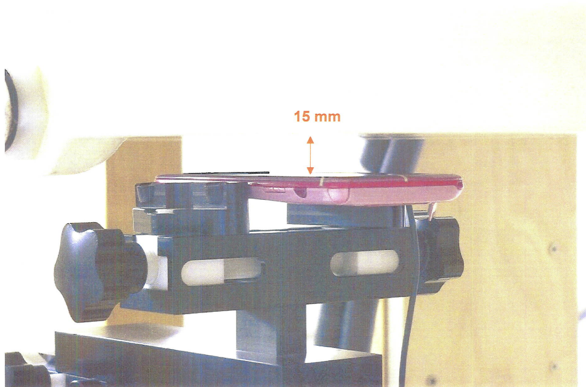
Fig. 32: Body worn configuration, position 1, display towards the phantom, headset attached, 15 mm distance
