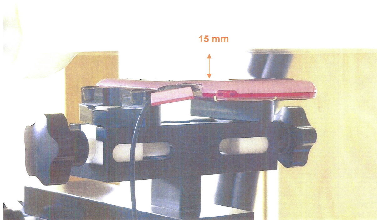
Fig. 33: Body worn configuration, position 2, display towards the ground, headset attached, 15 mm distance.
