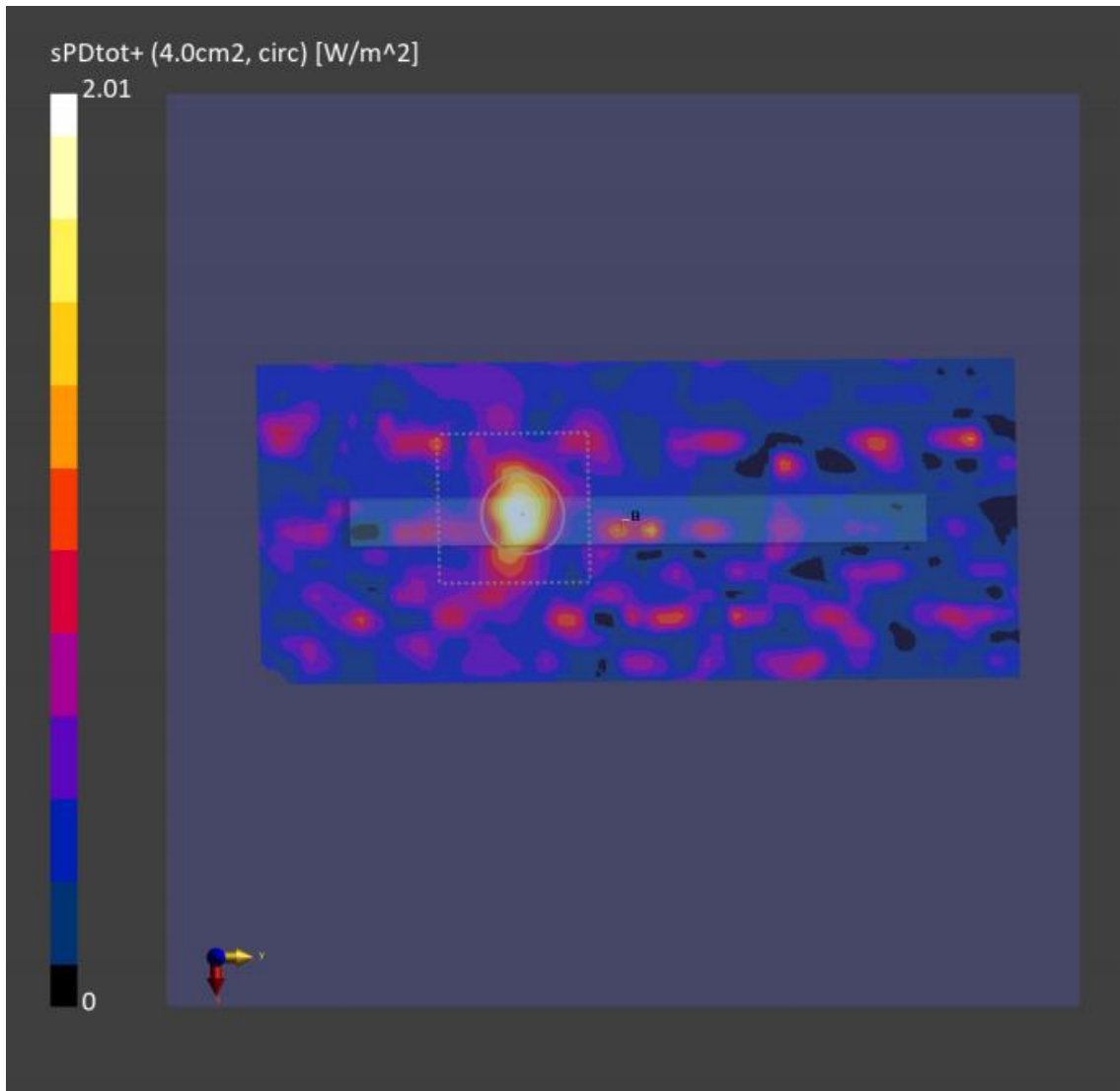
Figure 8-2: 4cm 2 -averaged power density distribution measured at input.power.limit of -0.9 dBm on the Left Side surface for n258 beam 31
