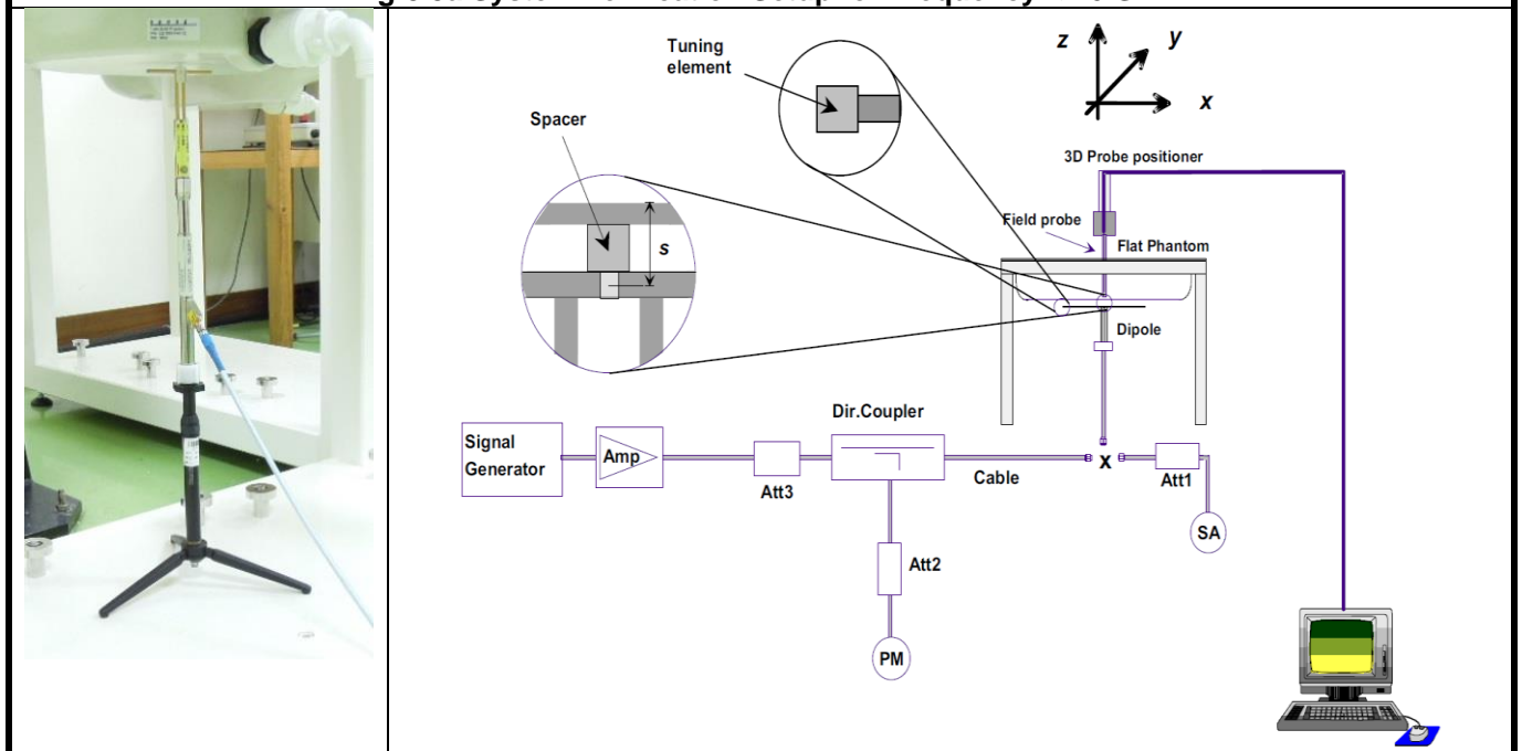
Fig-3.3b System Verification Setup for Frequency > 6 GHz
