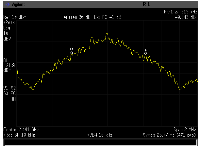
Figure 6-2a: 20dB Bandwidth Basic rate, Channel 39.
