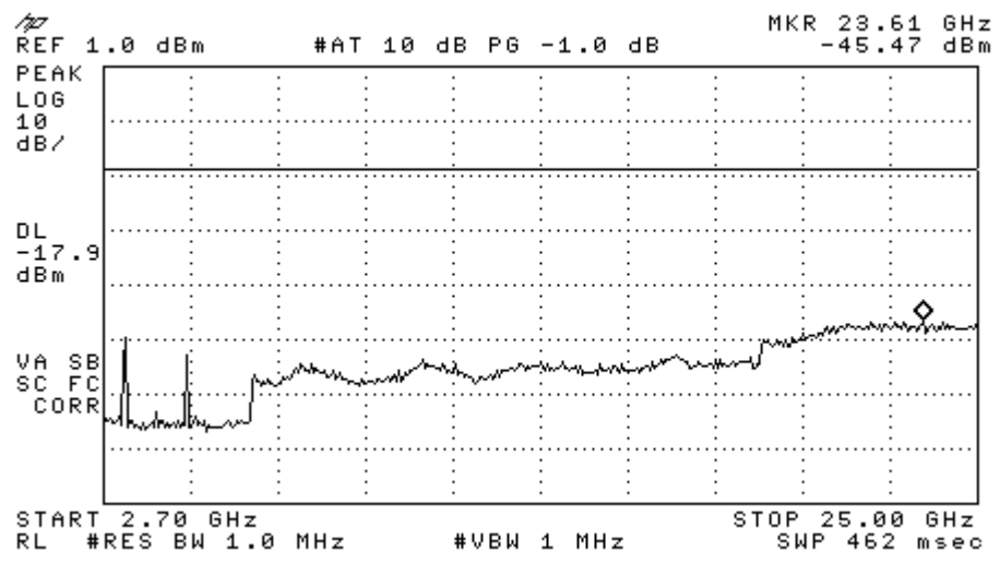
Figure 11-2b: Conducted Spurious Emissions (CH 39).
