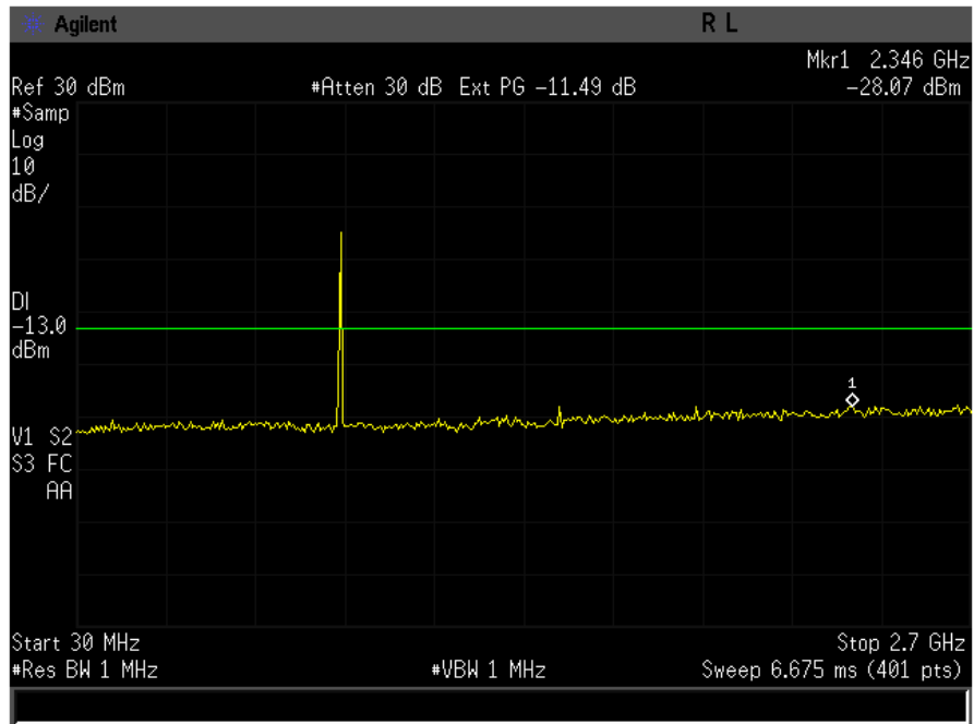
Figure 9-1a CDMA 800 BC-10 – Conducted Spurious Emission (CH 476)
