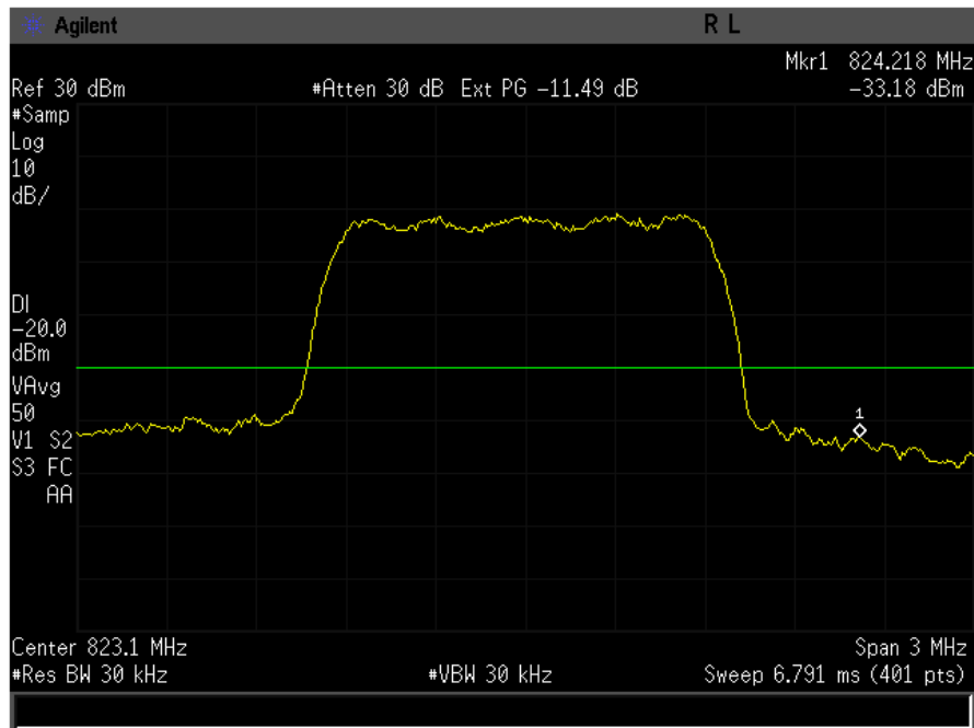
Figure 7-3 CDMA 800 Upper Band Edge @ CH 684
