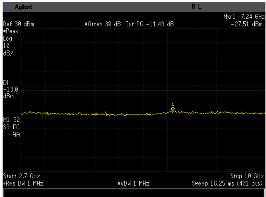
Figure 9-1b CDMA 800 BC-10 – Conducted Spurious Emission (CH 476)
