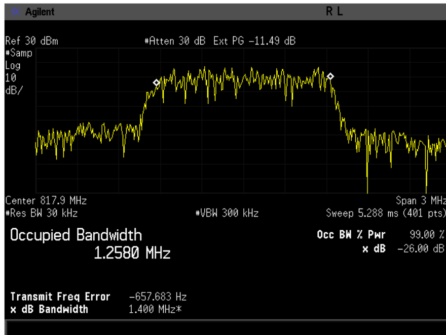
Figure 7-1 CDMA 800 BC-10 @ CH 476
