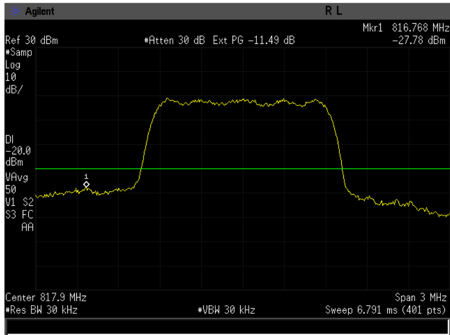
Figure 7-2 CDMA 800 BC-10 Lower Band Edge @ CH 476
