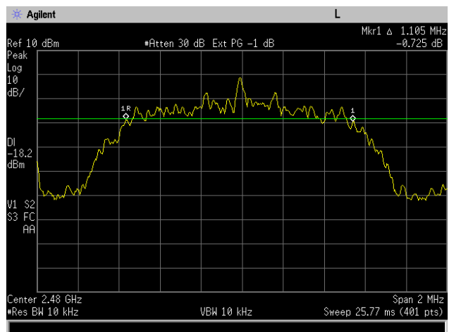
Figure 6-3c: 20dB Bandwidth EDR D8PSK, Channel 78.
