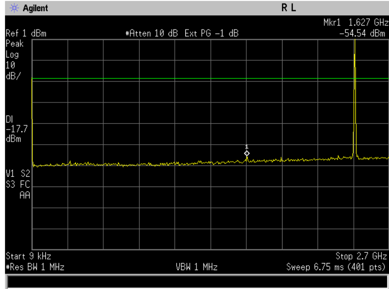
Figure 11-2a: Conducted Spurious Emissions (CH 39).
