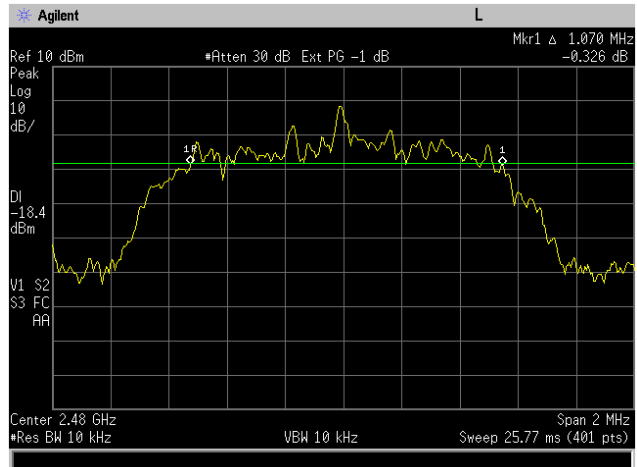
Figure 6-3b: 20dB Bandwidth EDR DQPSK, Channel 78.
