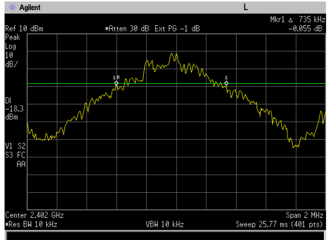
Figure 6-1a: 20dB Bandwidth Basic rate, Channel 0.
