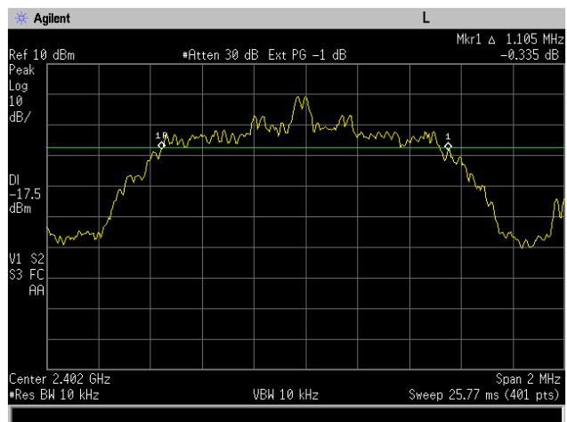
Figure 6-1c: 20dB Bandwidth EDR D8PSK, Channel 0.
