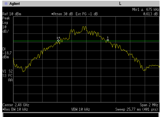
Figure 6-3a: 20dB Bandwidth Basic rate, Channel 78.
