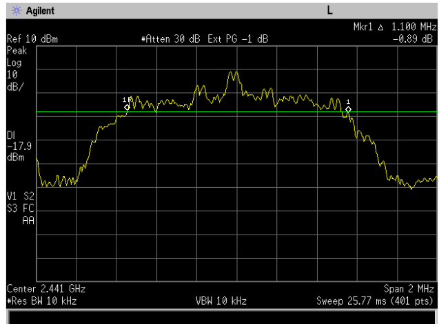
Figure 6-2b: 20dB Bandwidth EDR DQPSK, Channel 39.
