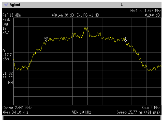
Figure 6-2c: 20dB Bandwidth EDR D8PSK, Channel 39.
