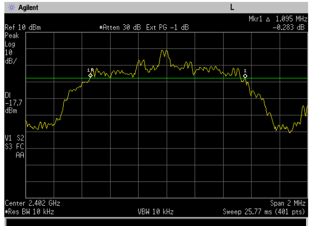
Figure 6-1b: 20dB Bandwidth EDR DQPSK, Channel 0.
