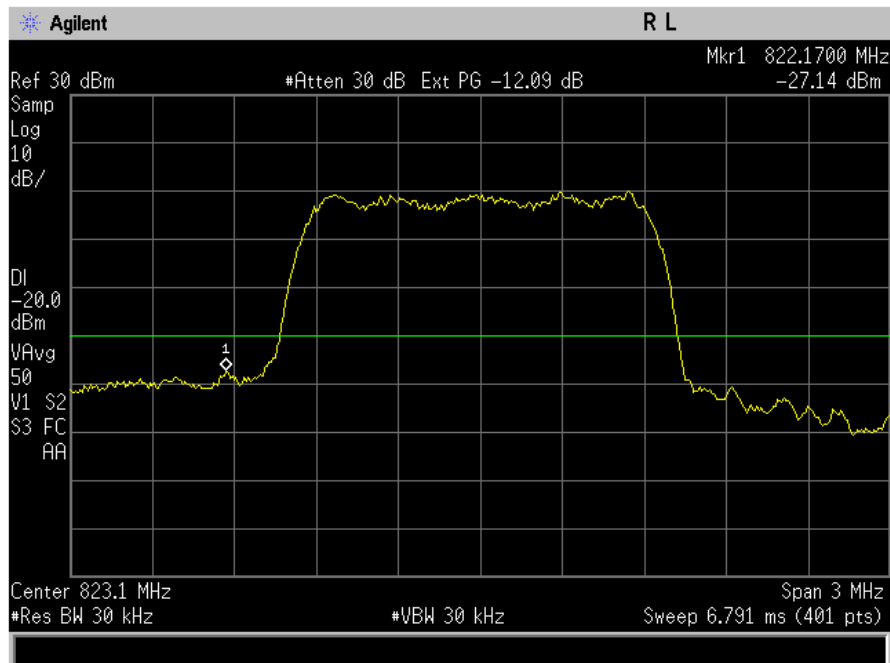
Figure 7-3 CDMA 800 BC-10 Upper Band Edge @ CH 684
