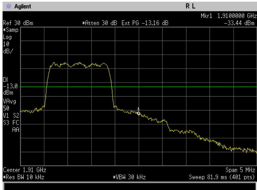
Figure 8-6 CDMA 1900 Upper Band Edge @ CH 1175
