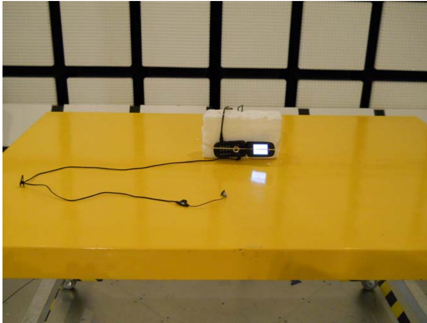
Z-AXIS WITH CHARGER PHOTO
