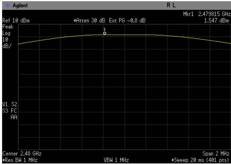
Figure 5-3: Peak Output Power, Channel 78.
