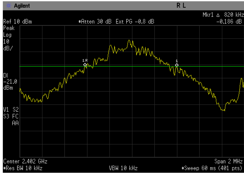
Figure 6-1a: 20dB Bandwidth Basic rate, Channel 0.
