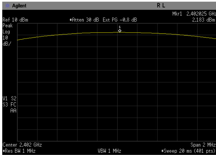
Figure 5-1b: Peak Output Power, EDR D8PSK Channel 0.
