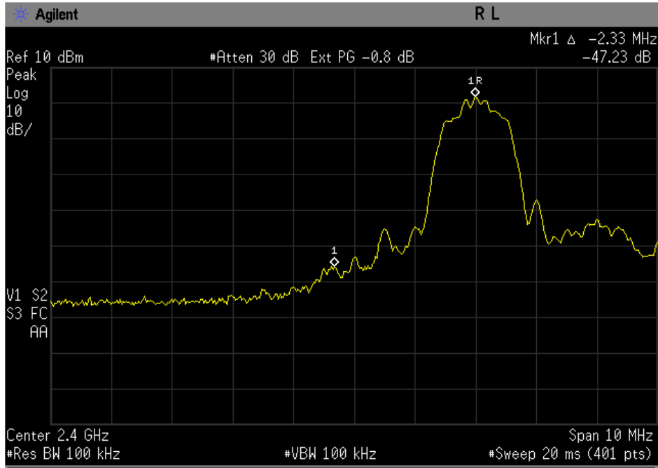
Figure 10-2a: EDR DQPSK Low band edge with hopping disabled.
