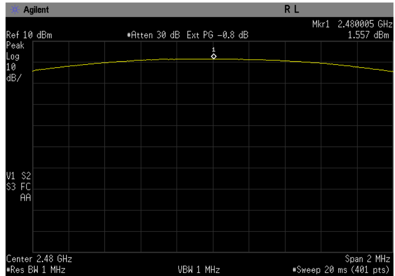
Figure 5-3b: Peak Output Power, EDR D8PSK Channel 78.
