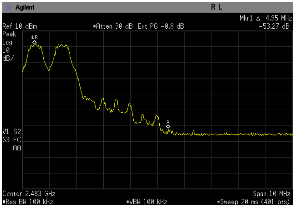
Figure 10-4b: Basic Rate High band edge with hopping enabled.
