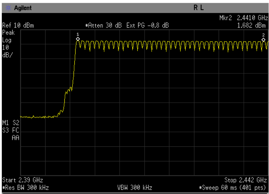
Figure 8a: Number of Hopping Frequencies (Channels 0-39).
