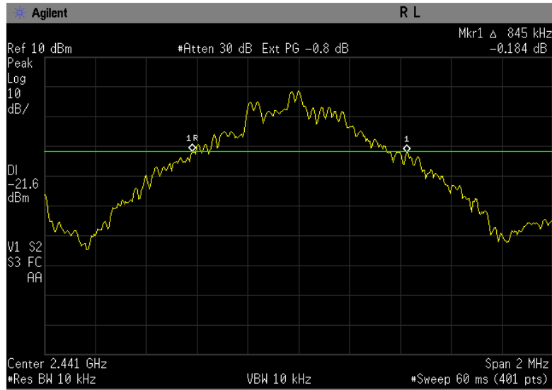
Figure 6-2a: 20dB Bandwidth Basic rate, Channel 39.
