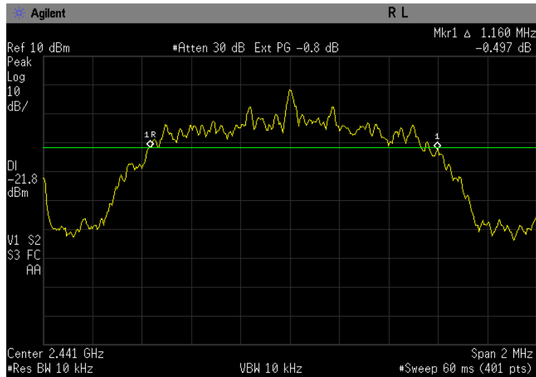
Figure 6-2c: 20dB Bandwidth EDR D8PSK, Channel 39.
