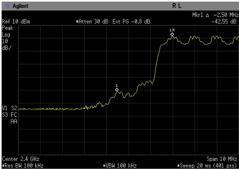
Figure 10-2b: EDR DQPSK Low band edge with hopping enabled.
