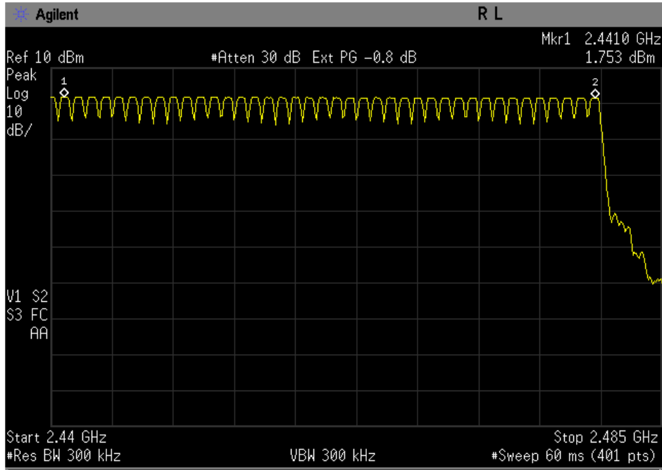
Figure 8b: Number of Hopping Frequencies (Channels 39-78).
