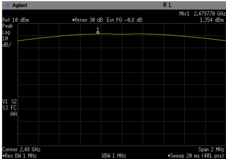
Figure 5-3a: Peak Output Power, EDR DQPSK Channel 78.
