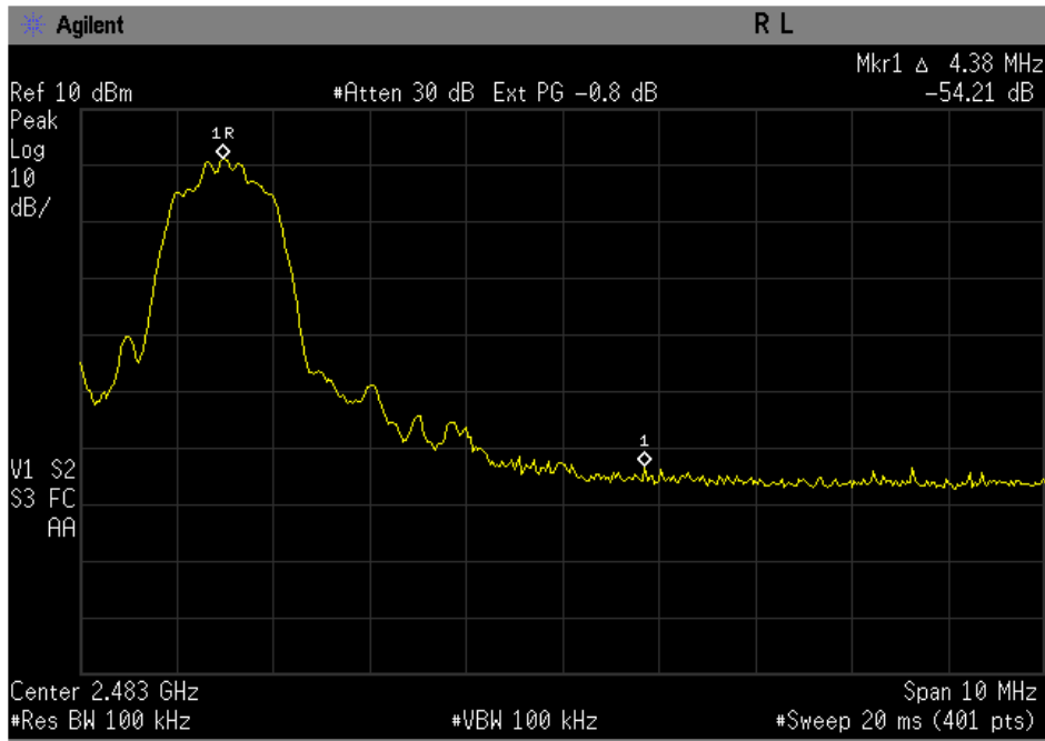
Figure 10-5a: EDR DQPSK High band edge with hopping disabled.
