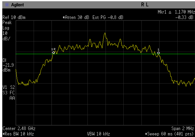
Figure 6-3c: 20dB Bandwidth EDR D8PSK, Channel 78.
