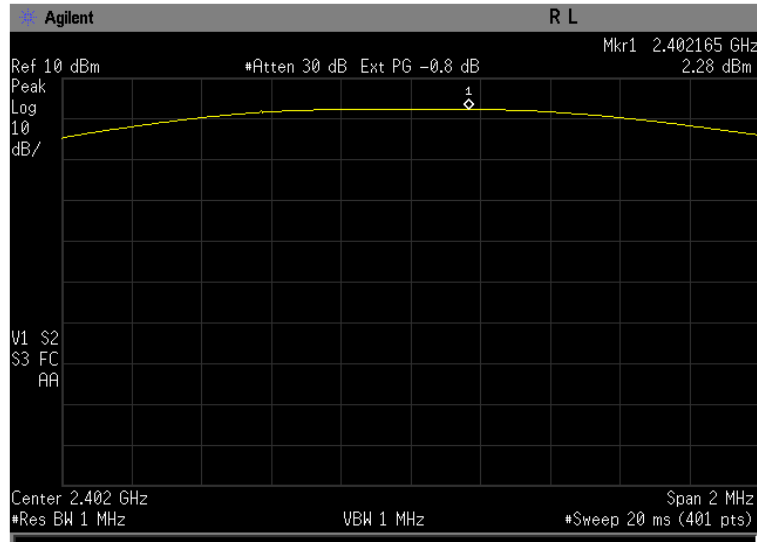
Figure 5-1: Peak Output Power, Basic Rate Channel 0.
