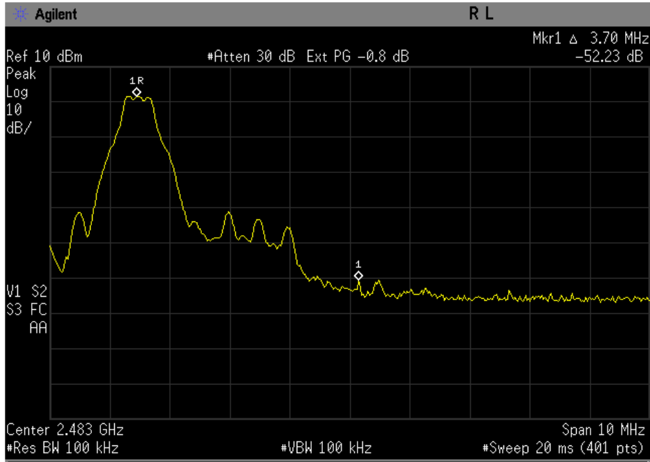
Figure 10-4a: Basic Rate High band edge with hopping disabled.
