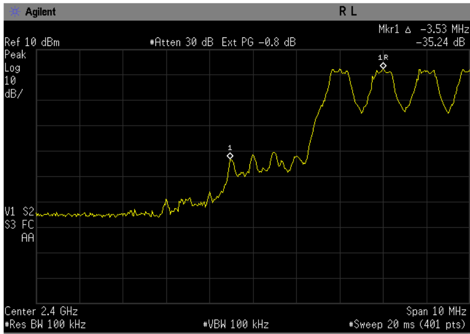
Figure 10-1b: Basic Rate Low band edge with hopping enabled.
