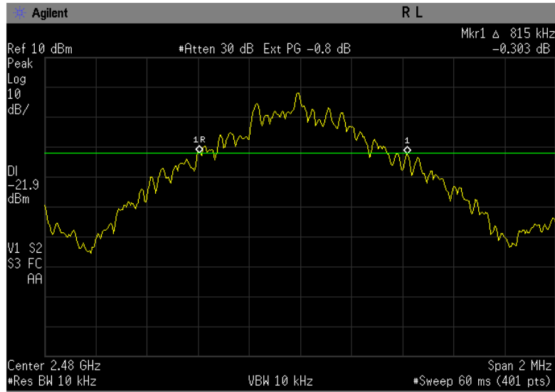
Figure 6-3a: 20dB Bandwidth Basic rate, Channel 78.
