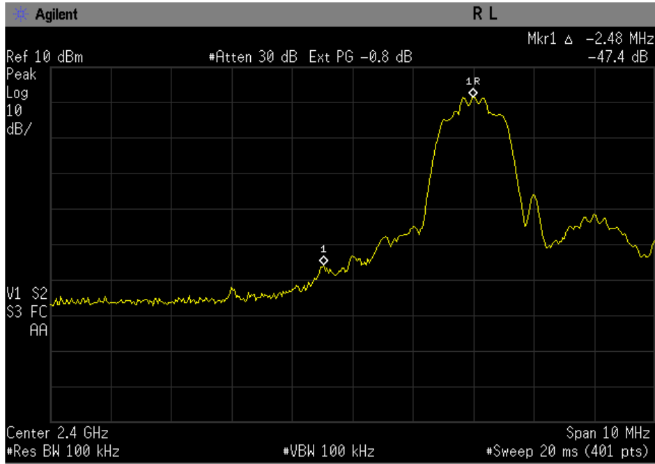
Figure 10-3a: EDR D8PSK Low band edge with hopping disabled.
