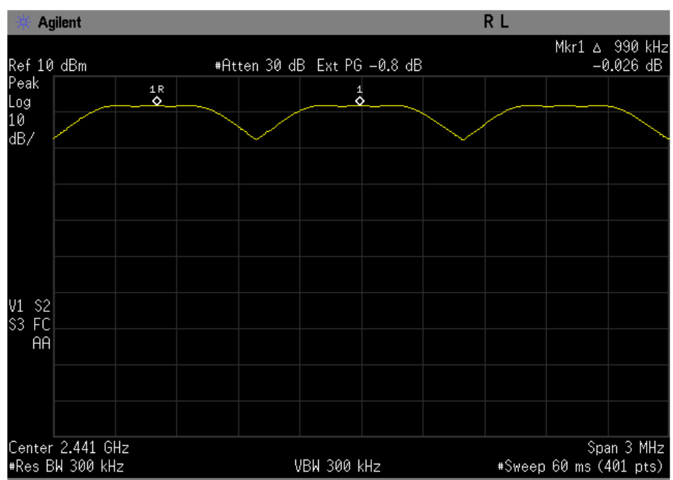
Figure 7: Carrier Frequency Separation between channels 38, 39 (mid-channel) & 40.
