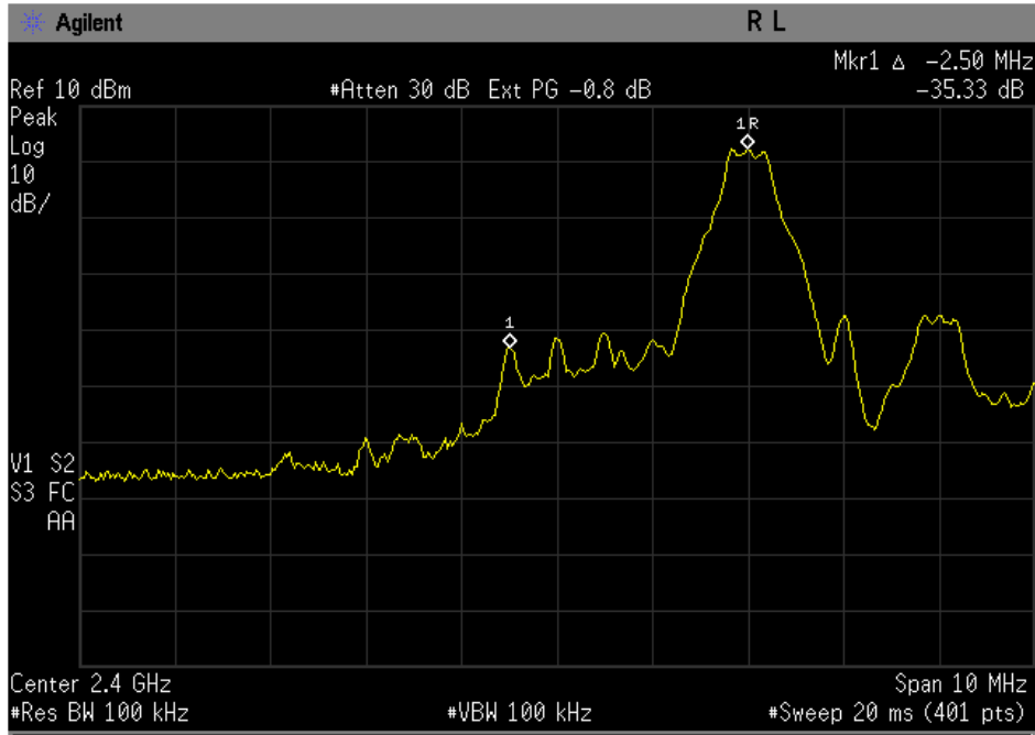
Figure 10-1a: Basic Rate Low band edge with hopping disabled.
