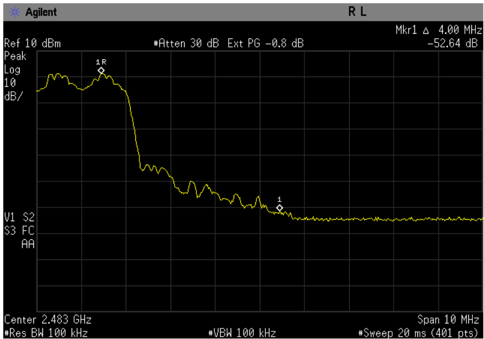
Figure 10-5b: EDR DQPSK High band edge with hopping enabled.
