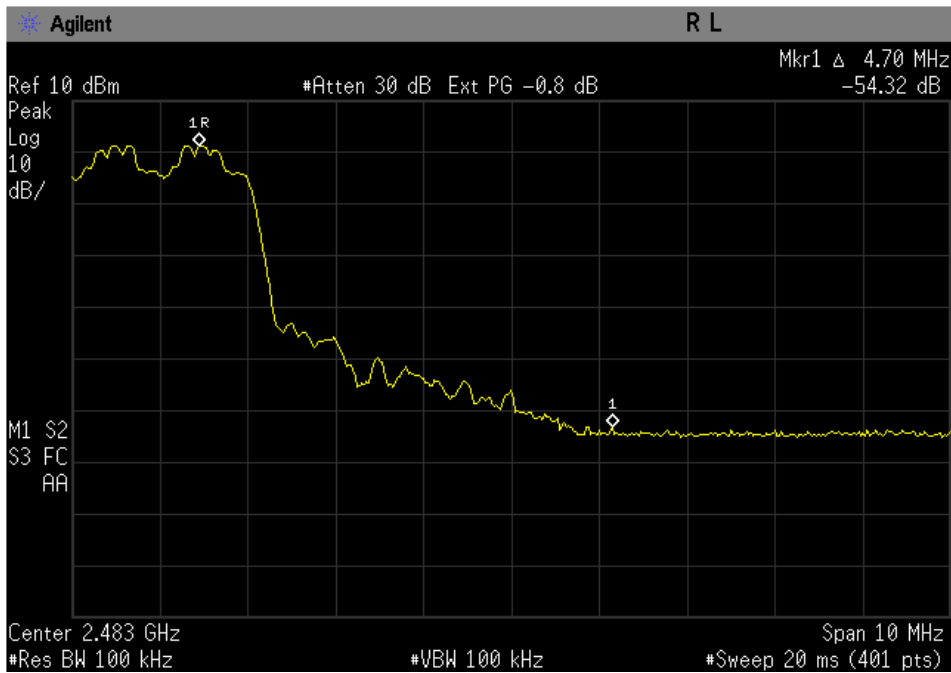
Figure 10-6b: EDR D8PSK High band edge with hopping enabled.
