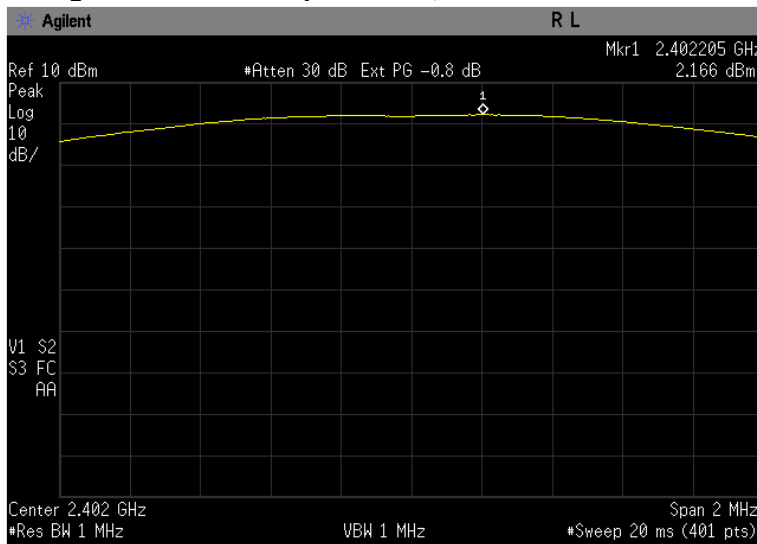
Figure 5-1a: Peak Output Power, EDR DQPSK Channel 0.
