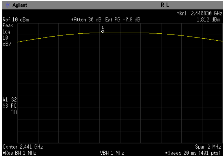
Figure 5-2: Peak Output Power, Channel 39.
