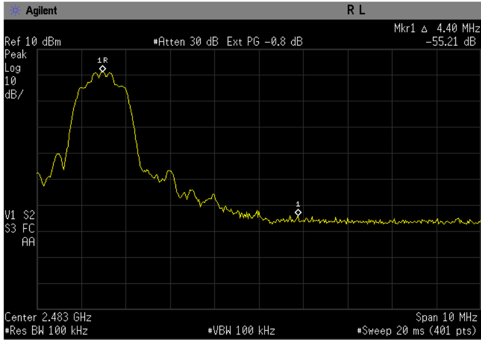
Figure 10-6a: EDR D8PSK High band edge with hopping disabled.
