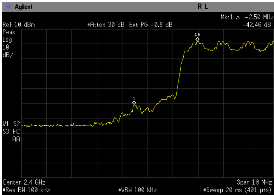
Figure 10-3b: EDR D8PSK Low band edge with hopping enabled.
