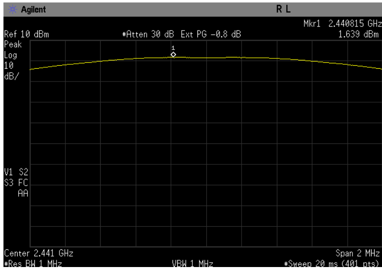
Figure 5-2a: Peak Output Power, EDR DQPSK Channel 39.
