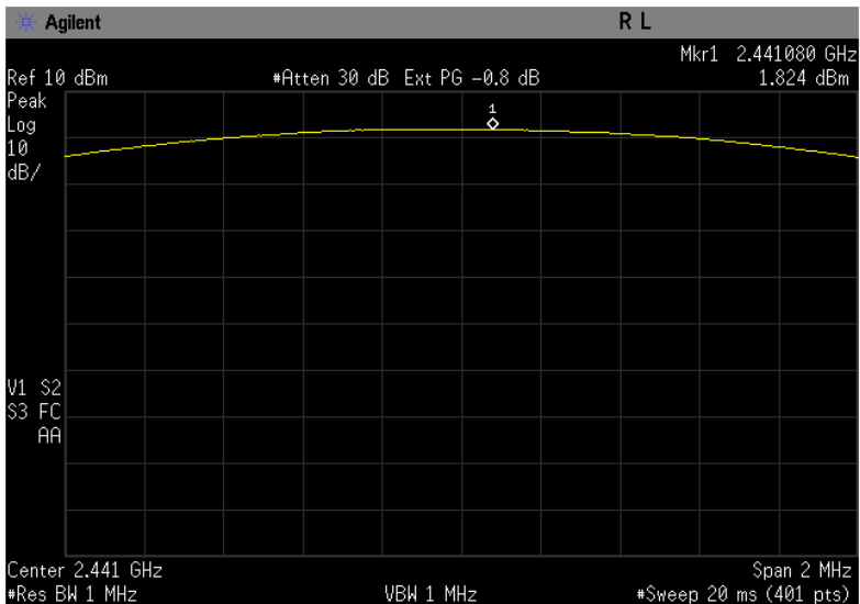
Figure 5-2b: Peak Output Power, EDR D8PSK Channel 39.
