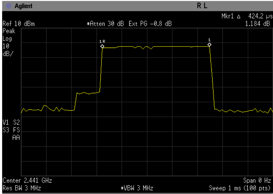
Figure 9: Duration of one transmission (Channel 39).
