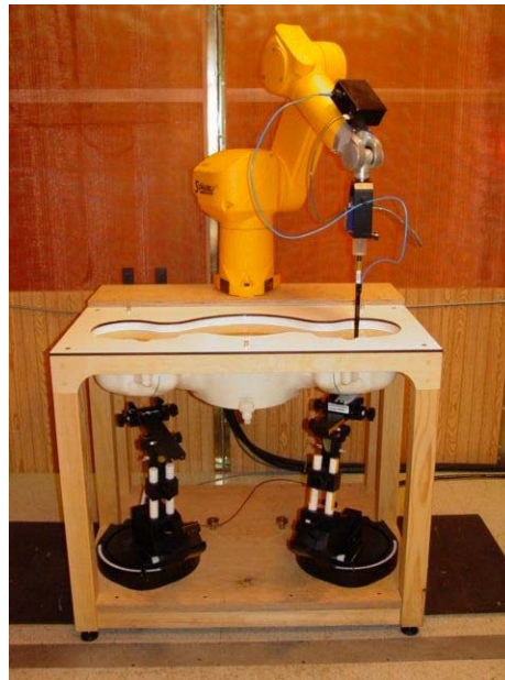
Figure 5.1 DASY 4 System
