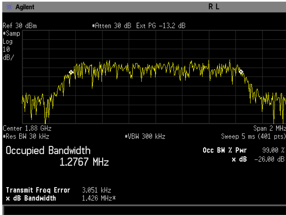
Figure 8-4 CDMA 1900 @ CH 600
