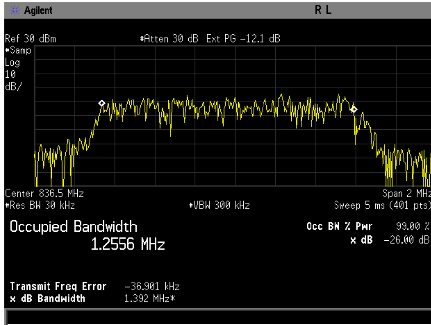
Figure 8-1 CDMA 800 @ CH 383
