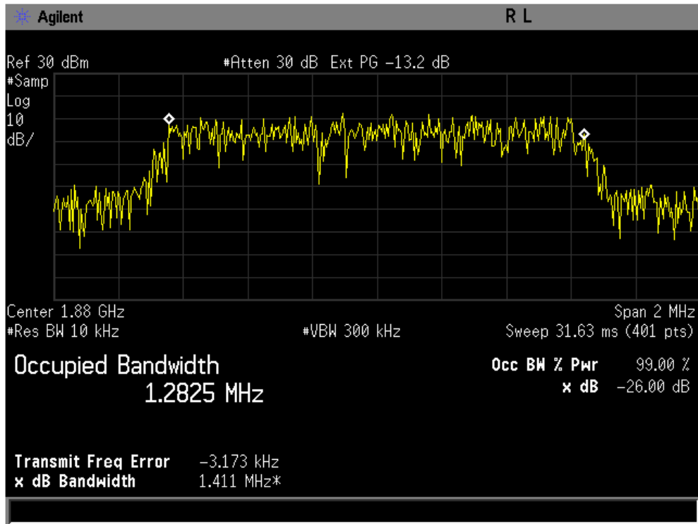
Figure 8-4 CDMA 1900 @ CH 600
