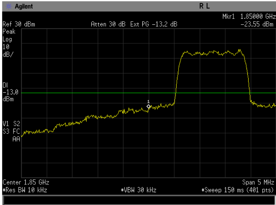
Figure 8-5 CDMA 1900 Lower Band Edge @ CH 25
