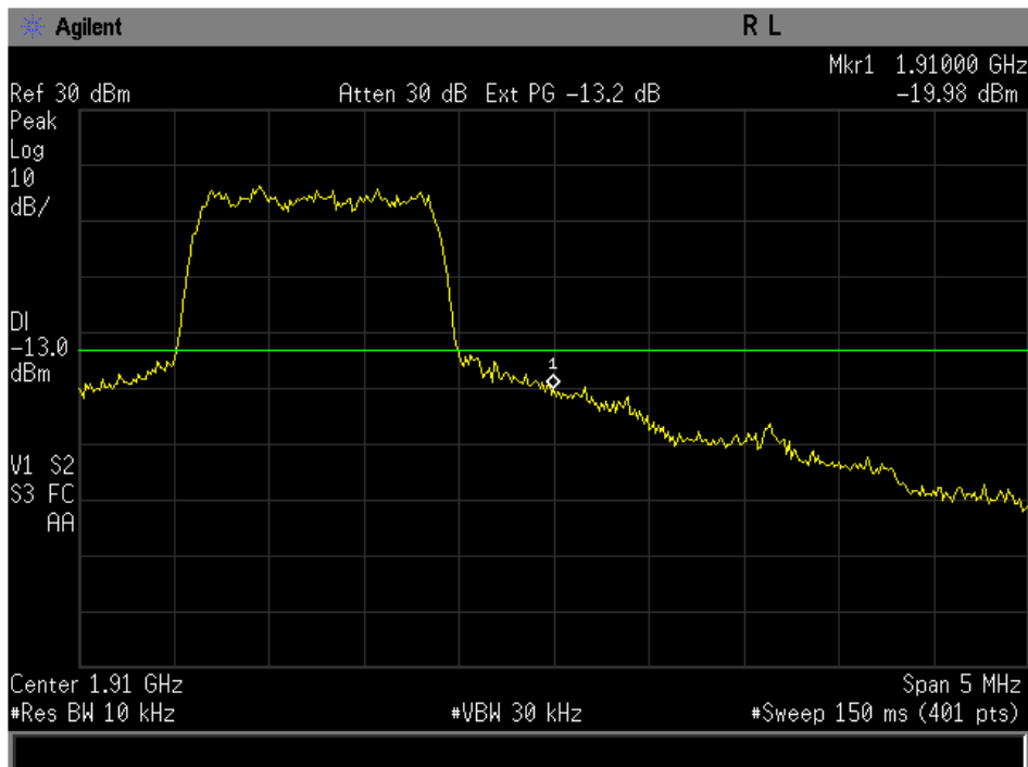
Figure 8-6 CDMA 1900 Upper Band Edge @ CH 1175
