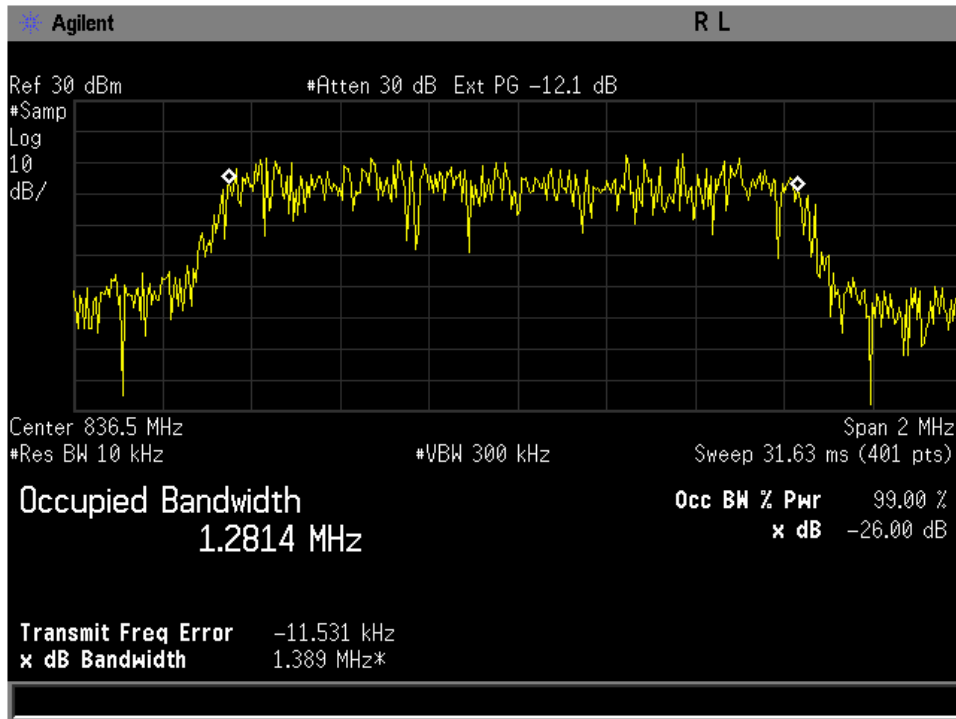
Figure 8-1 CDMA 800 @ CH 383
