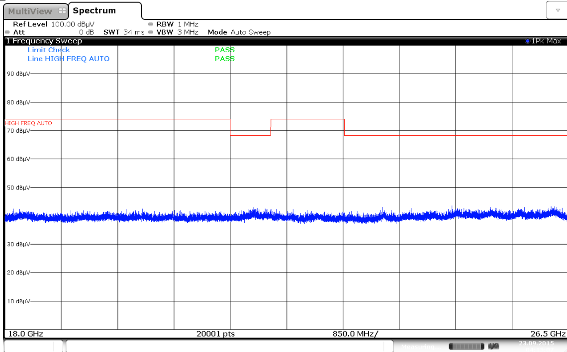
Plot 6-41. Radiated Spurious Plot above 18GHz (Pol. H)
