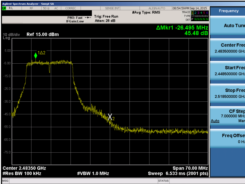
Plot 6-24. Band Edge Plot (802.11g – Ch. 11)
