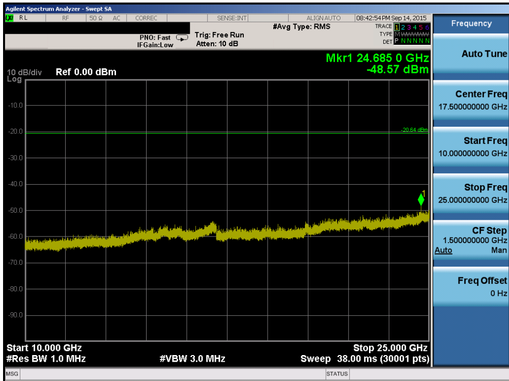
Plot 6-30. Conducted Spurious Plot (802.11b – Ch. 1)
