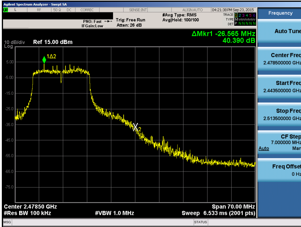
Plot 6-23. Band Edge Plot (802.11g – Ch. 10)
