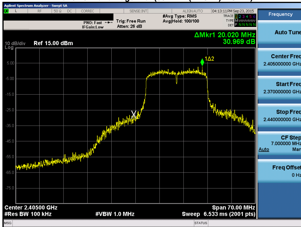
Plot 6-26. Band Edge Plot (802.11n (2.4GHz) – Ch. 2)
