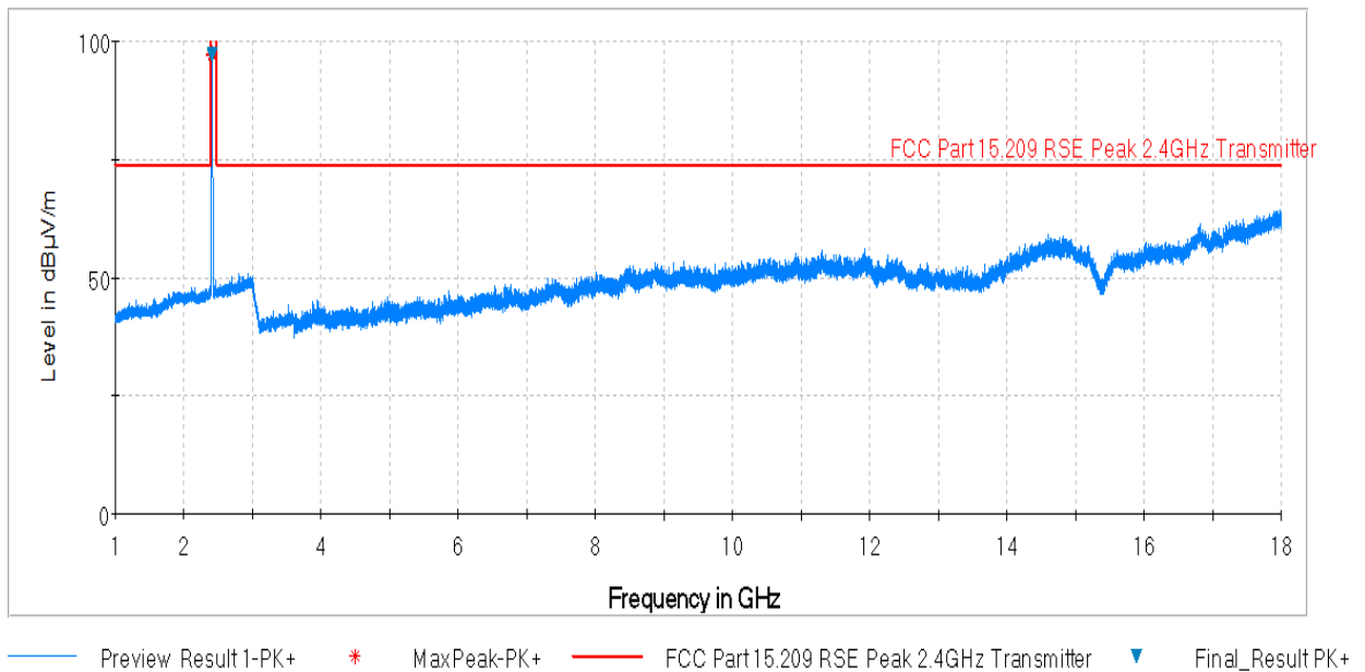
Plot 6-36. Radiated Spurious Plot above 1GHz (802.11b – Ch. 1, Ant. Pol. V)
