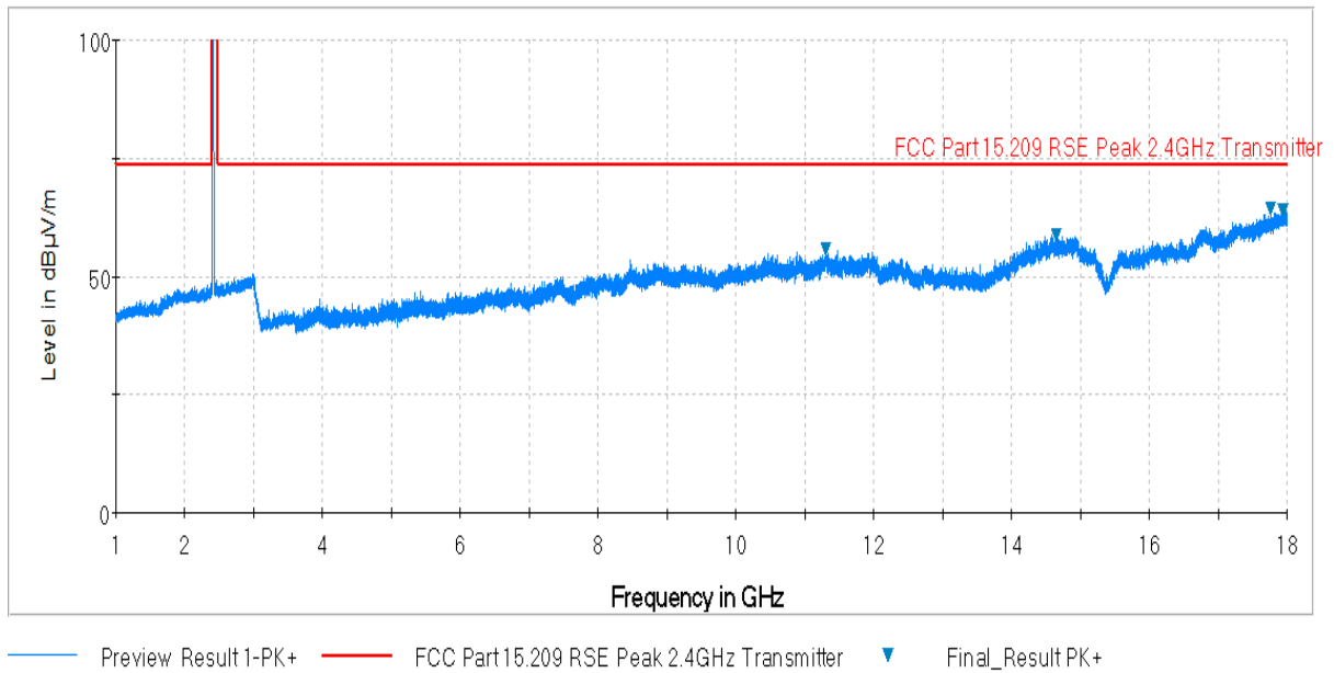
Plot 6-35. Radiated Spurious Plot above 1GHz (802.11b – Ch. 1, Ant. Pol. H)
