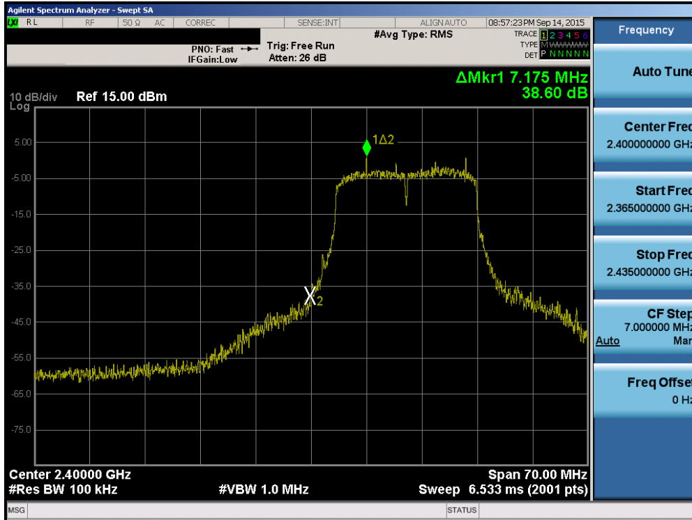
Plot 6-25. Band Edge Plot (802.11n (2.4GHz) – Ch. 1)
