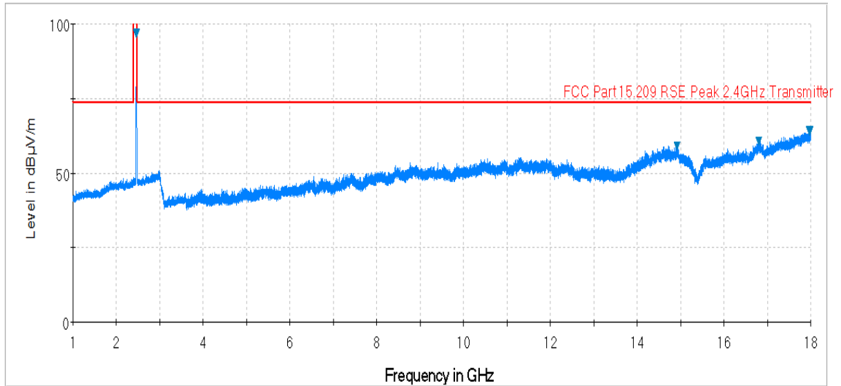
Plot 6-39. Radiated Spurious Plot above 1GHz (802.11b – Ch. 11, Ant. Pol. H)
