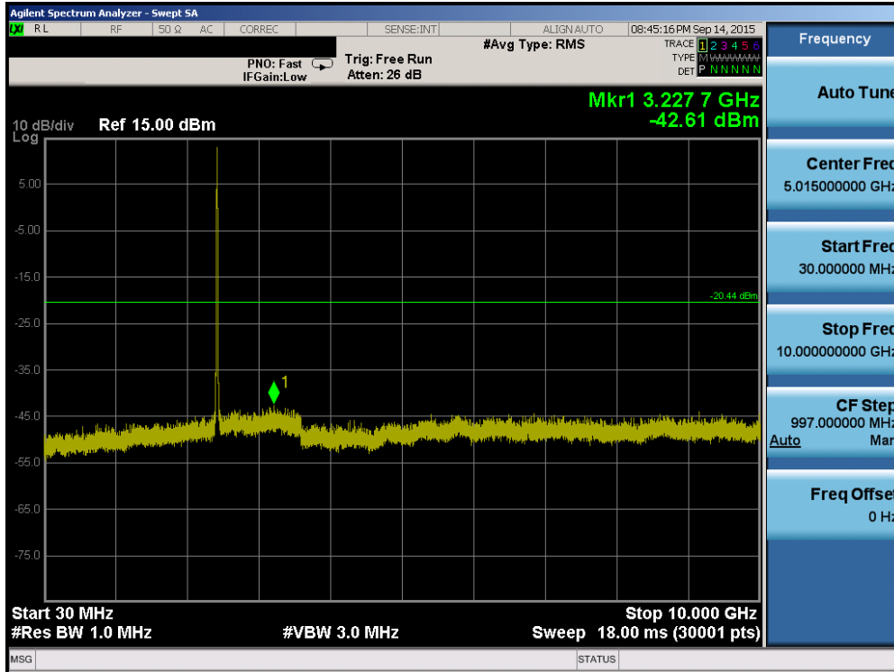
Plot 6-31. Conducted Spurious Plot (802.11b – Ch. 6)
