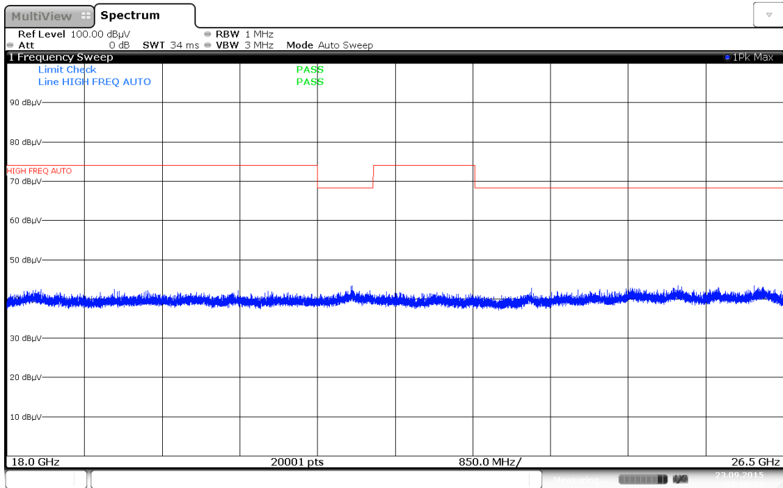
Plot 6-42. Radiated Spurious Plot above 18GHz (Pol. V)
