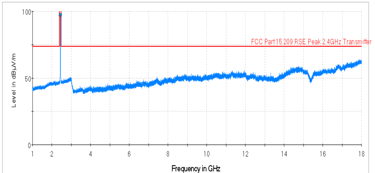
Plot 6-38. Radiated Spurious Plot above 1GHz (802.11b – Ch. 6, Ant. Pol. V)
