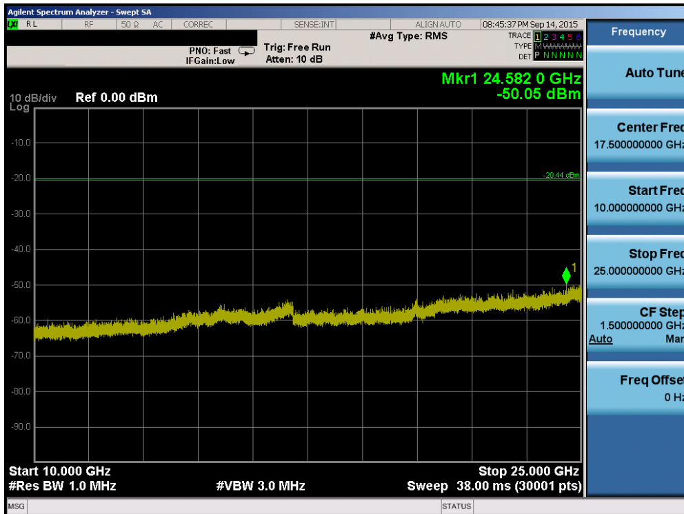
Plot 6-32. Conducted Spurious Plot (802.11b – Ch. 6)
