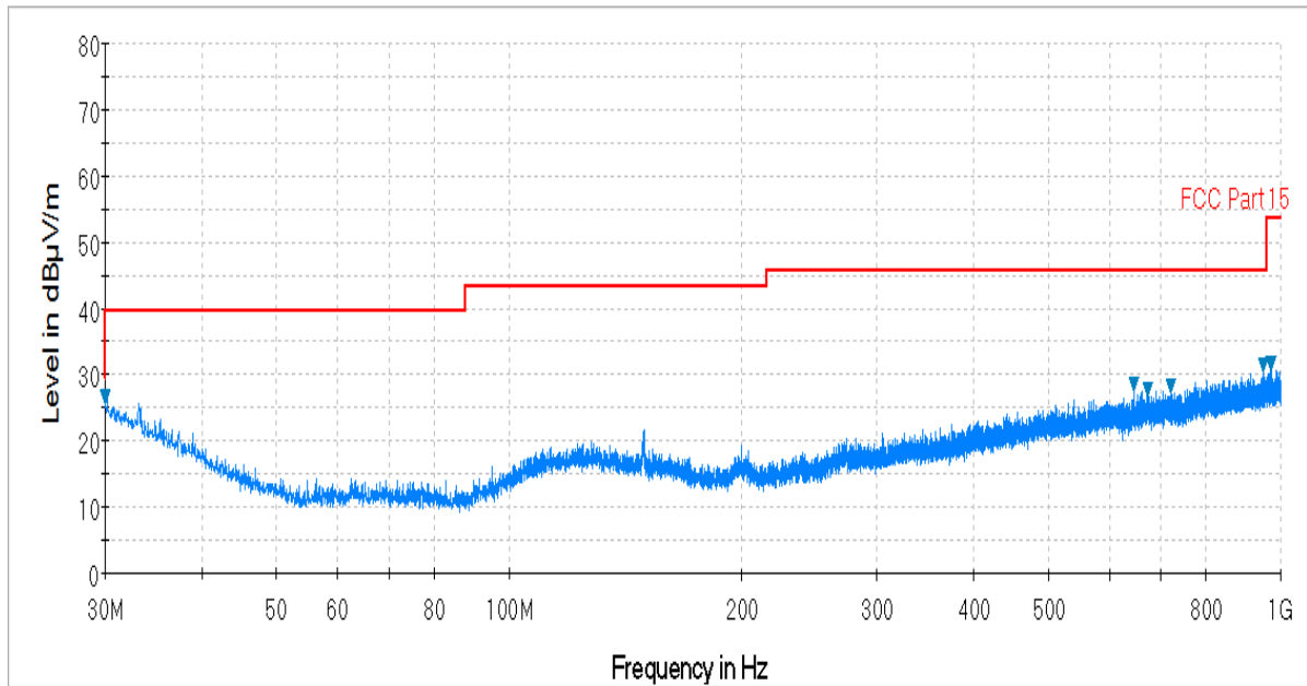
Plot 6-52. Radiated Spurious Plot below 1GHz (Pol. V)
