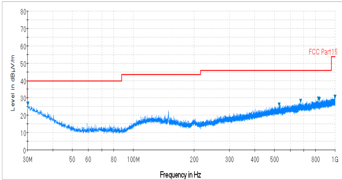
Plot 6-51. Radiated Spurious Plot below 1GHz (Pol. H)
