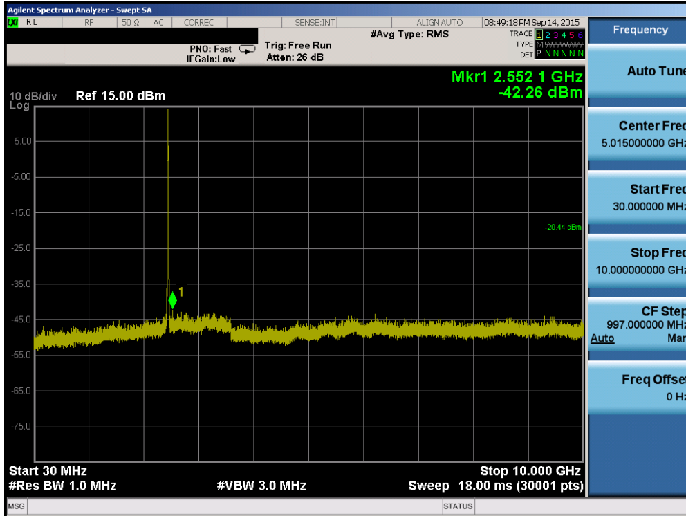
Plot 6-33. Conducted Spurious Plot (802.11b – Ch. 11)
