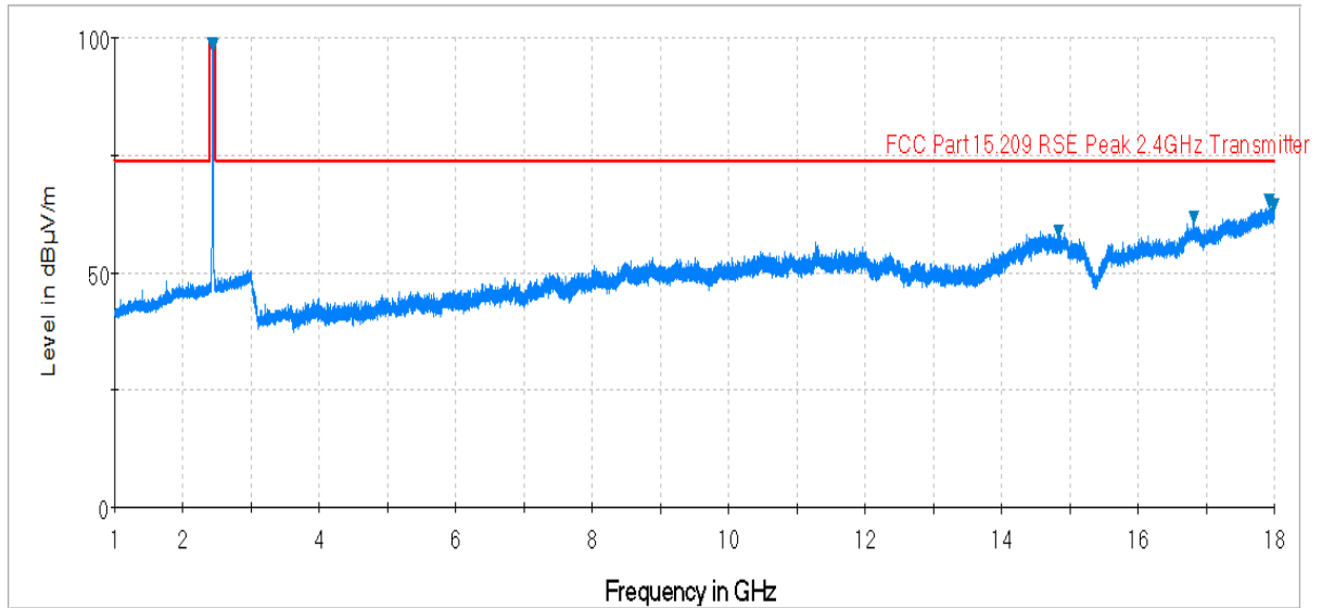
Plot 6-37. Radiated Spurious Plot above 1GHz (802.11b – Ch. 6, Ant. Pol. H)
