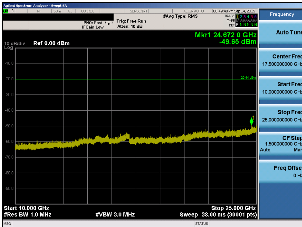
Plot 6-34. Conducted Spurious Plot (802.11b – Ch. 11)
