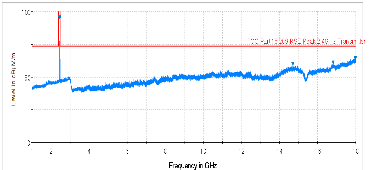
Plot 6-40. Radiated Spurious Plot above 1GHz (802.11b – Ch. 11, Ant. Pol. V)
