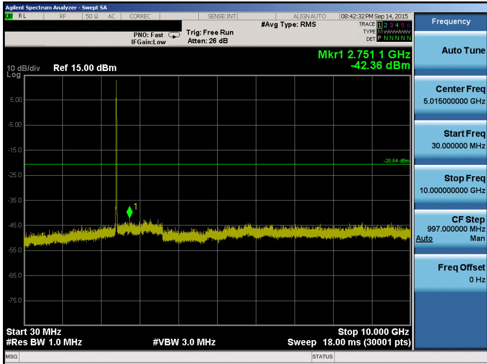
Plot 6-29. Conducted Spurious Plot (802.11b – Ch. 1)
