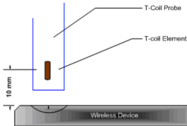
Figure 5-10 Measurement Distance
