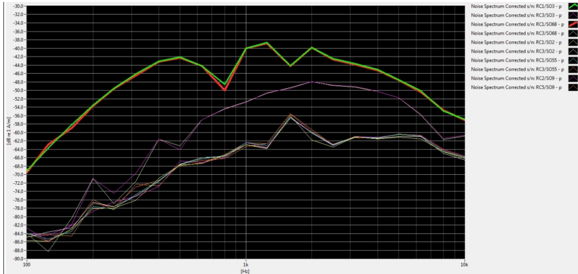
Figure 6-1 CDMA Audio Band Magnetic Noise
