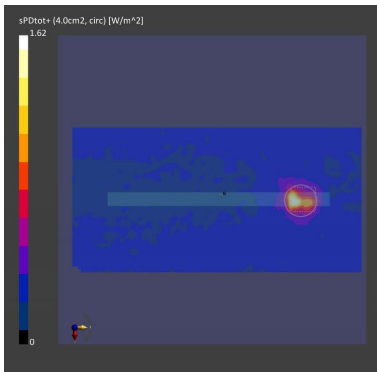
Figure 8-3: 4cm2-averaged power density distribution measured at input.power.limit of 2.34 dBm on the Right Side surface for n260 beam 1
