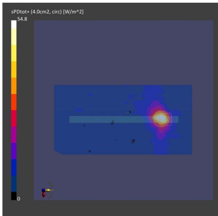
Figure 8-2: 4cm2-averaged power density distribution measured at input.power.limit of 3.81 dBm on the Right Side surface for n261 beam 22
