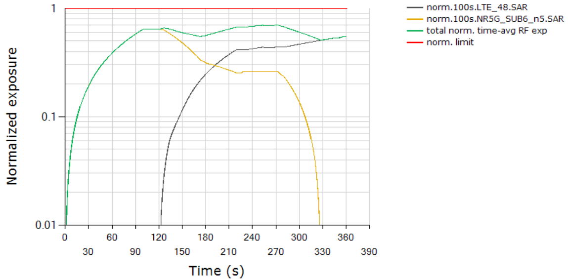
Total Normalized Time-averaged RF Exposure Tech: LTE, Band 48 / Tech: NR5G SUB6, Band n5
