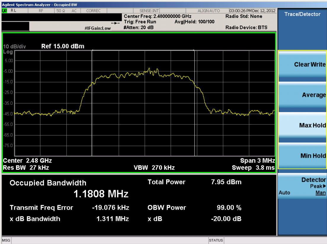
Plot 6-6. 20dB Bandwidth Plot (Bluetooth, 2Mbps – Ch. 78)
