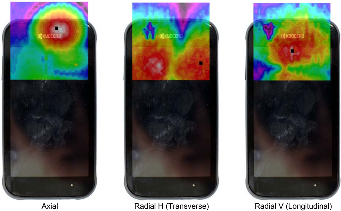
Figure 13-3 T-Coil Scan Overlay Magnetic Field Distributions
