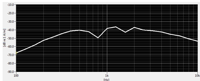
Figure 6-2 Worst-case ABM2 Plot for WD
