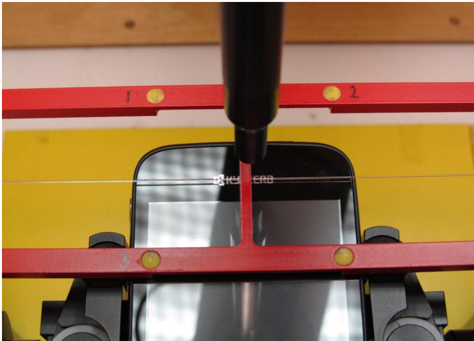
Figure 1b – HAC RF Emission Test Setup
