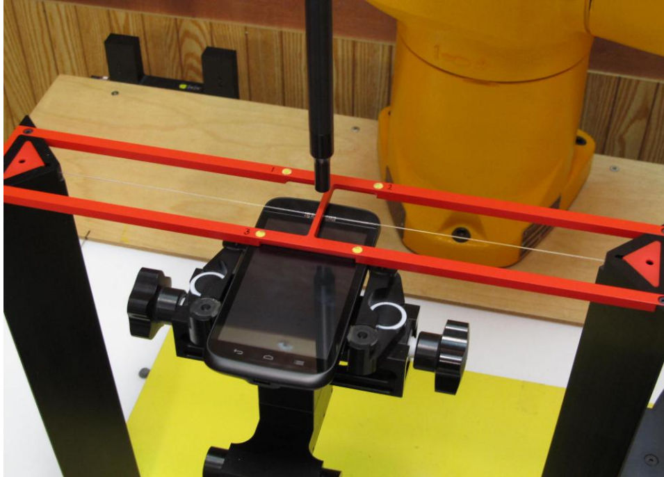
Figure 1a – HAC RF Emission Test Setup
