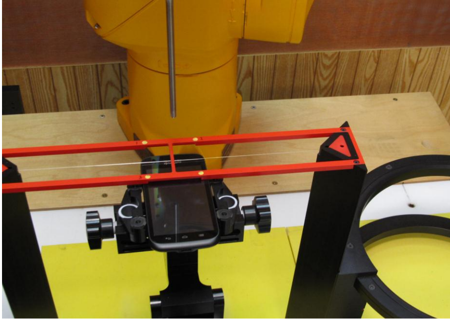
Figure 1a – HAC Tcoil Emission Test Setup
