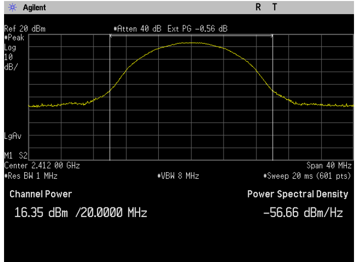
Figure 7-1: Output Power 802.11b, 11Mbps, Ch 1
