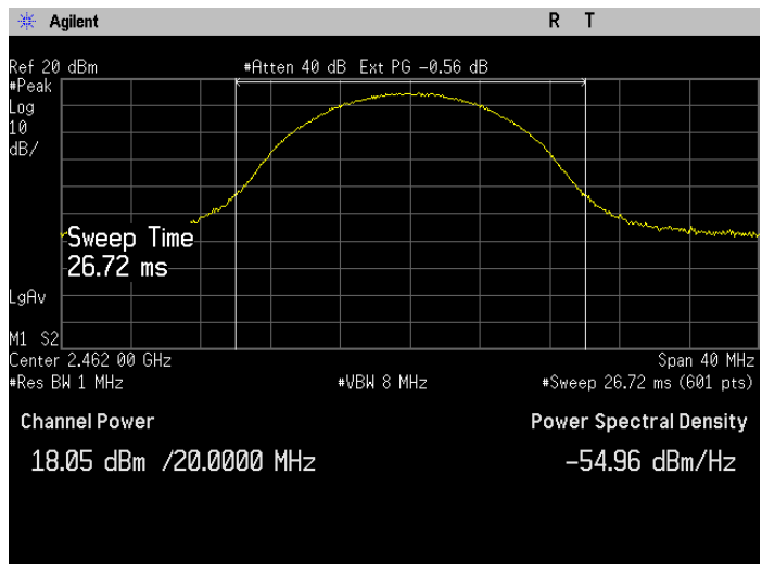
Figure 7-3: Output Power 802.11b, 11Mbps, Ch 11
