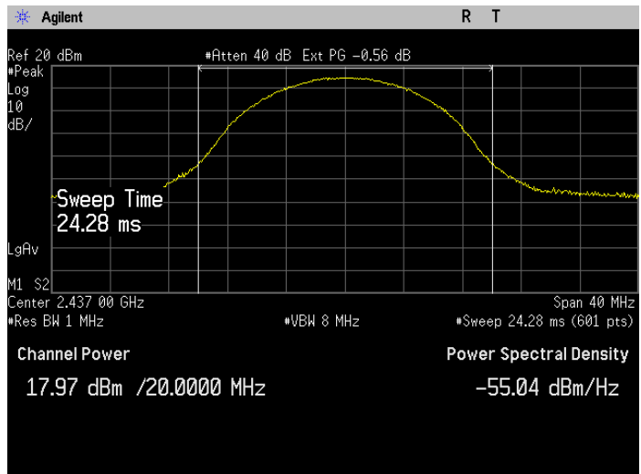
Figure 7-2: Output Power 802.11b, 11Mbps, Ch 6
