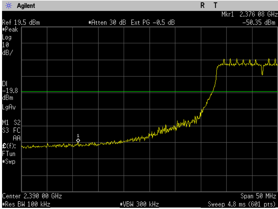
Figure 9-3a: Low band edge, 802.11n, ch1.
