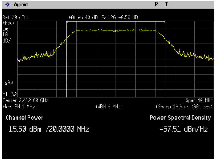
Figure 7-7: Output Power 802.11n, MSC0, Ch 1
