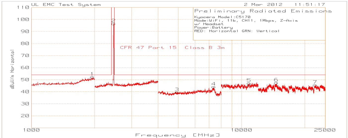
Figure 13 Radiated Emissions Graph Z-Axis
