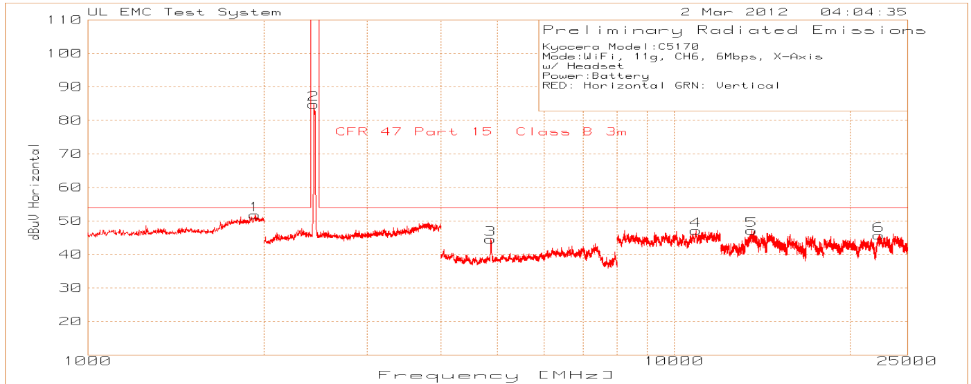
Figure 10 Radiated Emissions Graph X-Axis
