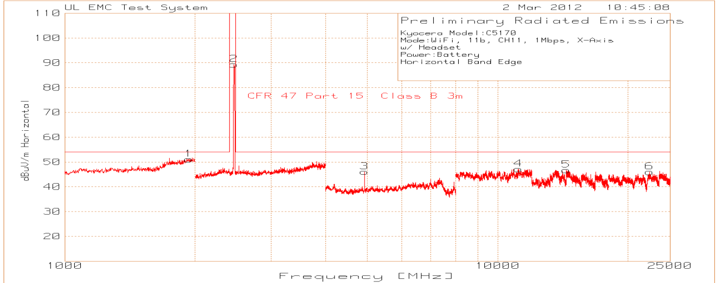
Figure 14 Radiated Emissions Graph X-Axis
