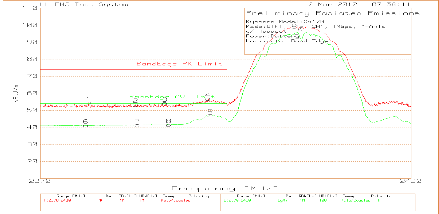
Figure 17 Band-edge Graph Y-Axis, Horizontal
