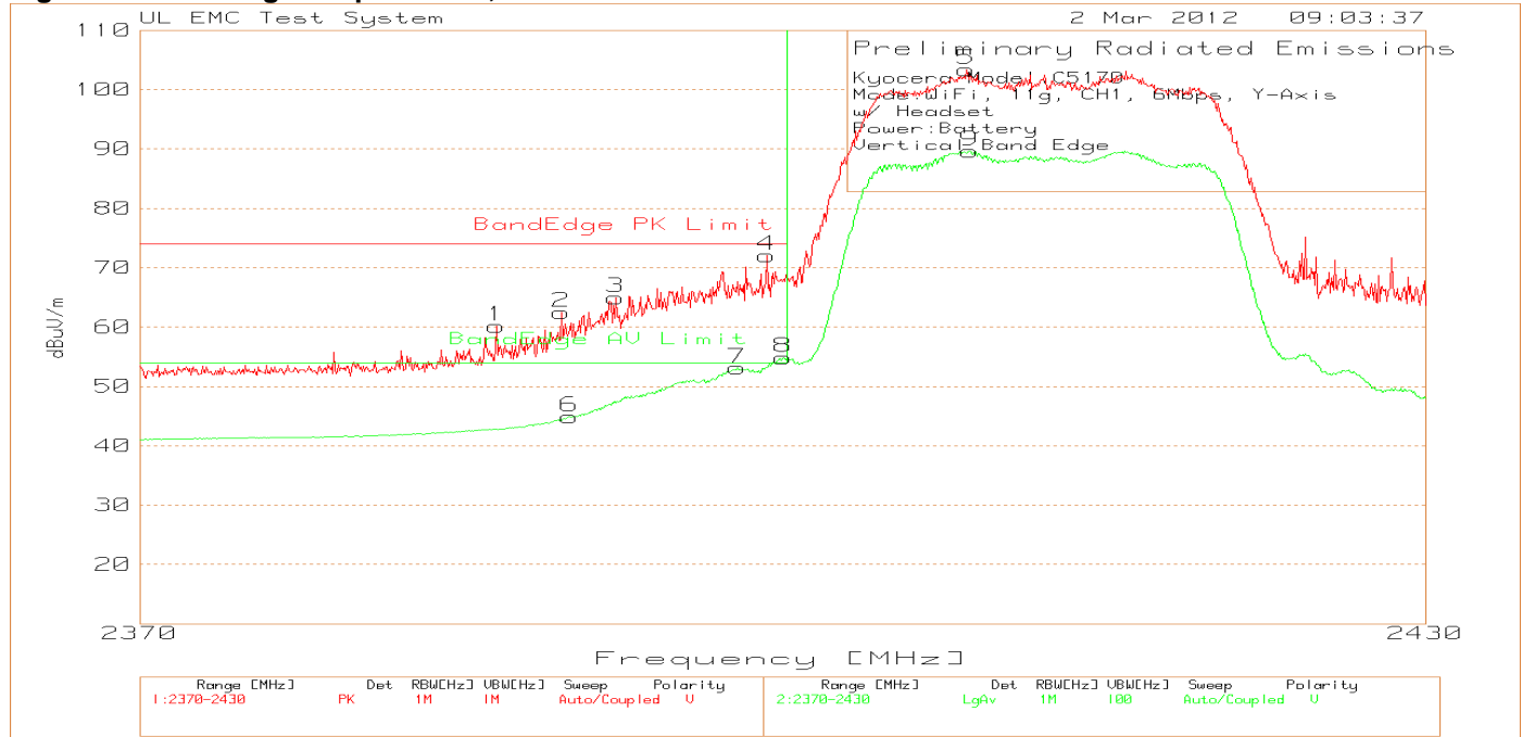
Figure 22 Band-edge Graph Y-Axis, Vertical
