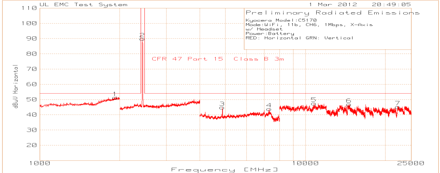
Figure 9 Radiated Emissions Graph X-Axis
