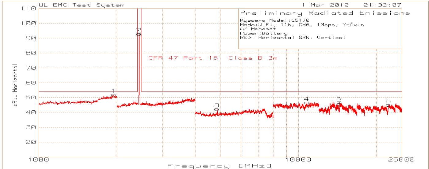
Figure 12 Radiated Emissions Graph Y-Axis
