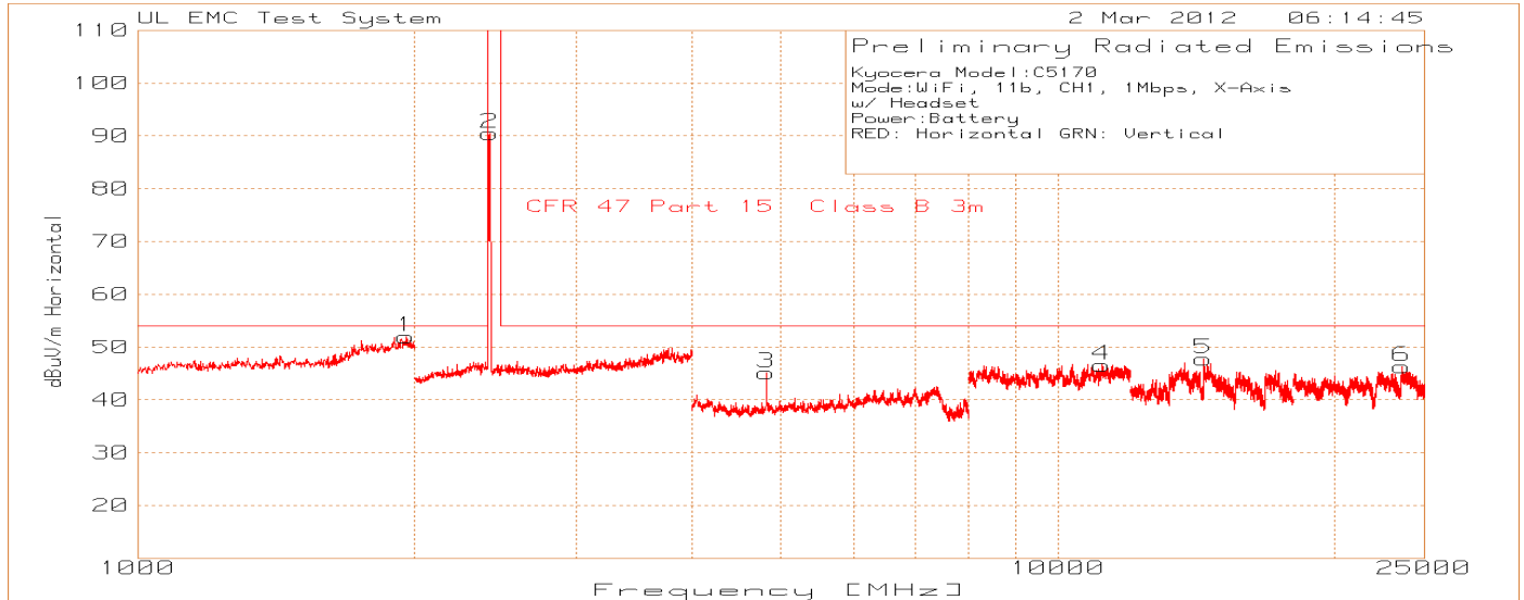
Figure 6 Radiated Emissions Graph X-Axis
