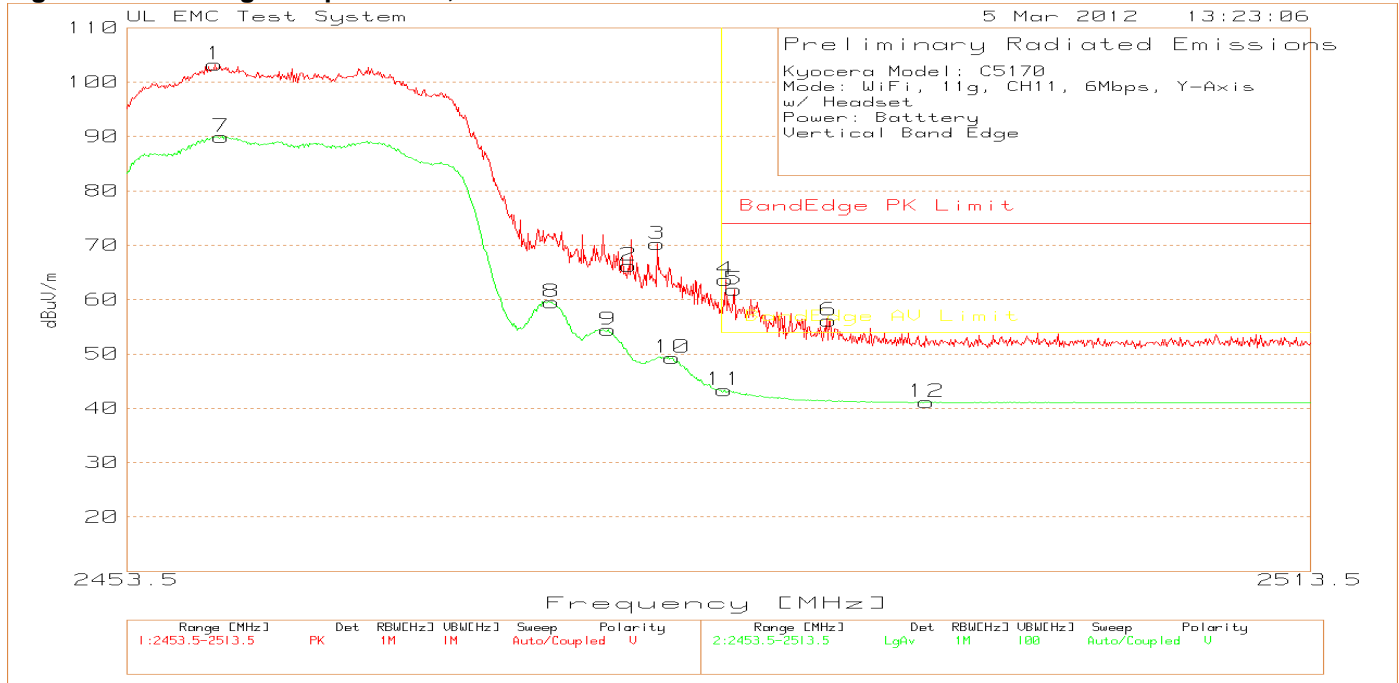
Figure 34 Band-edge Graph Y-Axis, Vertical
