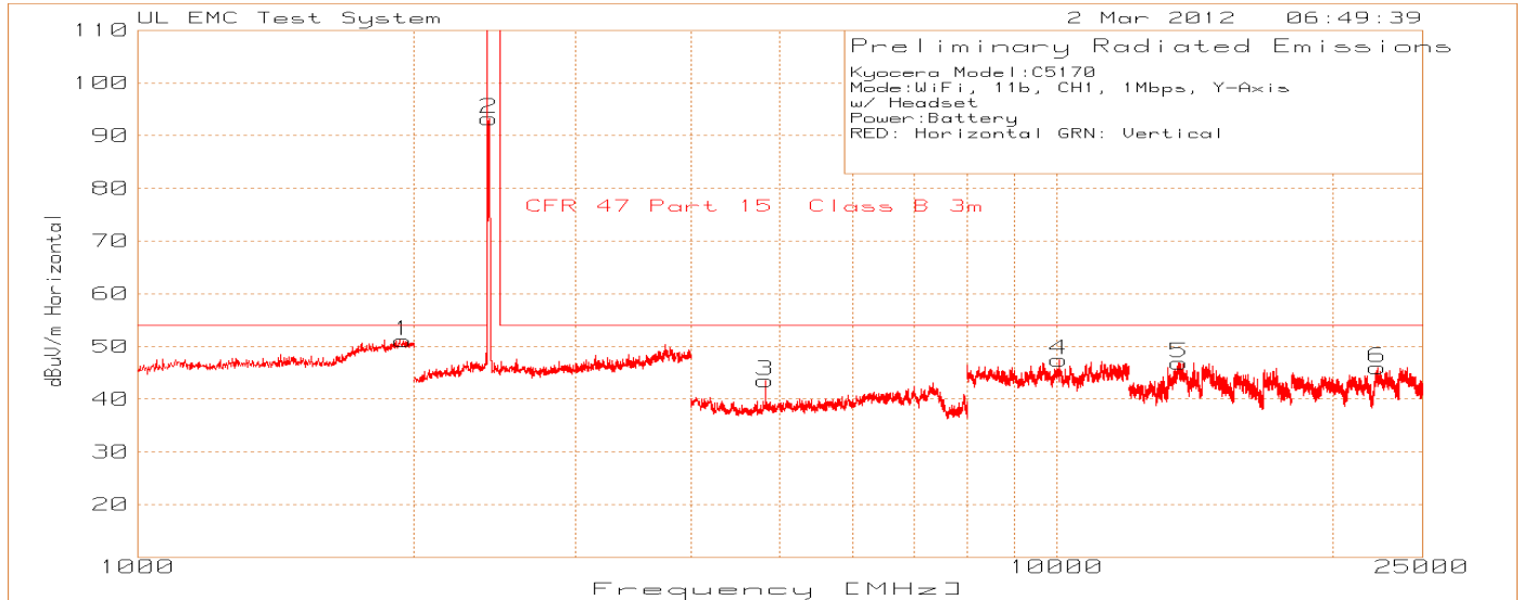
Figure 7 Radiated Emissions Graph Y-Axis
