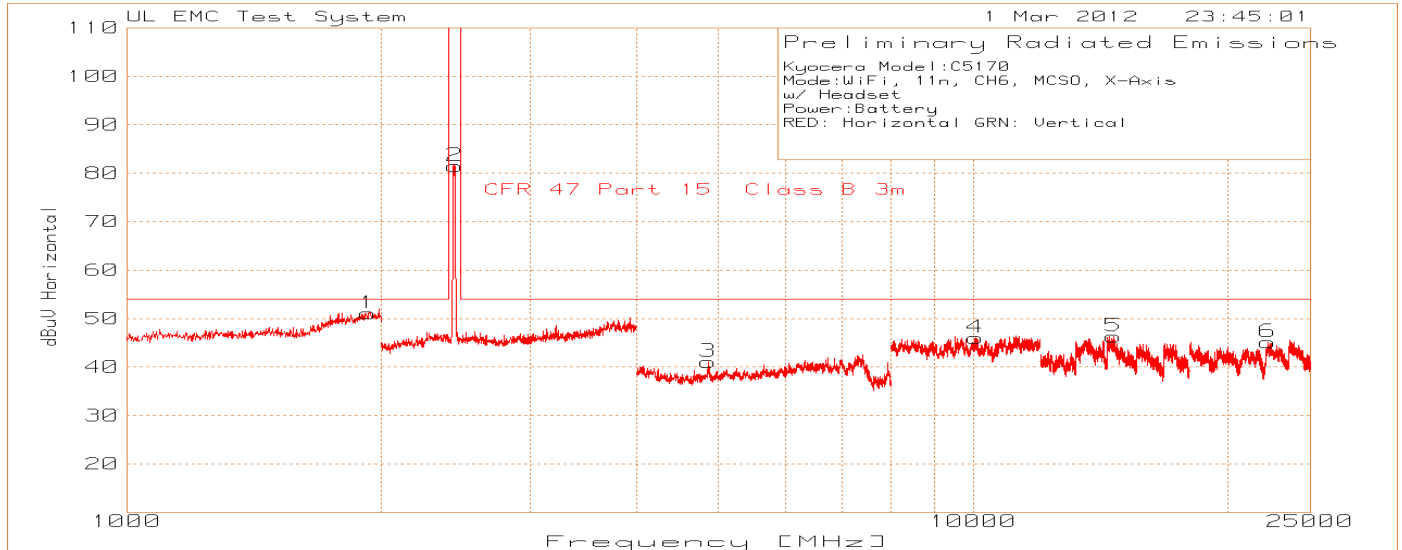
Figure 11 Radiated Emissions Graph X-Axis
