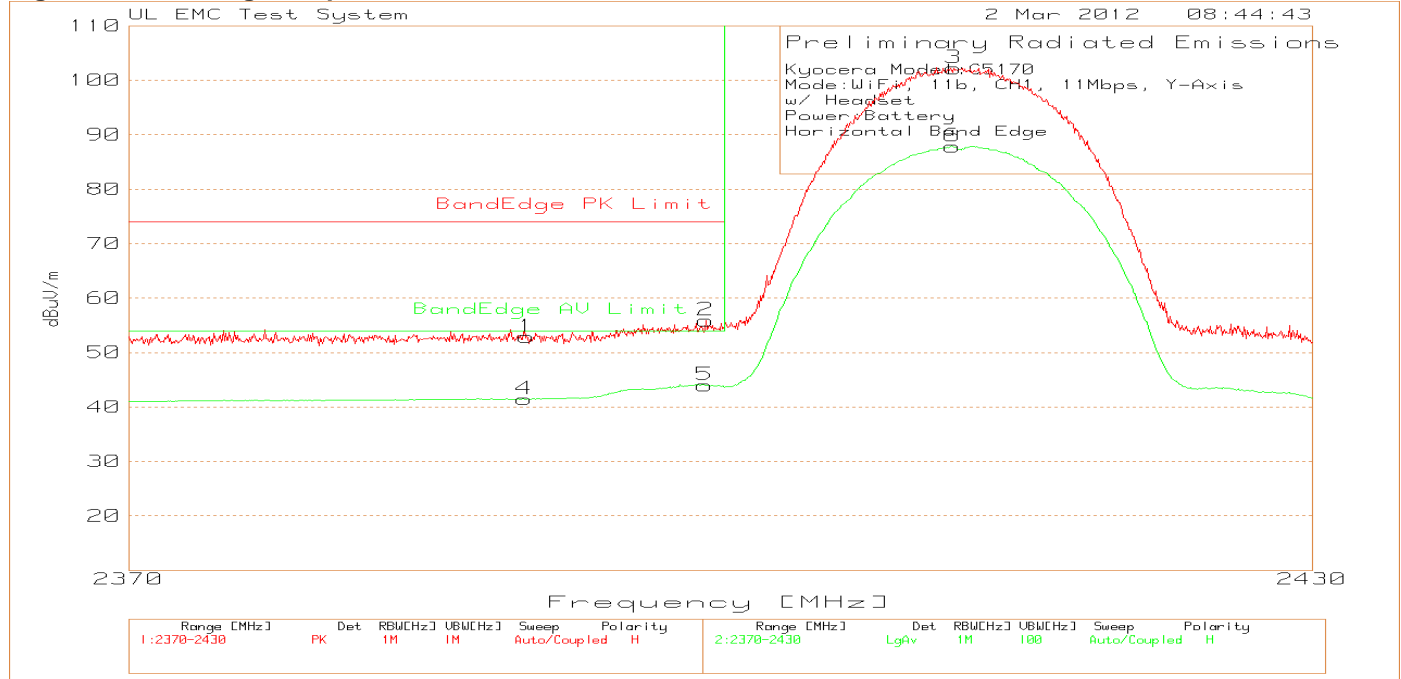
Figure 19 Band-edge Graph Y-Axis, Horizontal
