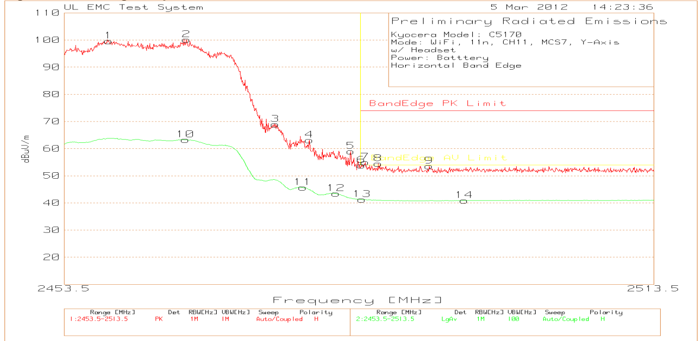
Figure 39 Band-edge Graph Y-Axis, Horizontal
