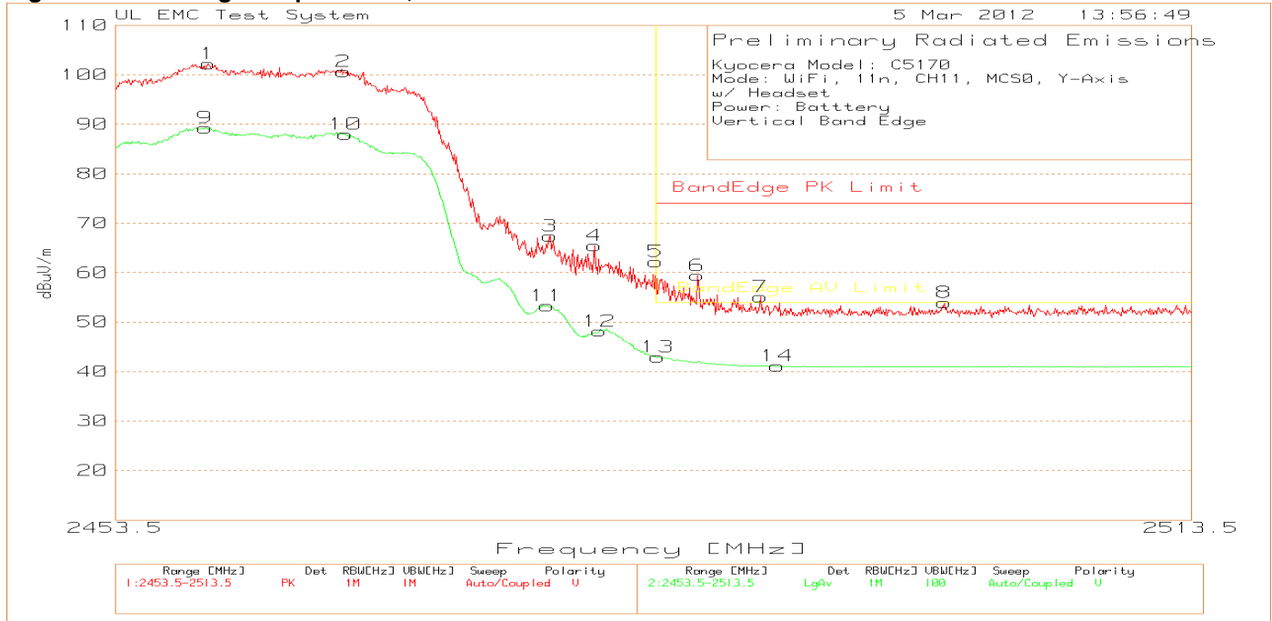
Figure 38 Band-edge Graph Y-Axis, Vertical
