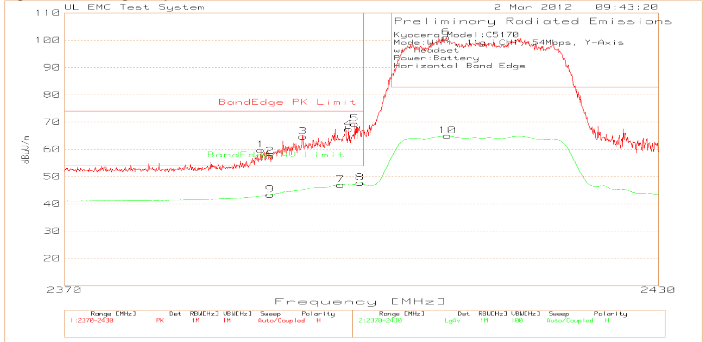
Figure 23 Band-edge Graph Y-Axis, Horizontal
