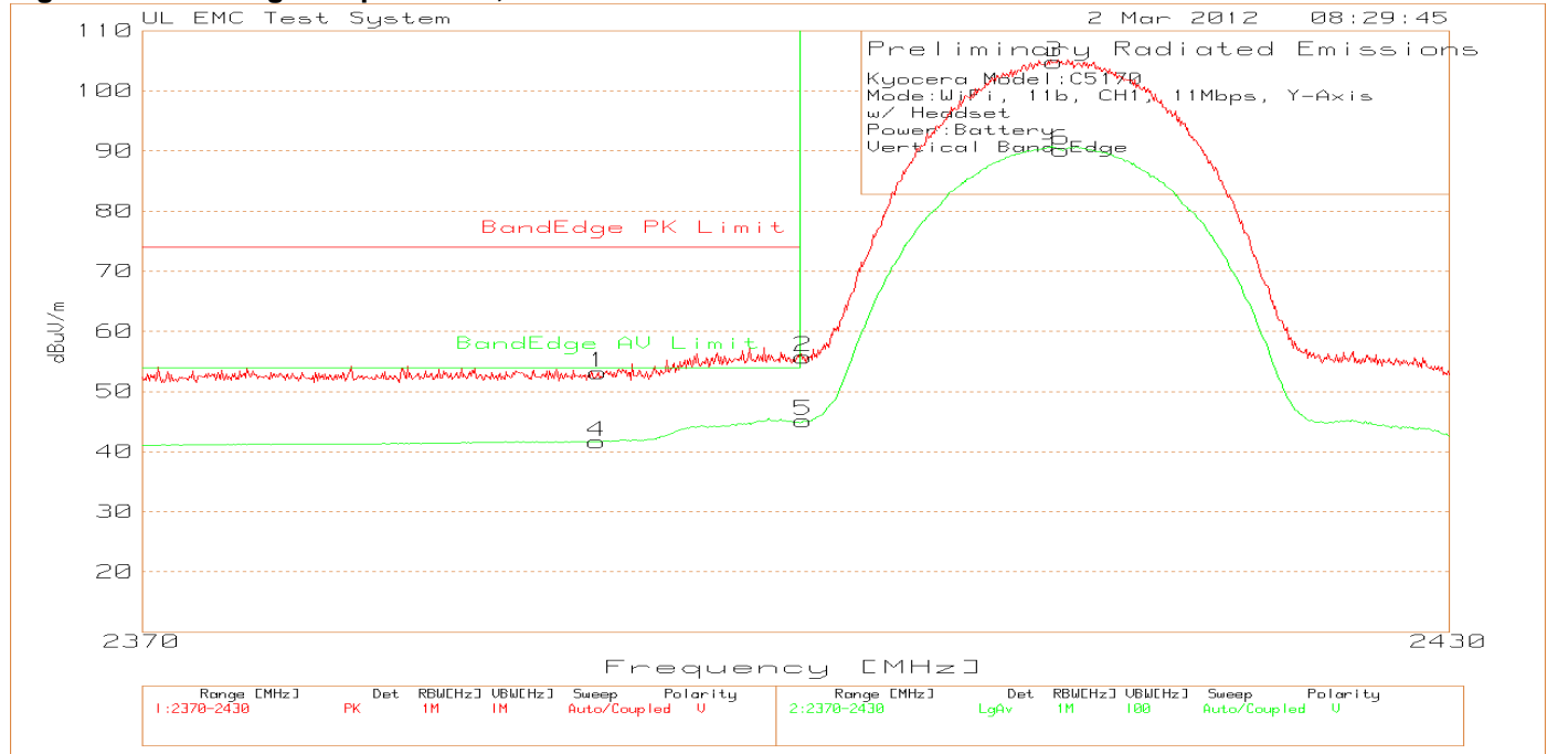
Figure 20 Band-edge Graph Y-Axis, Vertical
