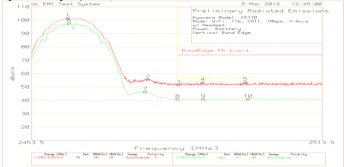
Figure 30 Band-edge Graph Y-Axis, Vertical
