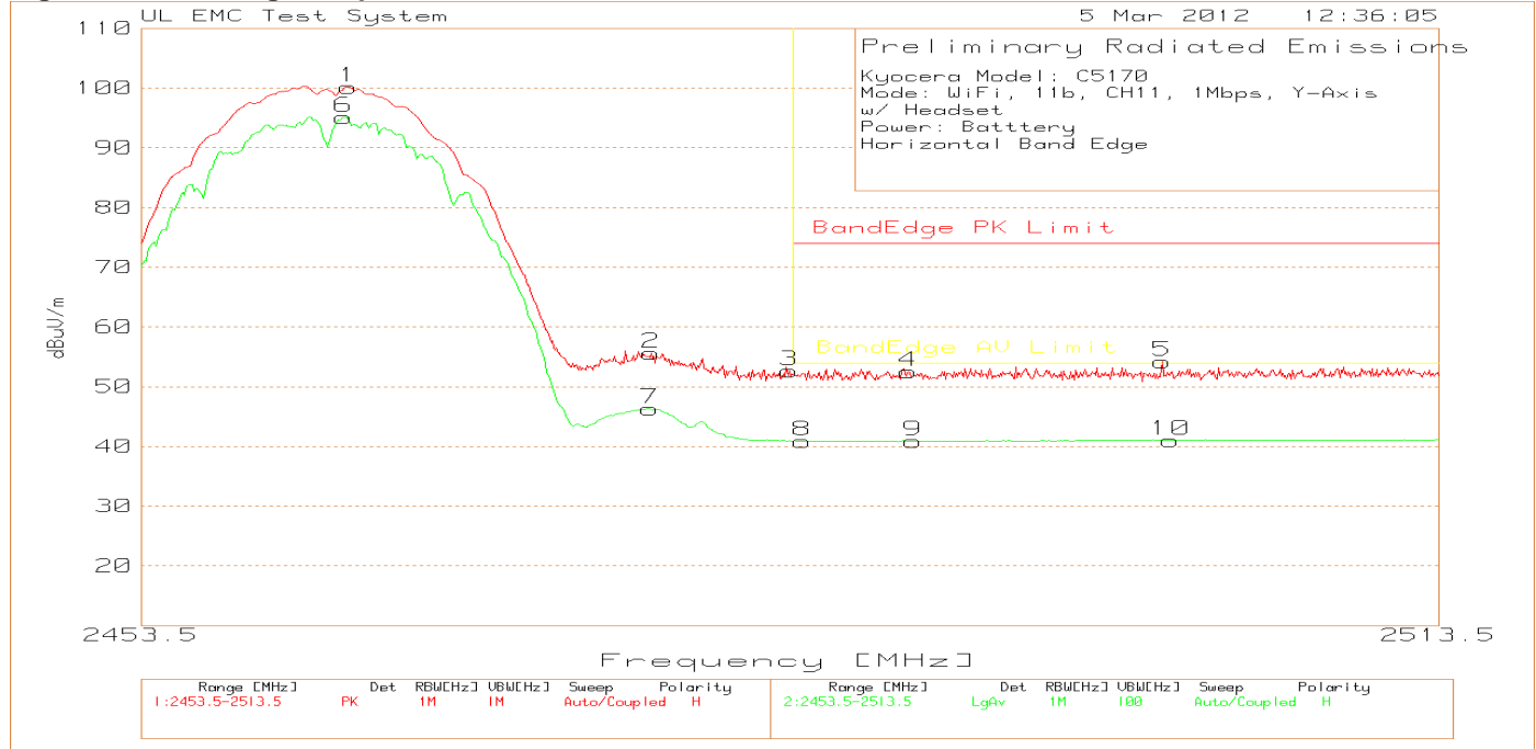
Figure 29 Band-edge Graph Y-Axis, Horizontal
