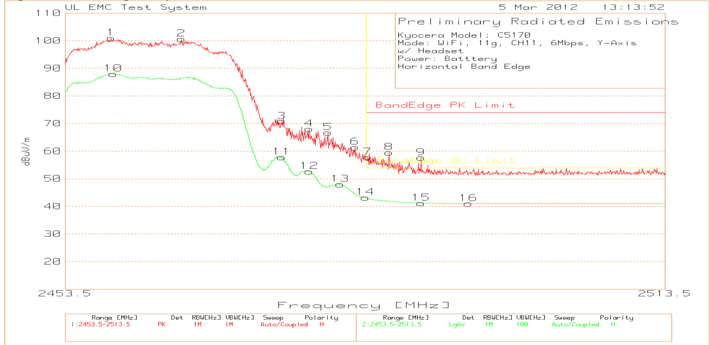
Figure 33 Band-edge Graph Y-Axis, Horizontal
