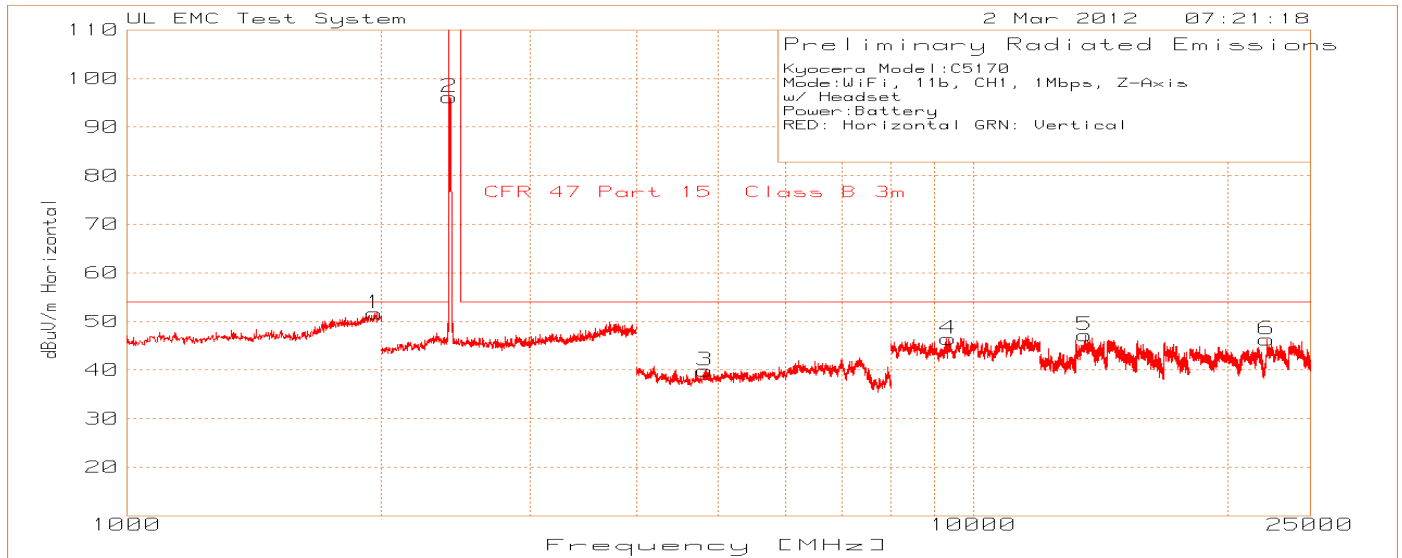
Figure 8 Radiated Emissions Graph Z-Axis
