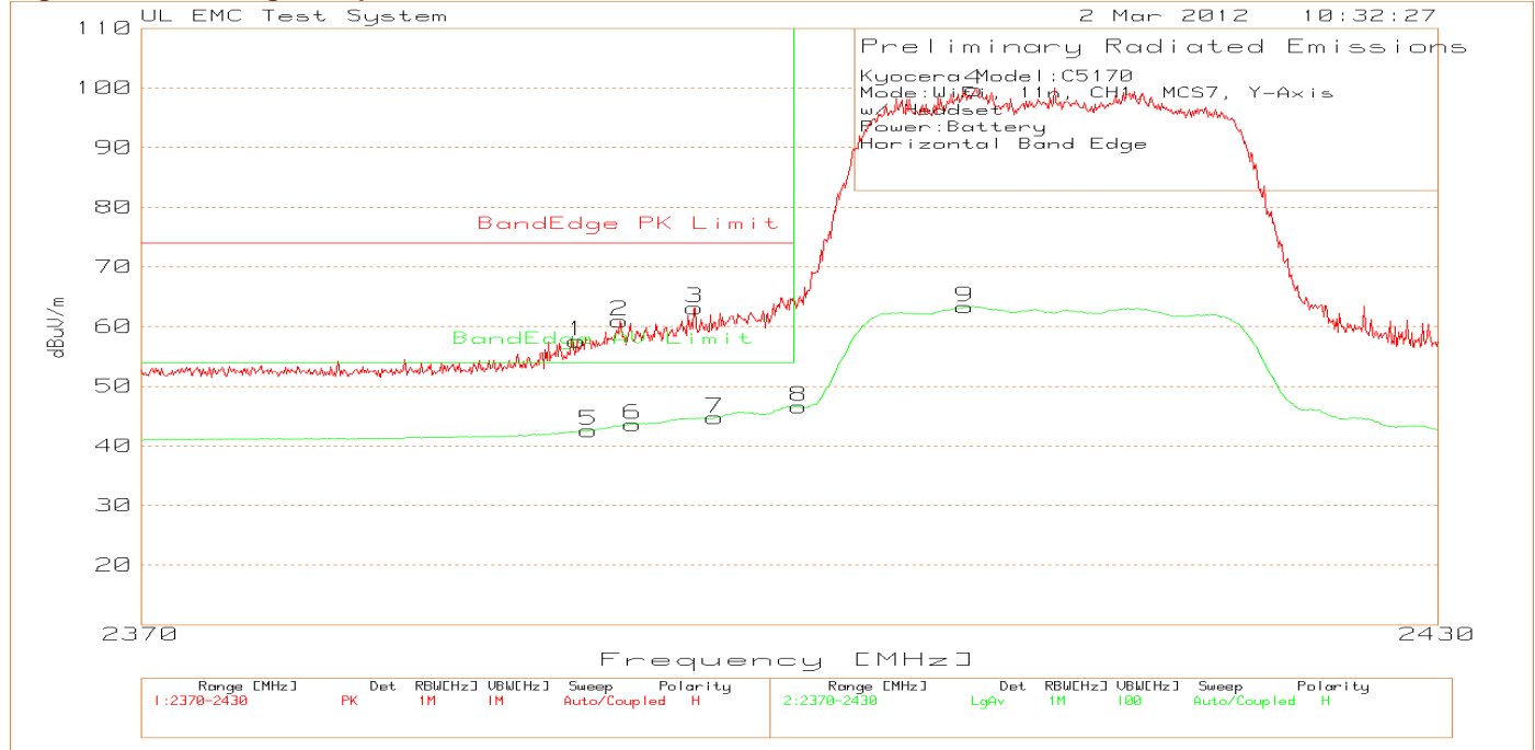
Figure 27 Band-edge Graph Y-Axis, Horizontal
