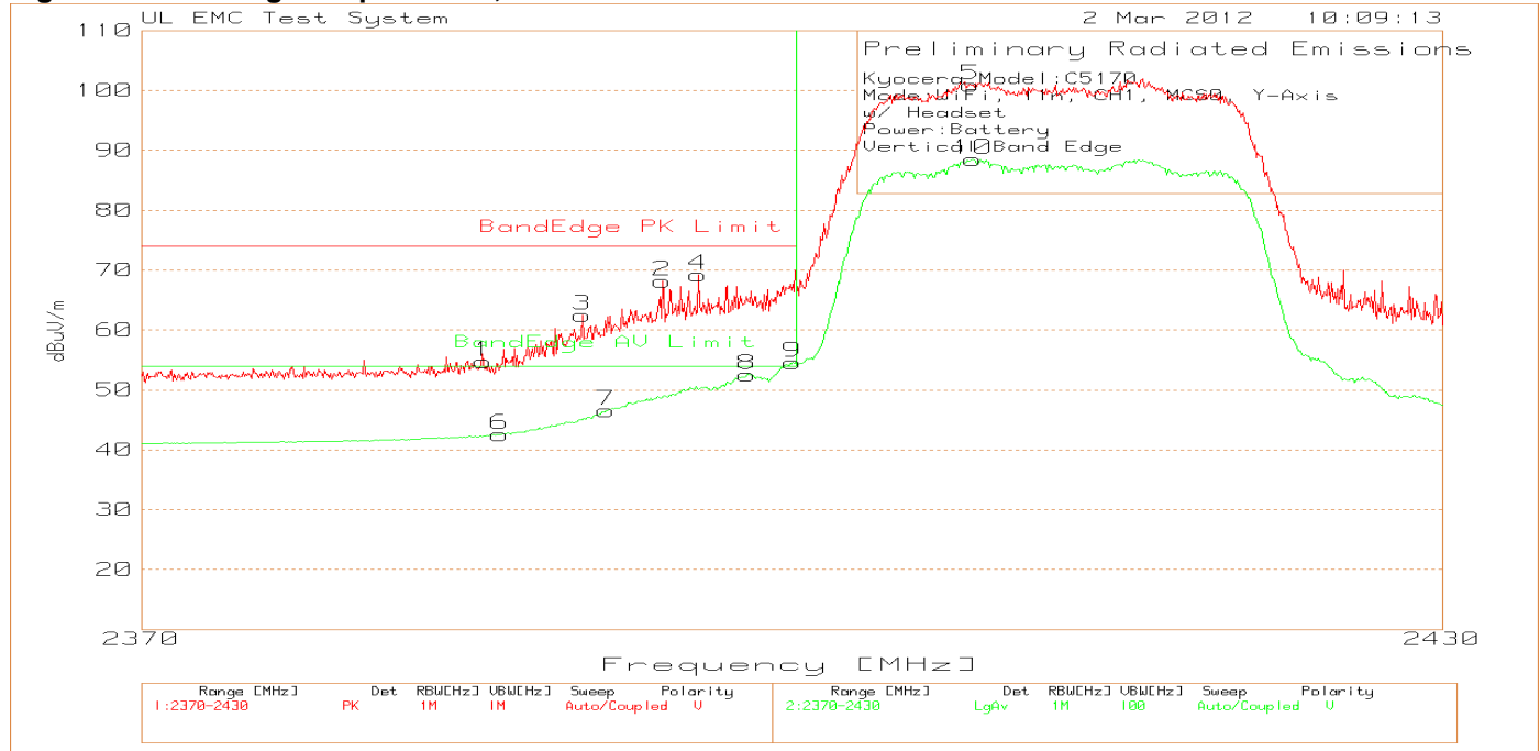
Figure 26 Band-edge Graph Y-Axis, Vertical
