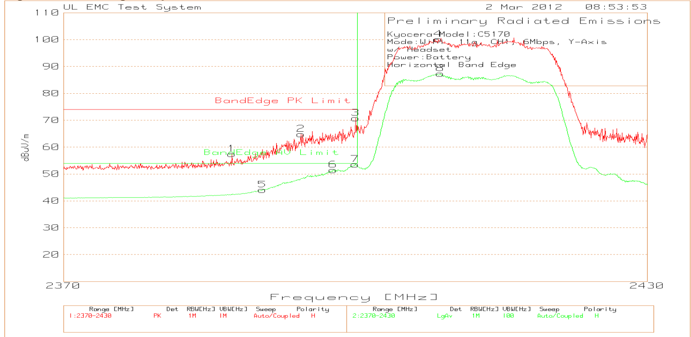
Figure 21 Band-edge Graph Y-Axis, Horizontal
