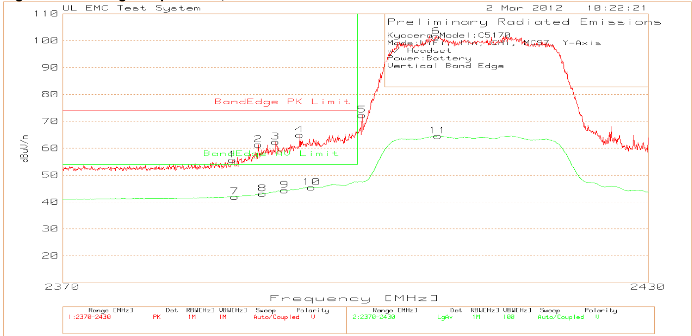
Figure 28 Band-edge Graph Y-Axis, Vertical
