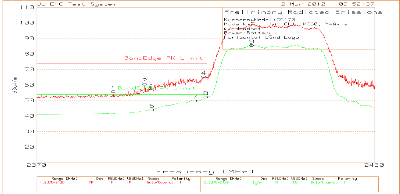
Figure 25 Band-edge Graph Y-Axis, Horizontal
