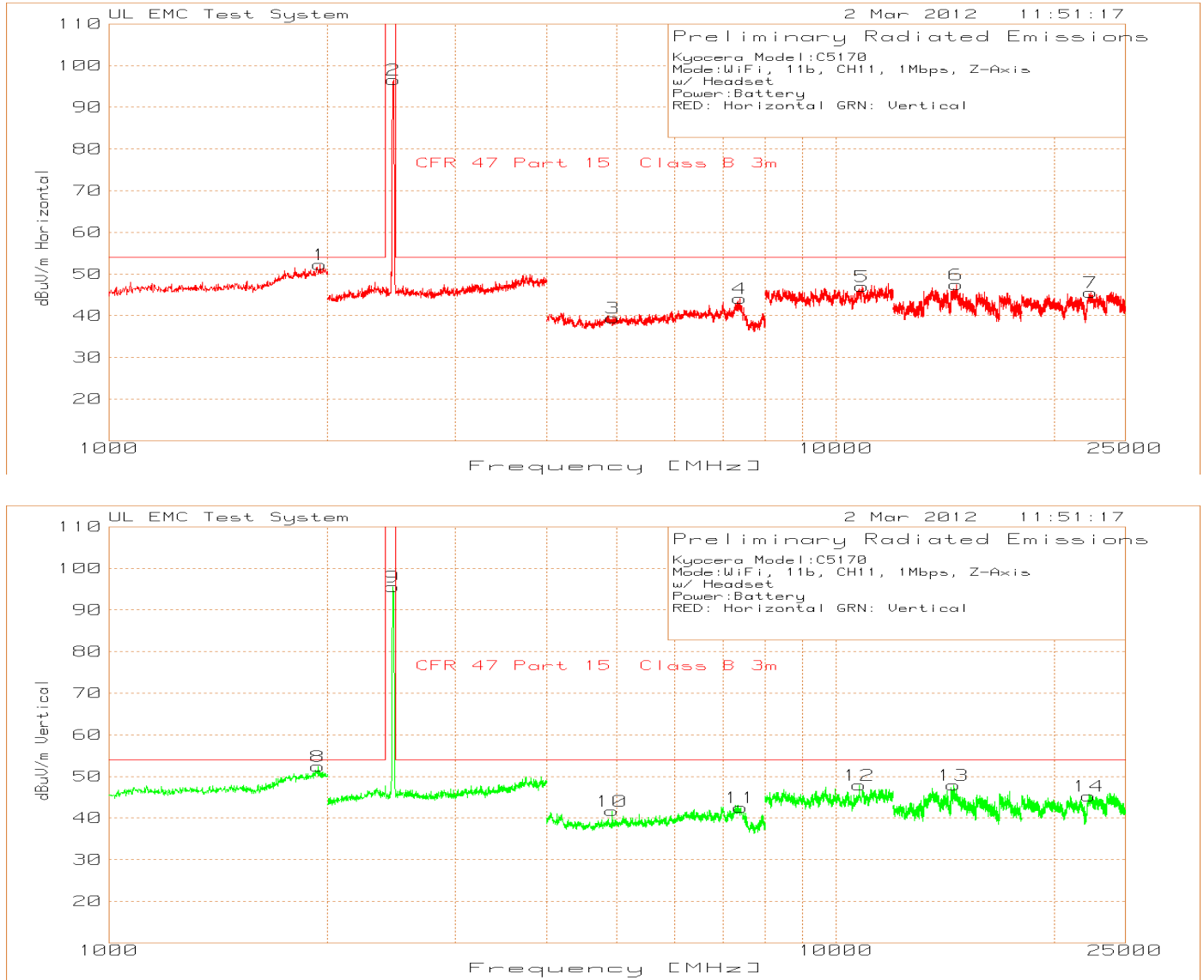
Figure 16 Radiated Emissions Graph Z-Axis
