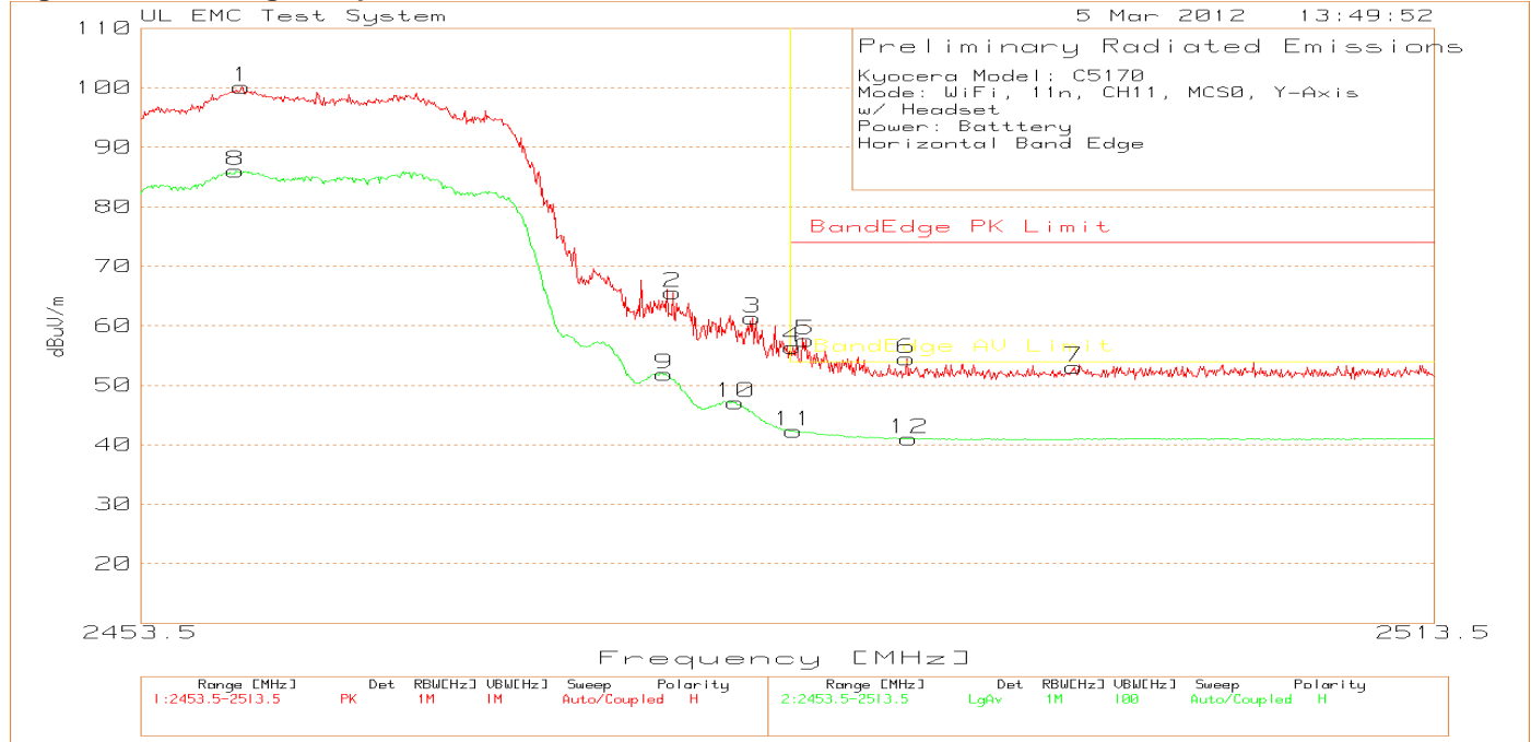
Figure 37 Band-edge Graph Y-Axis, Horizontal
