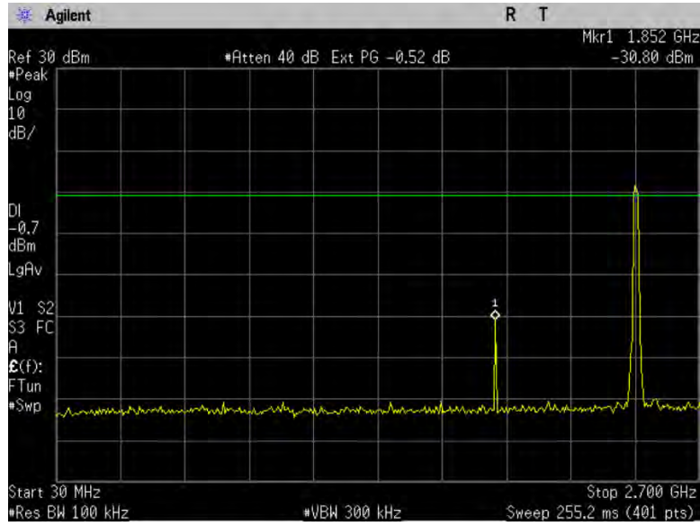
Figure 10-2b1: Conducted Spurious Emissions, 802.11g, Ch 6
