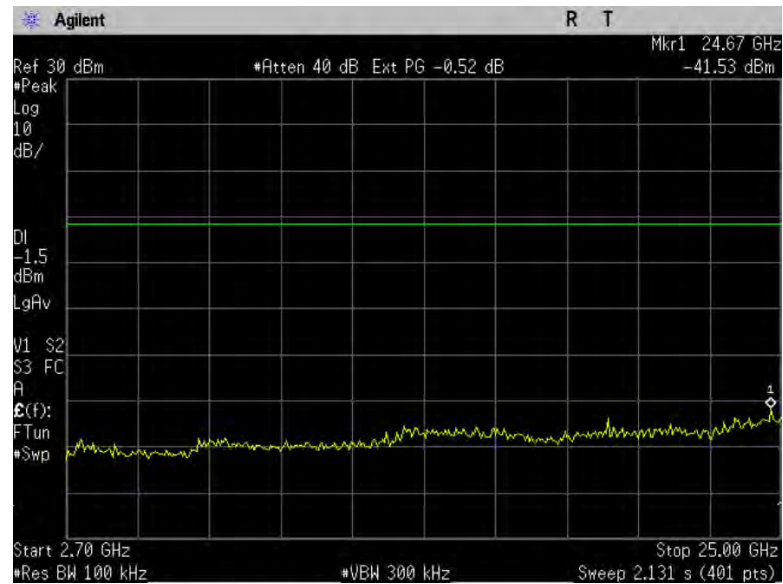
Figure 10-1b2: Conducted Spurious Emissions, 802.11b, Ch 6
