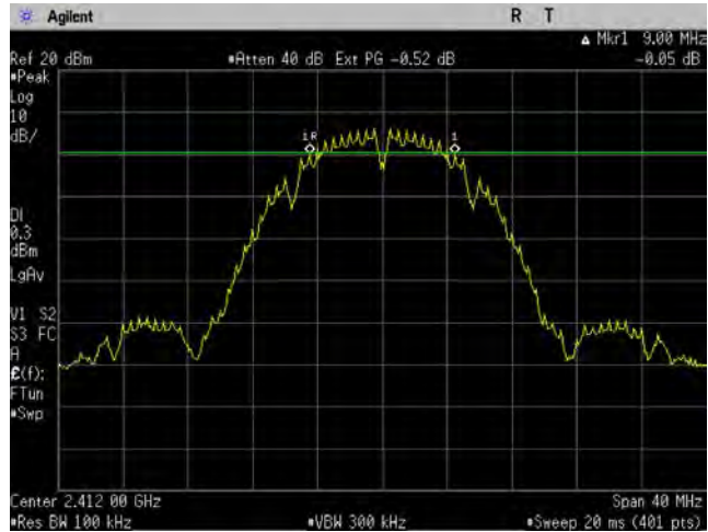
Figure 6-1a: 6 dB Bandwidth, 802.11b 1Mbps, Ch 1.
