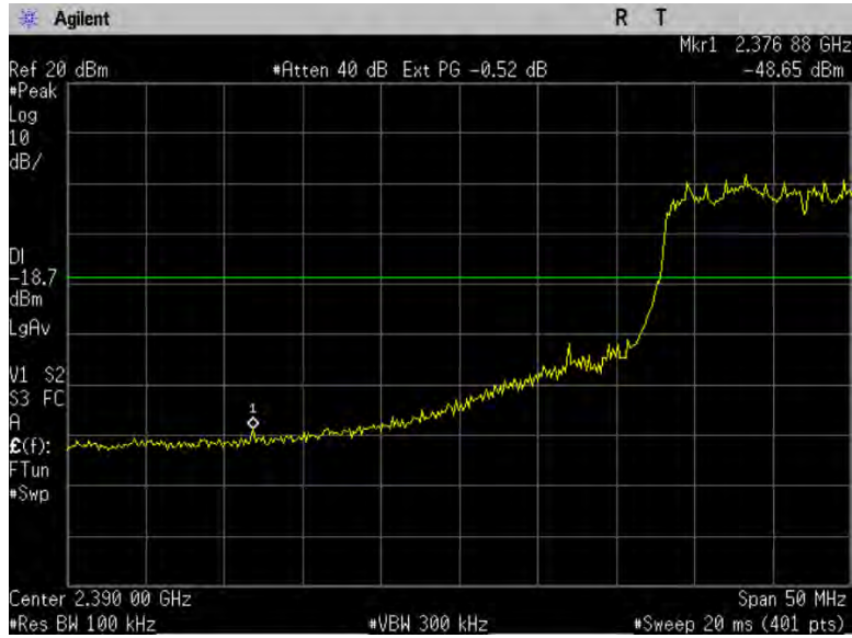
Figure 9-3a: Low band edge, 802.11n, ch1.
