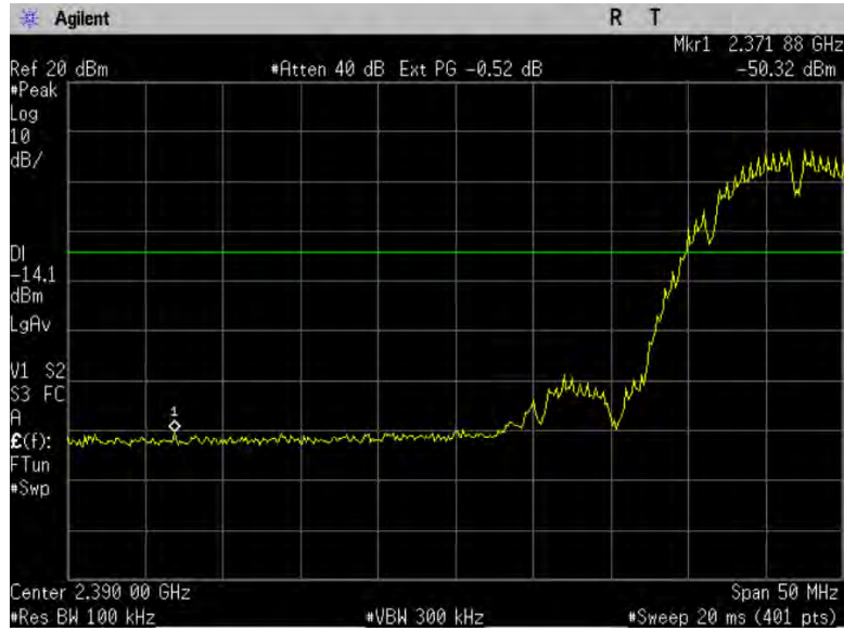
Figure 9-1a: Low band edge, 802.11b, ch1
