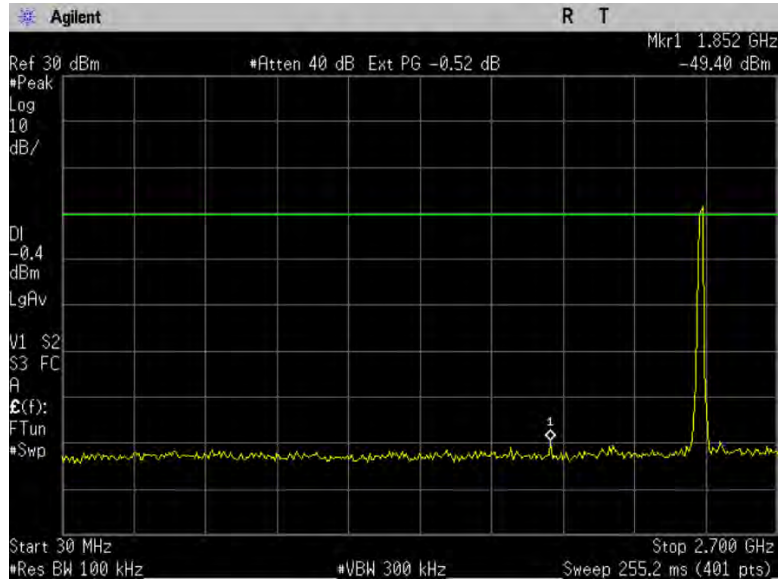
Figure 10-2a1: Conducted Spurious Emissions, 802.11g, Ch 1
