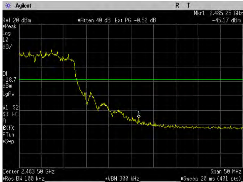
Figure 9-3b: High band edge, 802.11n, ch11.
