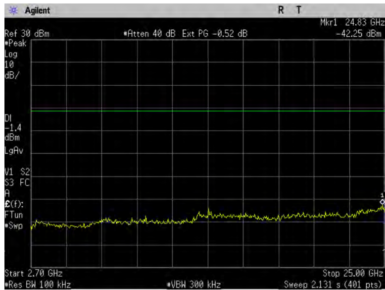
Figure 10-3a2: Conducted Spurious Emissions, 802.11n, Ch 1
