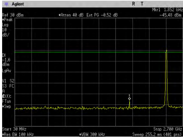
Figure 10-3b1: Conducted Spurious Emissions, 802.11n, Ch 6
