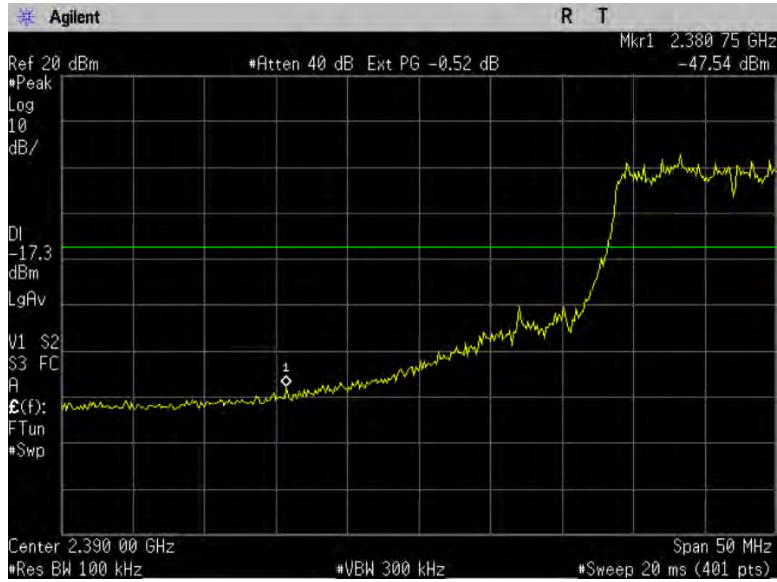
Figure 9-2a: Low band edge, 802.11g, ch1.
