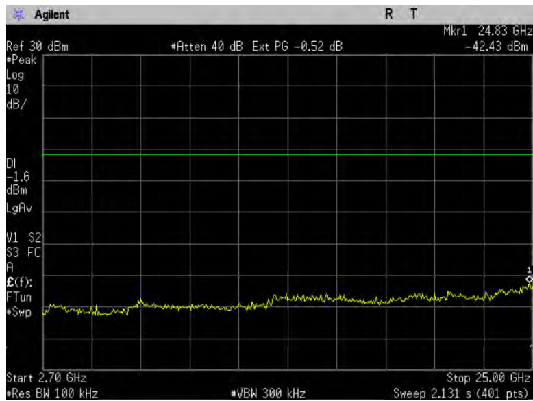
Figure 10-3b2: Conducted Spurious Emissions, 802.11n, Ch 6
