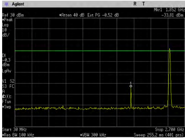
Figure 10-2c1: Conducted Spurious Emissions, 802.11g, Ch 11
