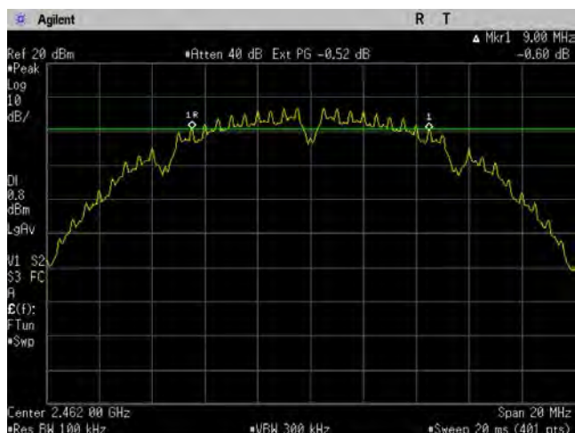
Figure 6-1c: 6 dB Bandwidth, 802.11b 1Mbps, Ch 11.
