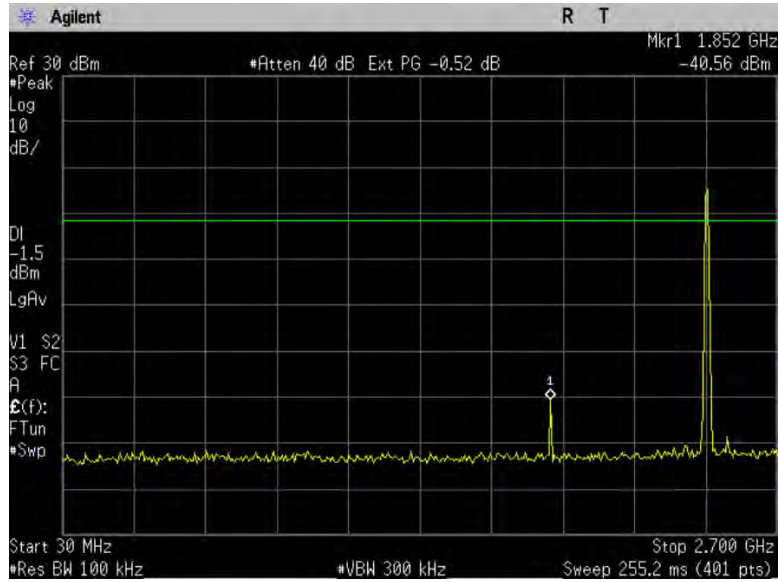
Figure 10-1b1: Conducted Spurious Emissions, 802.11b, Ch 6
