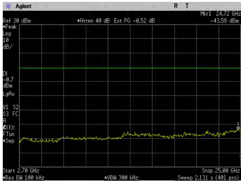
Figure 10-2b2: Conducted Spurious Emissions, 802.11g, Ch 6
