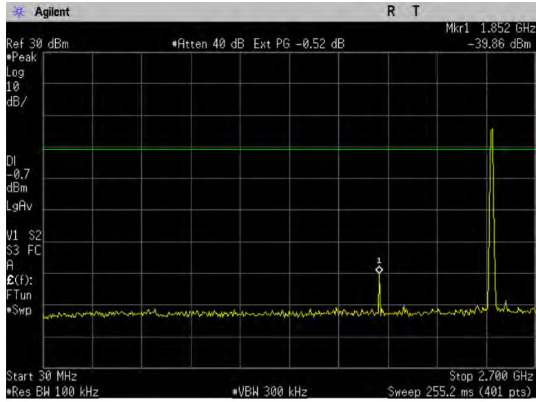
Figure 10-1c1: Conducted Spurious Emissions, 802.11b, Ch 11
