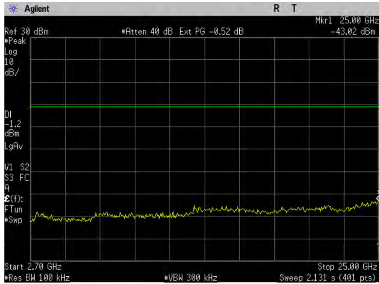
Figure 10-1a2: Conducted Spurious Emissions, 802.11b, Ch 1
