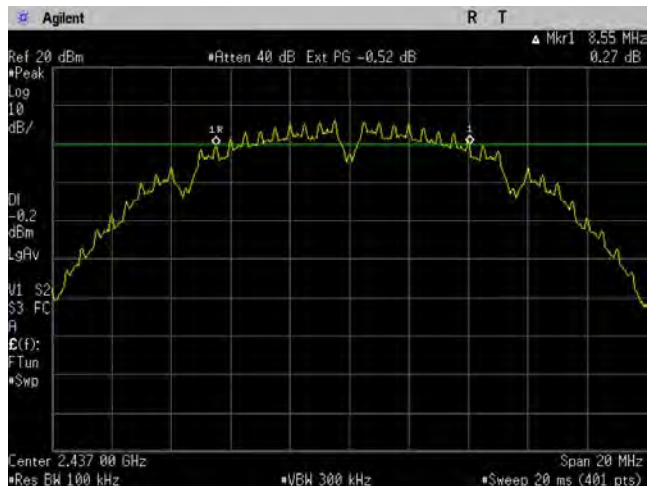
Figure 6-1b: 6 dB Bandwidth, 802.11b 1Mbps, Ch 6.
