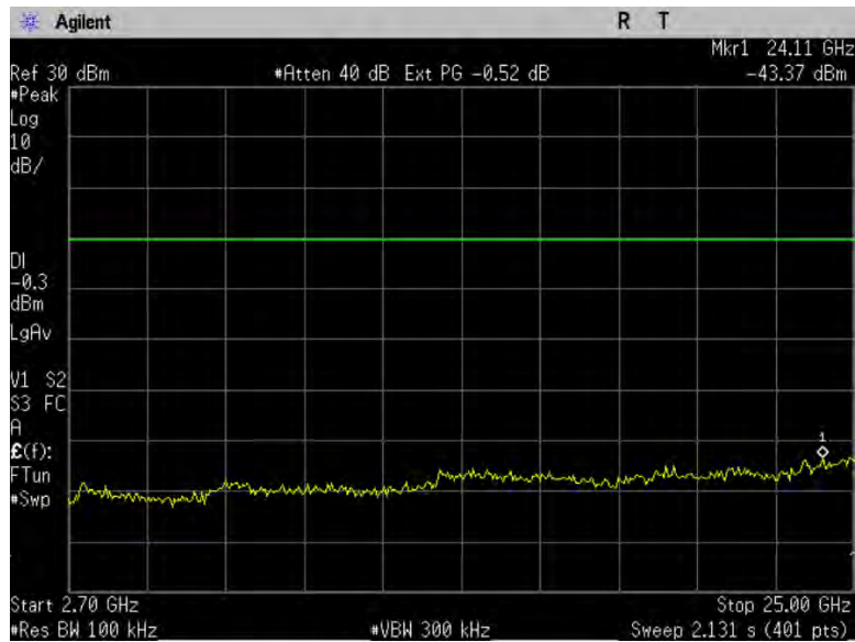
Figure 10-2c2: Conducted Spurious Emissions, 802.11g, Ch 11
