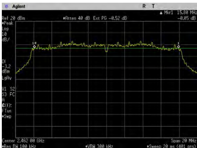
Figure 6-2c: 6 dB Bandwidth, 802.11g 6Mbps, Ch 11.
