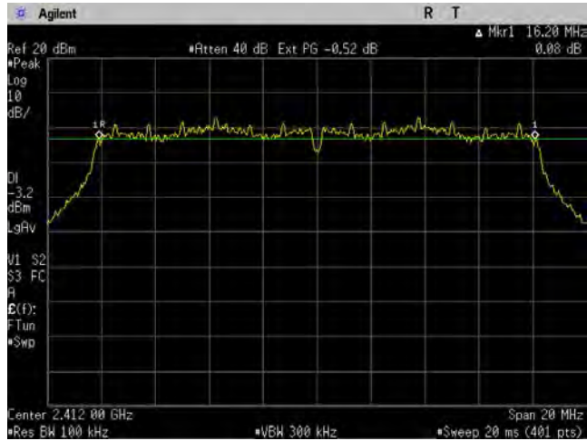
Figure 6-2a: 6 dB Bandwidth, 802.11g 6Mbps, Ch 1.
