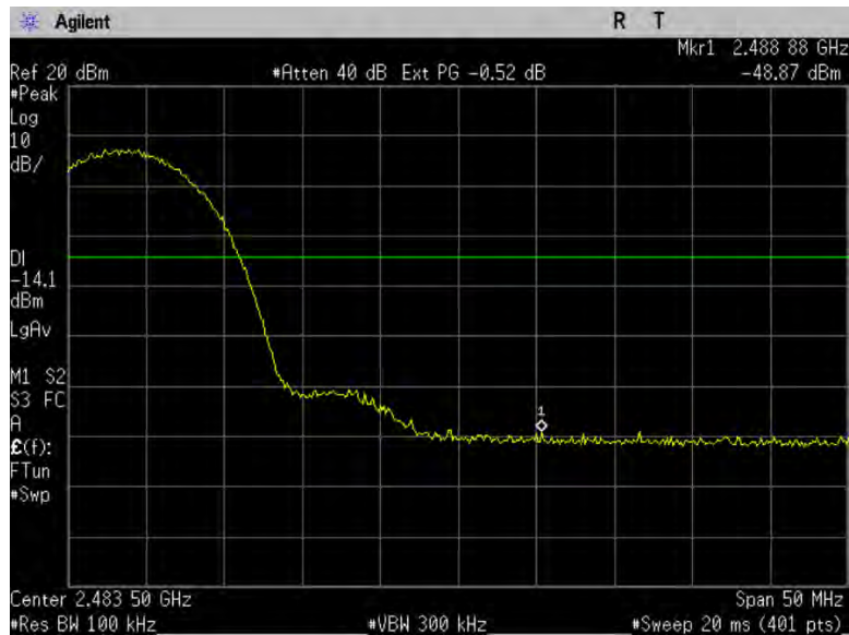
Figure 9-1b: High band edge, 802.11b, ch11.
