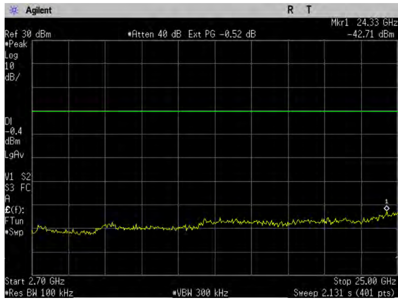
Figure 10-2a2: Conducted Spurious Emissions, 802.11g, Ch 1
