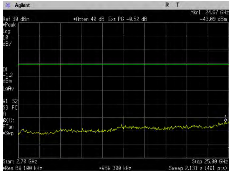
Figure 10-3c2: Conducted Spurious Emissions, 802.11n, Ch 11
