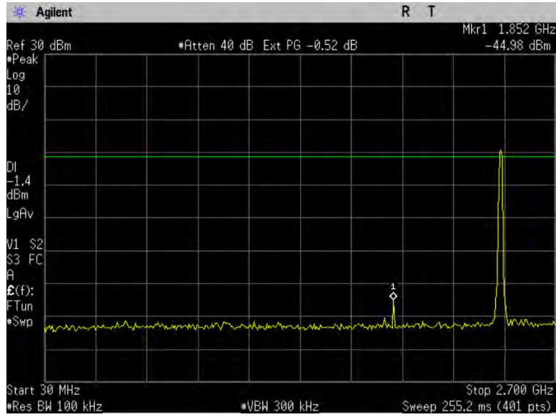
Figure 10-3a1: Conducted Spurious Emissions, 802.11n, Ch 1
