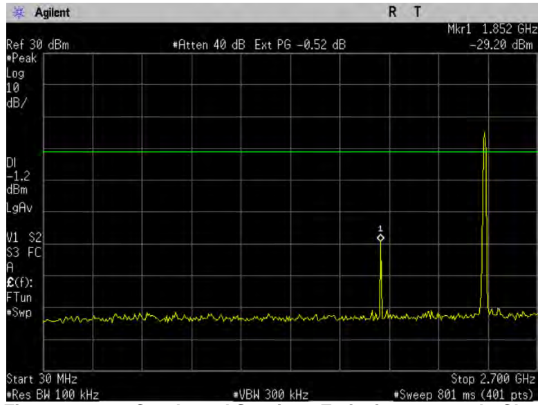
Figure 10-1a1: Conducted Spurious Emissions, 802.11b, Ch 1
