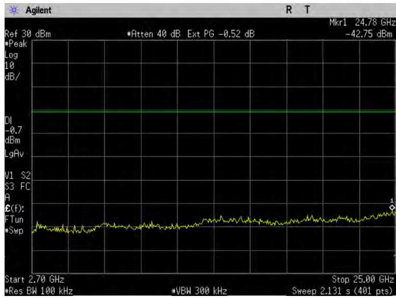
Figure 10-1c2: Conducted Spurious Emissions, 802.11b, Ch 11
