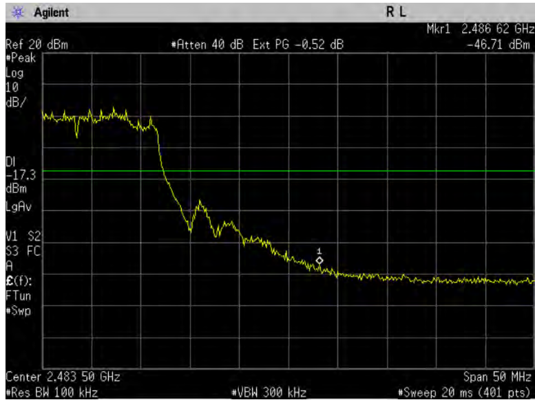
Figure 9-2b: High band edge, 802.11g, ch11.
