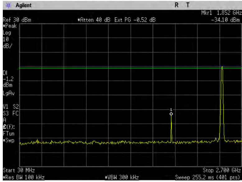
Figure 10-3c1: Conducted Spurious Emissions, 802.11n, Ch 11
