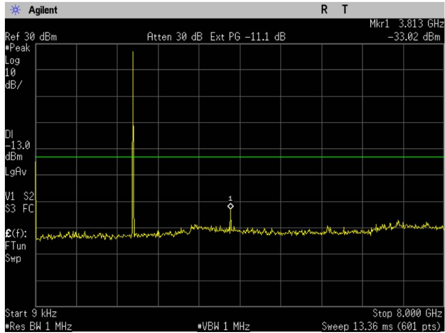
Figure 10-3a CDMA 1900 - Conducted Spurious Emission (CH 1175)
