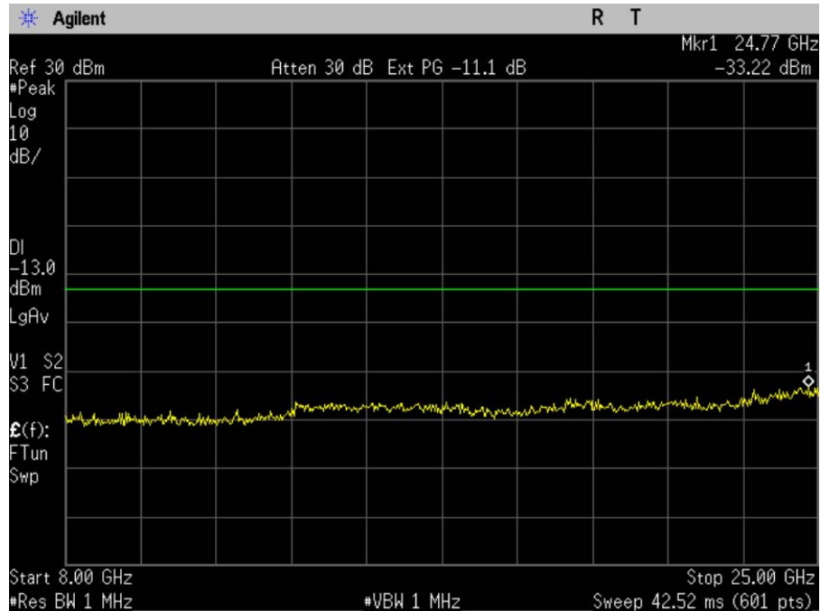
Figure 10-3b CDMA 1900 - Conducted Spurious Emission (CH 1175)
