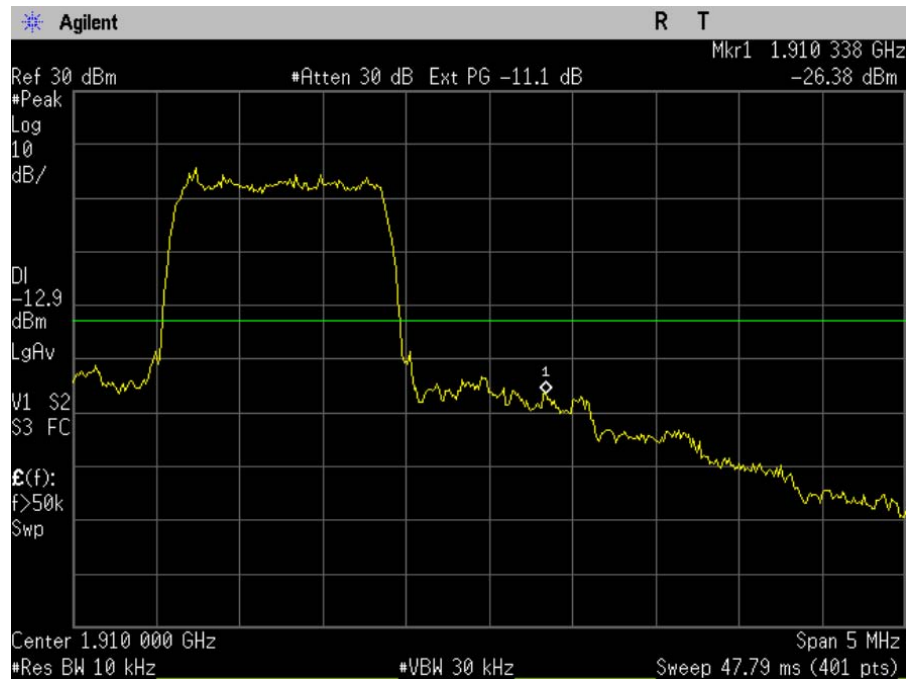
Figure 9-3 CDMA 1900 Upper Band Edge @ CH 1175
