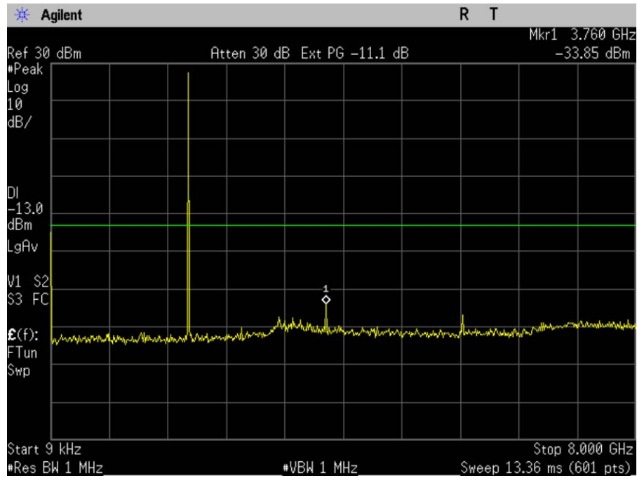
Figure 10-2a CDMA 1900 - Conducted Spurious Emission (CH 600)
