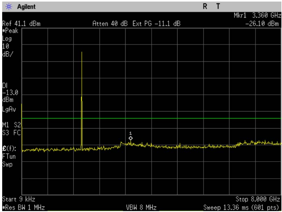
Figure 10-1a CDMA 1900 - Conducted Spurious Emission (CH 25)
