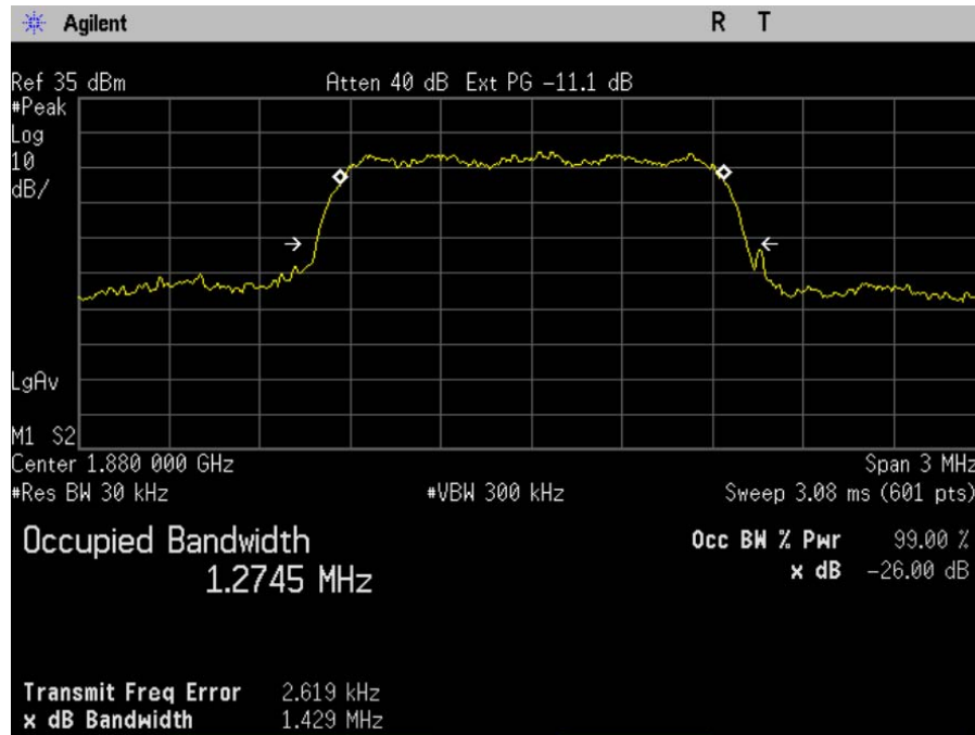
Figure 9-1 CDMA 1900 @ CH 600
