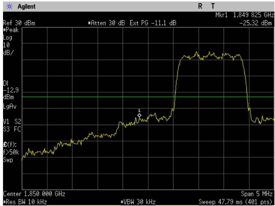
Figure 9-2 CDMA 1900 Lower Band Edge @ CH 25
