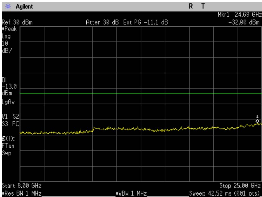
Figure 10-1b CDMA 1900 - Conducted Spurious Emission (CH 25)
