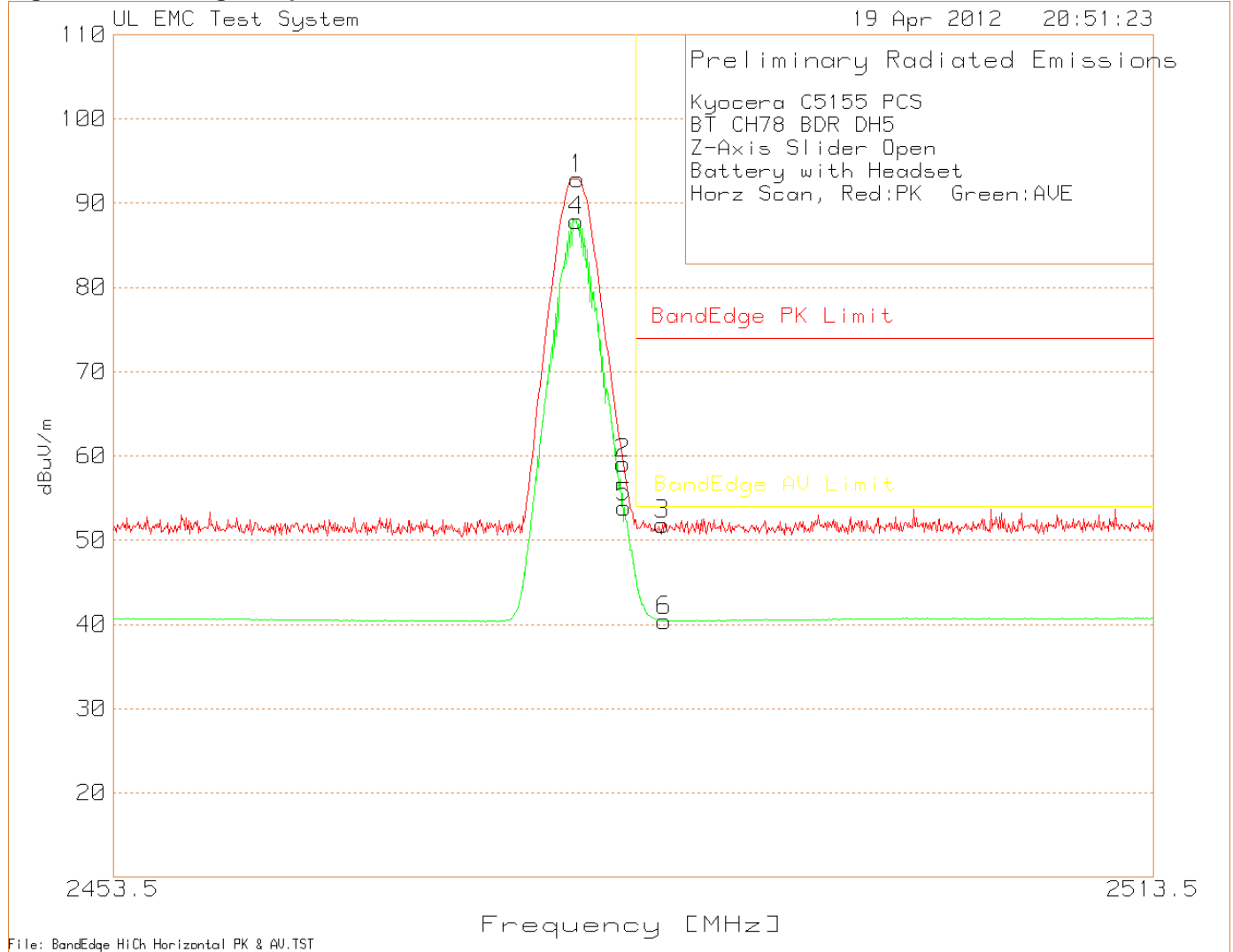
Figure 21 Band-edge Graph Z-Axis, Horizontal
