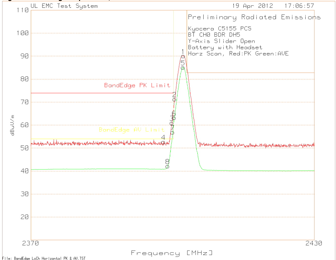
Figure 15 Band-edge Graph Y-Axis, Horizontal
