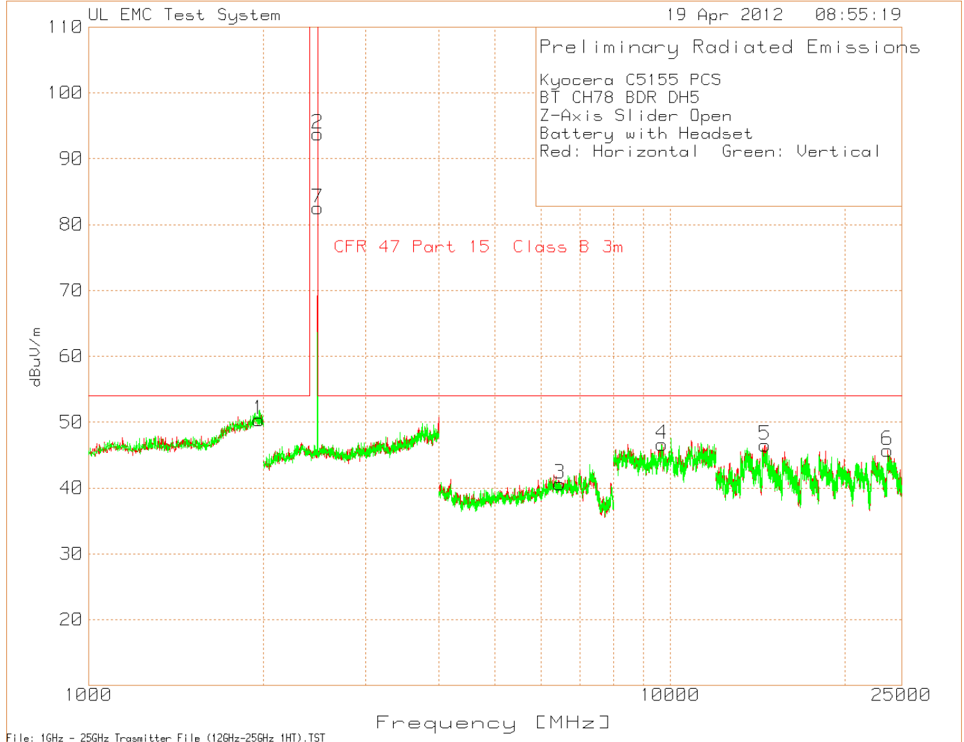
Figure 14 Radiated Emissions Graph Z-Axis
