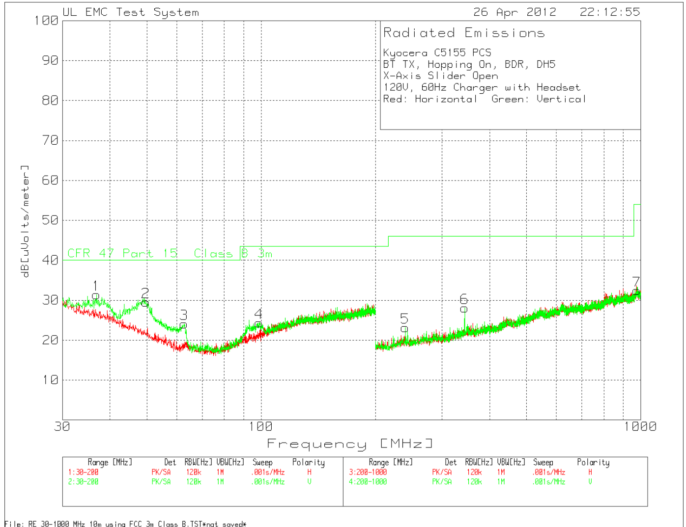
Figure 5 Radiated Emissions Graph X-Axis
