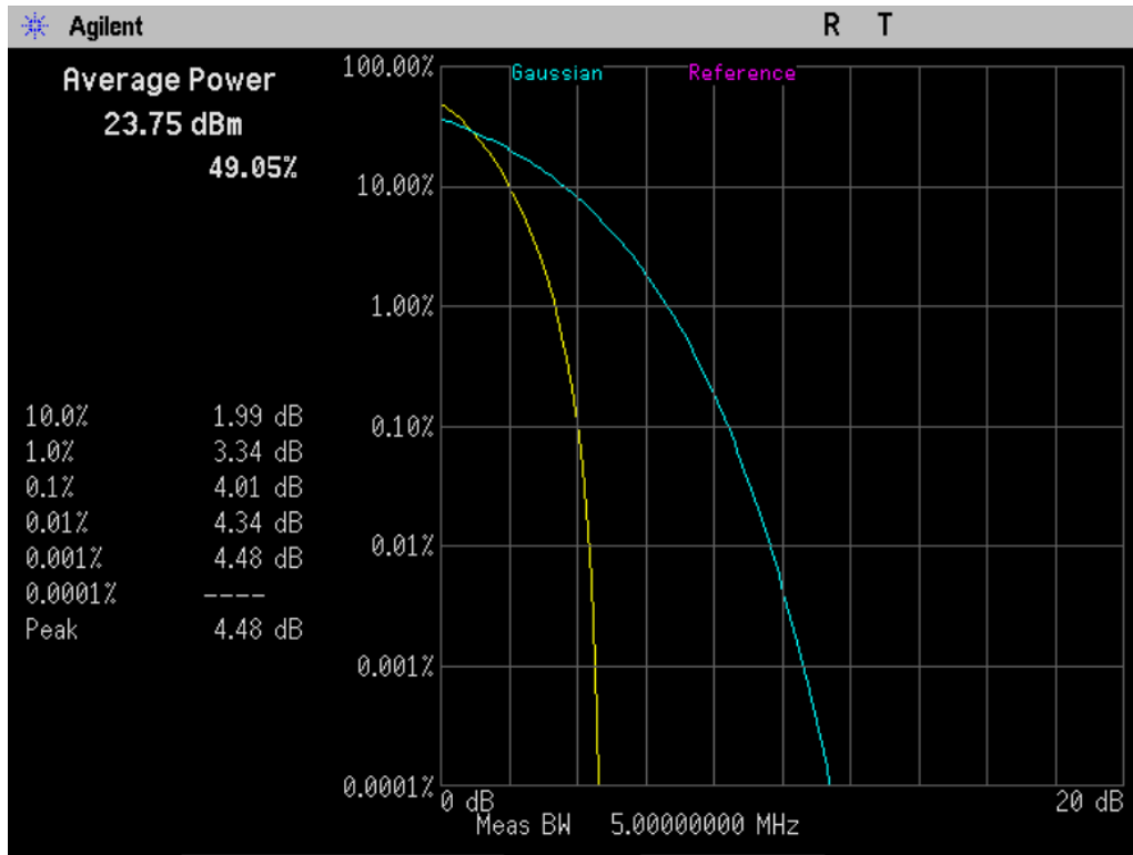
Figure 8-1 CCDF @ CH 600
