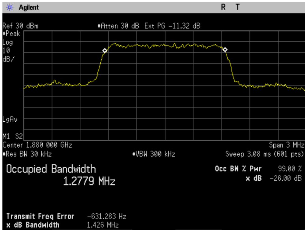
Figure 9-4 CDMA 1900 @ CH 600
