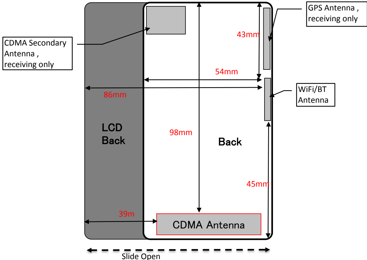
Figure 4.7 Antenna Distance to device edges
