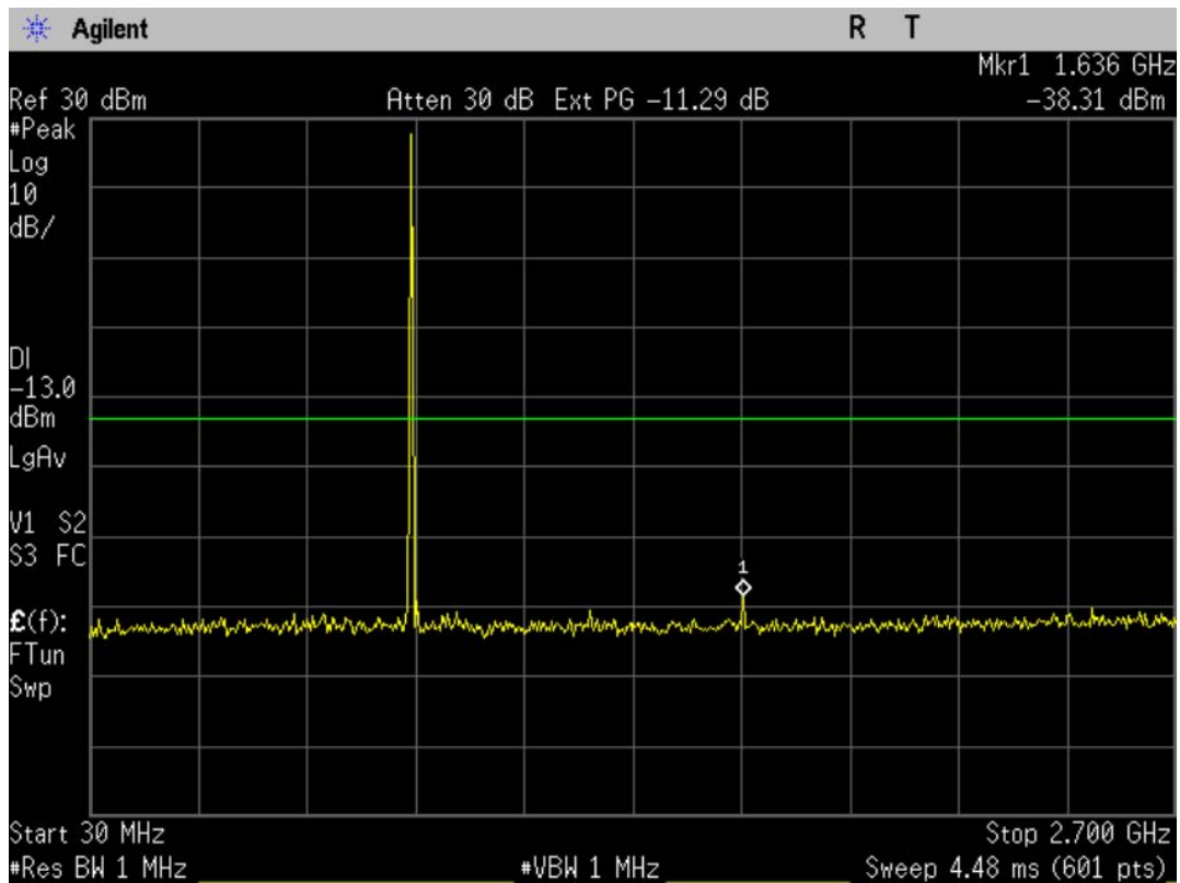
Figure 9-1a CDMA 800 BC-10 – Conducted Spurious Emission (CH 476)
