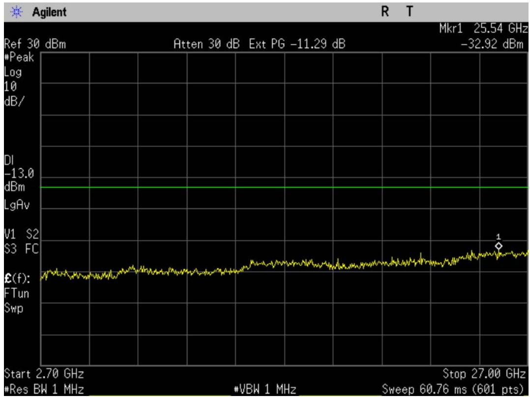
Figure 9-1b CDMA 800 BC-10 – Conducted Spurious Emission (CH 476)
