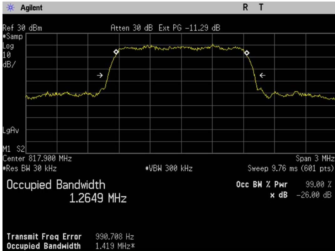
Figure 7-1 CDMA 800 BC-10 @ CH 476
