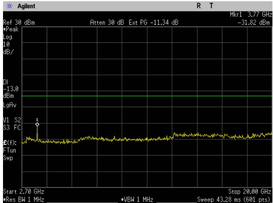
Figure 9-5b CDMA 1900 - Conducted Spurious Emission (CH 600)
