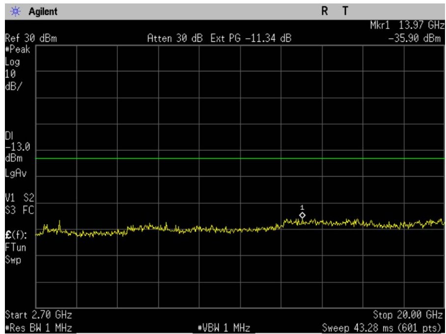
Figure 9-4b CDMA 1900 - Conducted Spurious Emission (CH 25)
