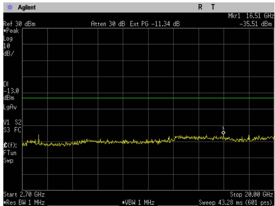
Figure 9-6b CDMA 1900 - Conducted Spurious Emission (CH 1175)
