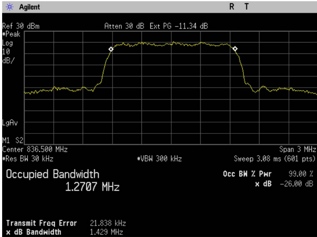
Figure 8-1 CDMA 800 @ CH 384
