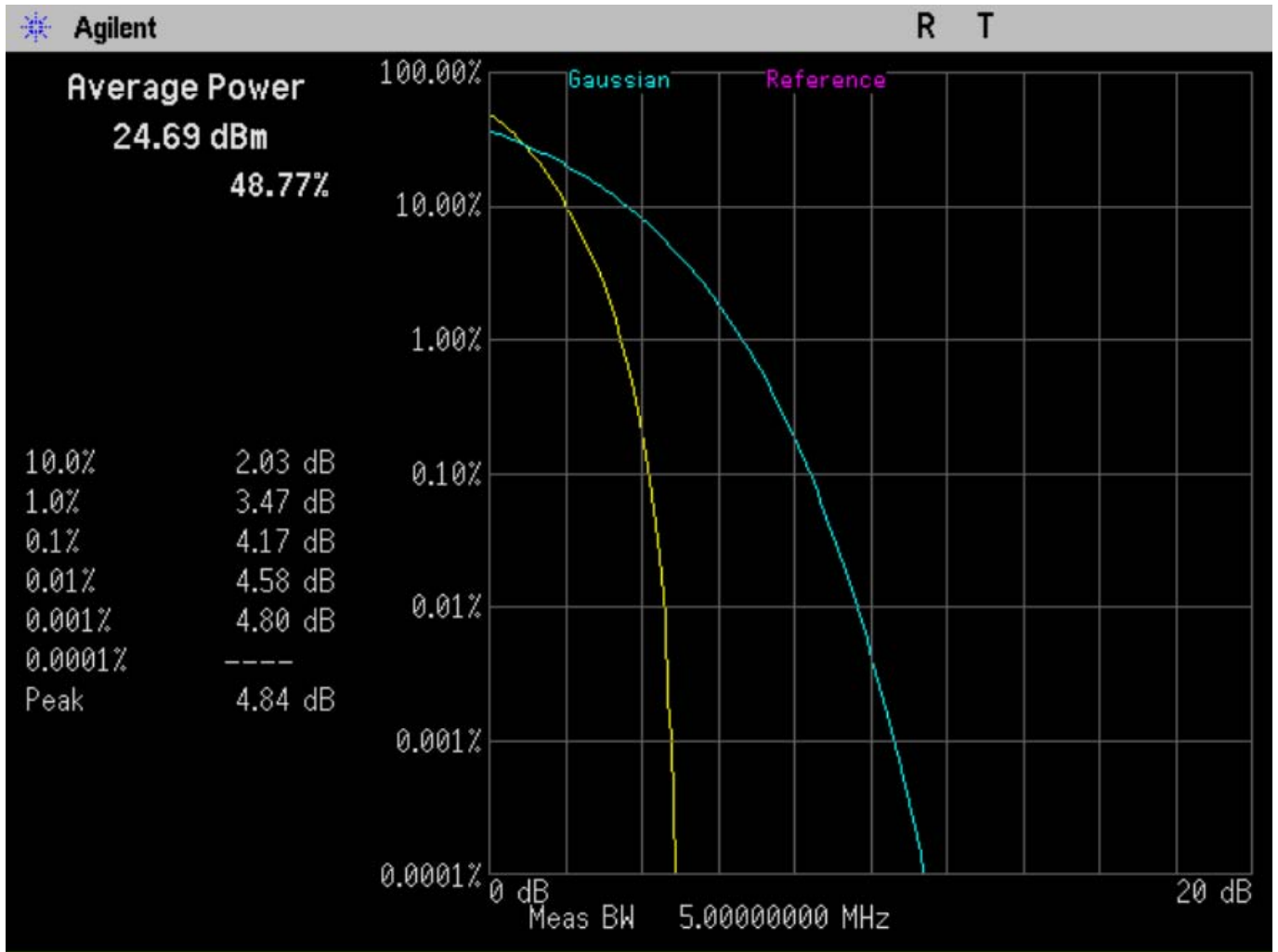
Figure 8-1 CCDF @ CH 600
