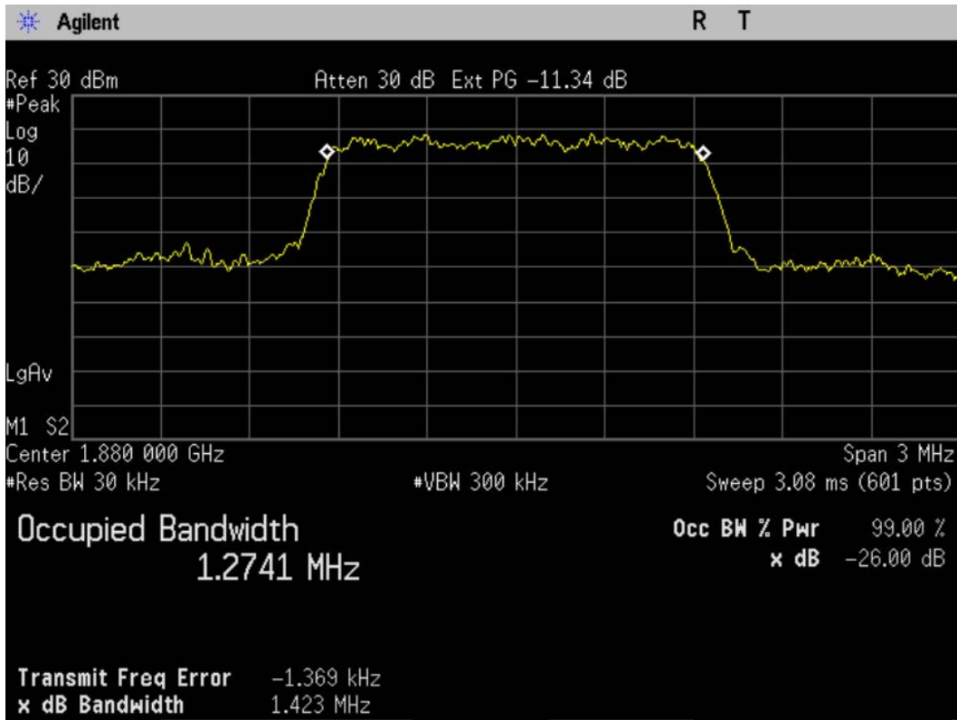
Figure 8-4 CDMA 1900 @ CH 600
