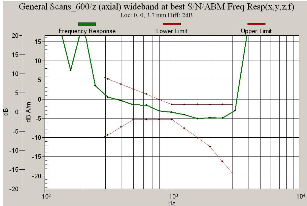
Figure 9.2c CDMA 1900, Slide Close, Frequency Response
