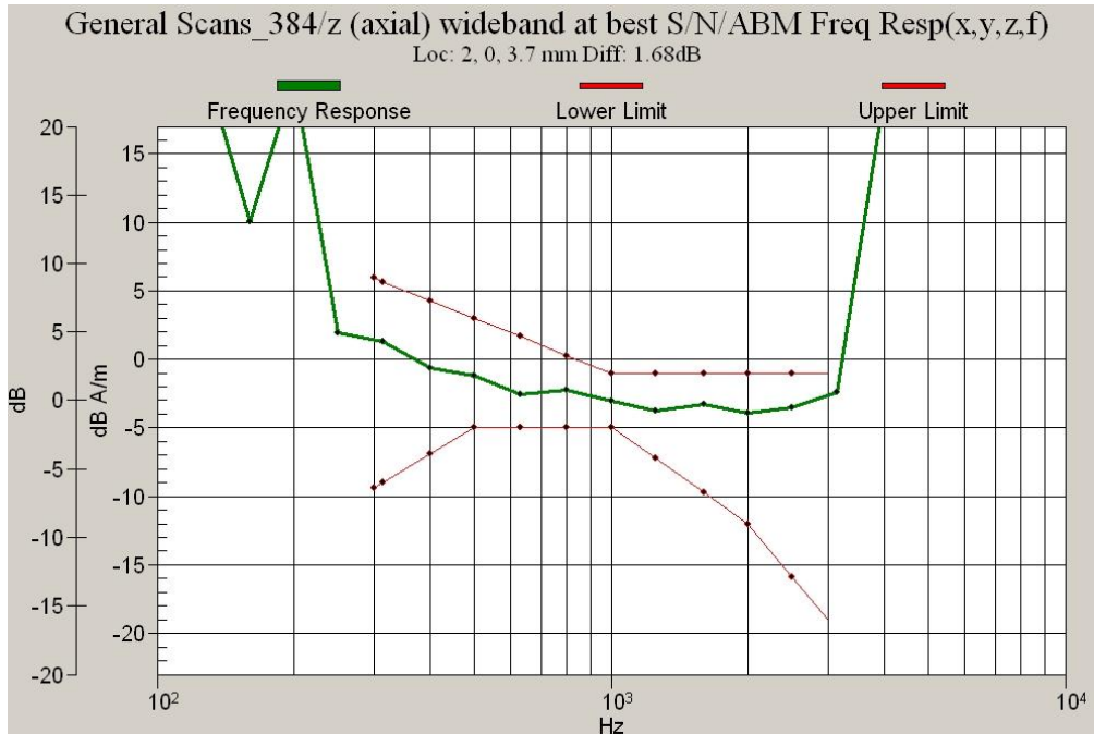
Figure 9.2b CDMA 800 BC-0, Slide Close, Frequency Response
