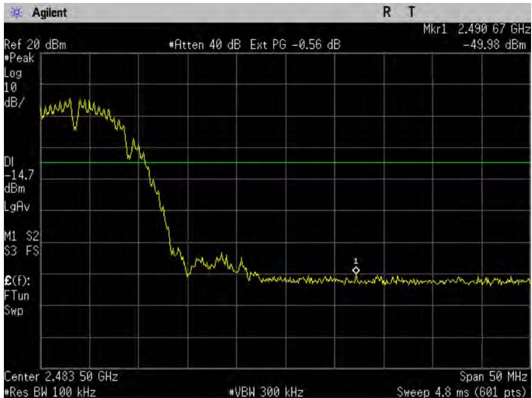
Figure 9-1b: High band edge, 802.11b, ch11.
