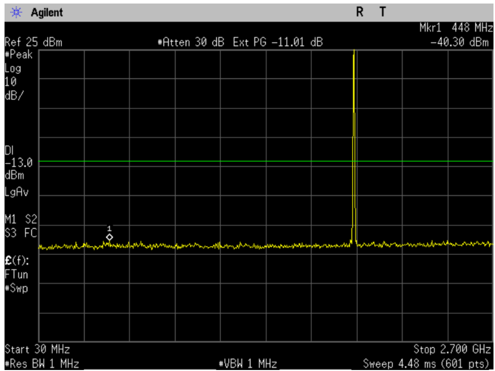
Figure 10-2a CDMA 1900 - Conducted Spurious Emission (CH 600)
