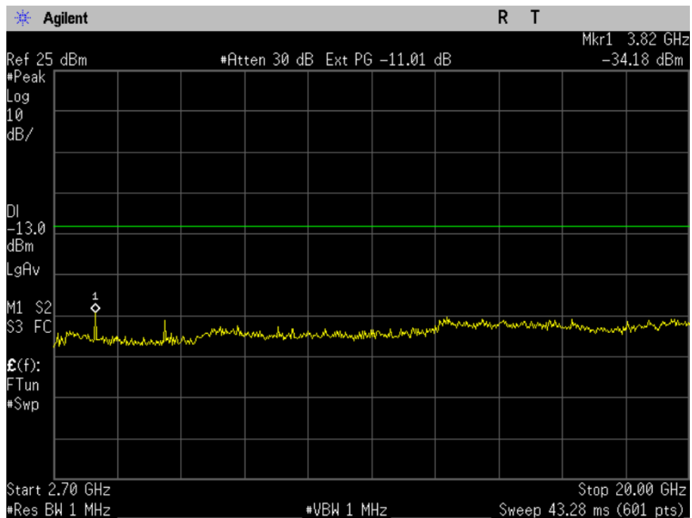
Figure 10-3b CDMA 1900 - Conducted Spurious Emission (CH 1175)
