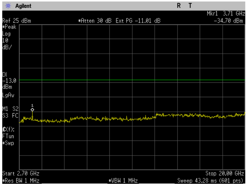
Figure 10-1b CDMA 1900 - Conducted Spurious Emission (CH 25)
