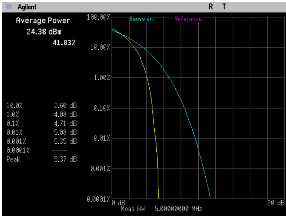
Figure 8-1 CCDF @ CH 600
