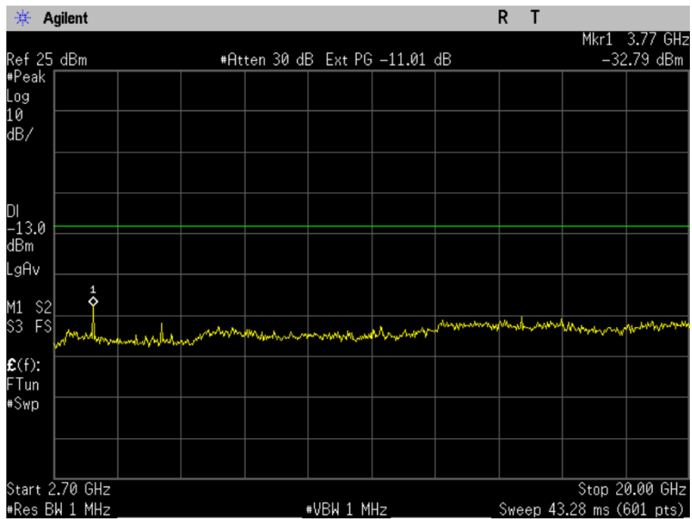
Figure 10-2b CDMA 1900 - Conducted Spurious Emission (CH 600)
