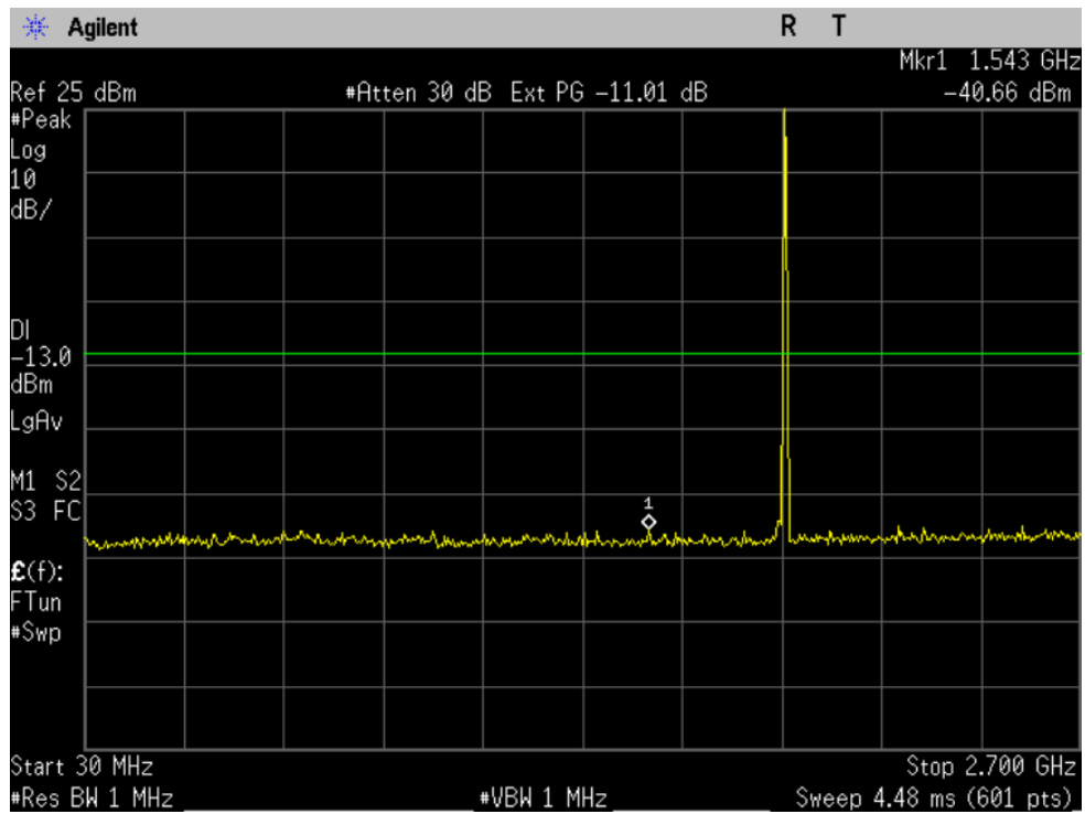
Figure 10-3a CDMA 1900 - Conducted Spurious Emission (CH 1175)
