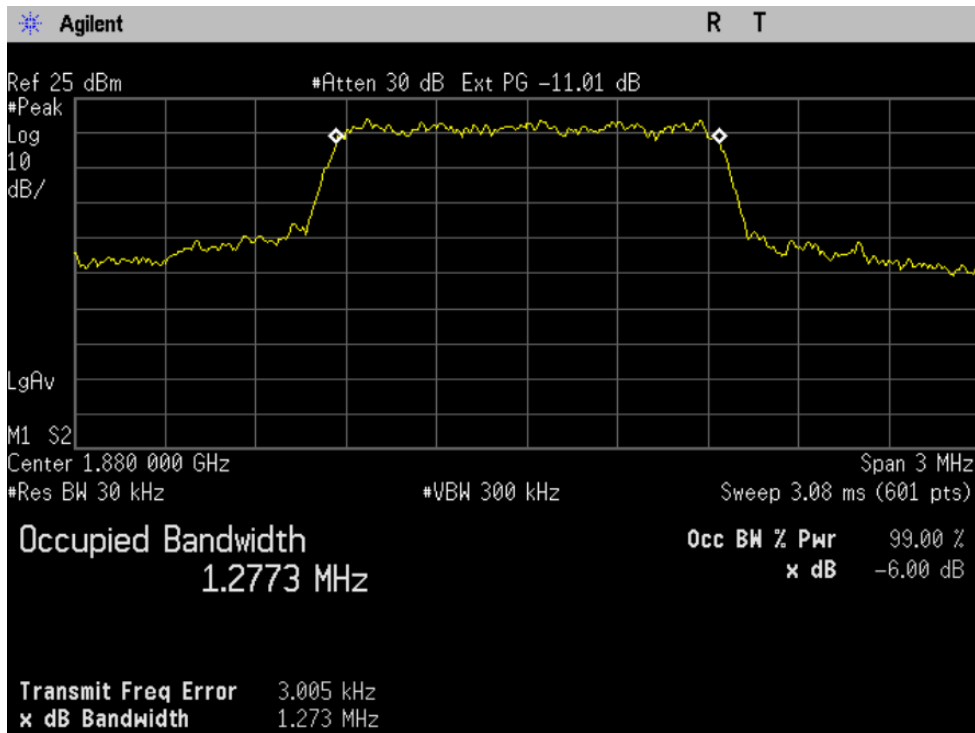
Figure 9-1 CDMA 1900 @ CH 600
