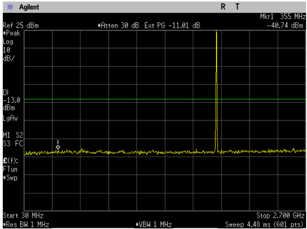
Figure 10-1a CDMA 1900 - Conducted Spurious Emission (CH 25)
