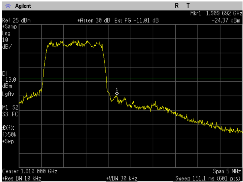
Figure 9-3 CDMA 1900 Upper Band Edge @ CH 1175
