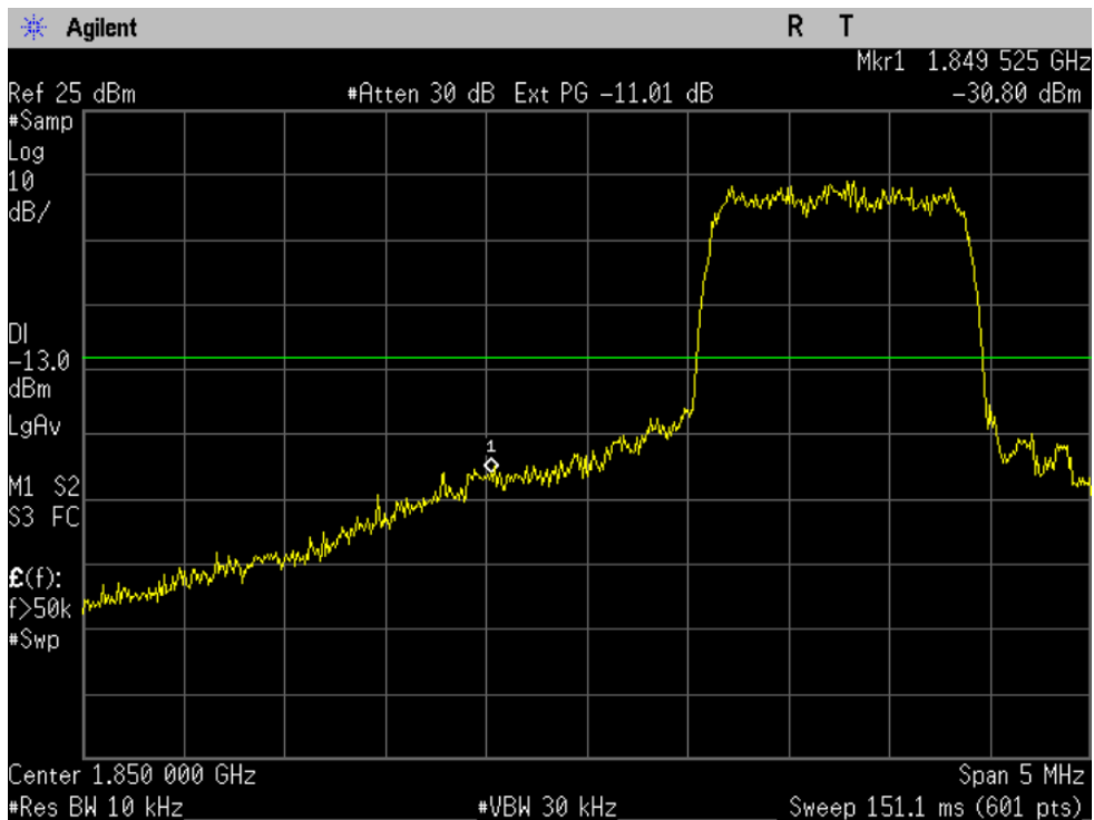
Figure 9-2 CDMA 1900 Lower Band Edge @ CH 25
