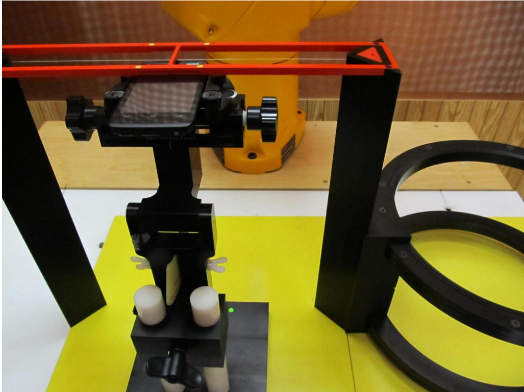
Figure 1a – HAC T-Coil Test Setup
