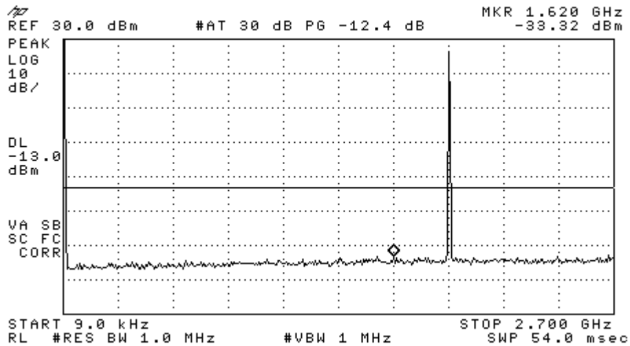
Figure 9-5a CDMA 1900 - Conducted Spurious Emission (CH 600)
