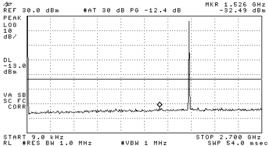
Figure 9-4a CDMA 1900 - Conducted Spurious Emission (CH 25)
