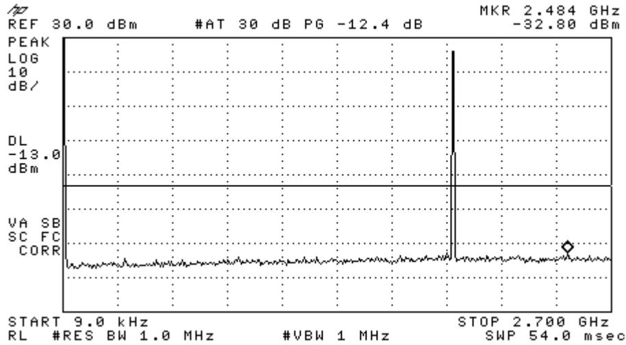
Figure 9-6a CDMA 1900 - Conducted Spurious Emission (CH 1175)
