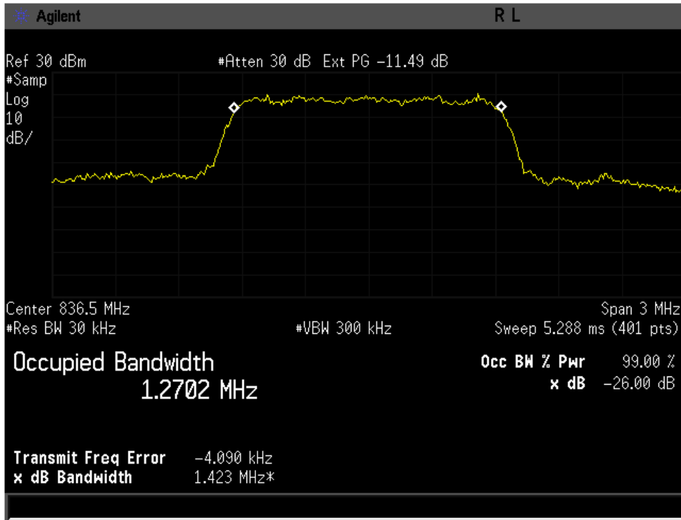
Figure 8-1 CDMA 800 @ CH 384
