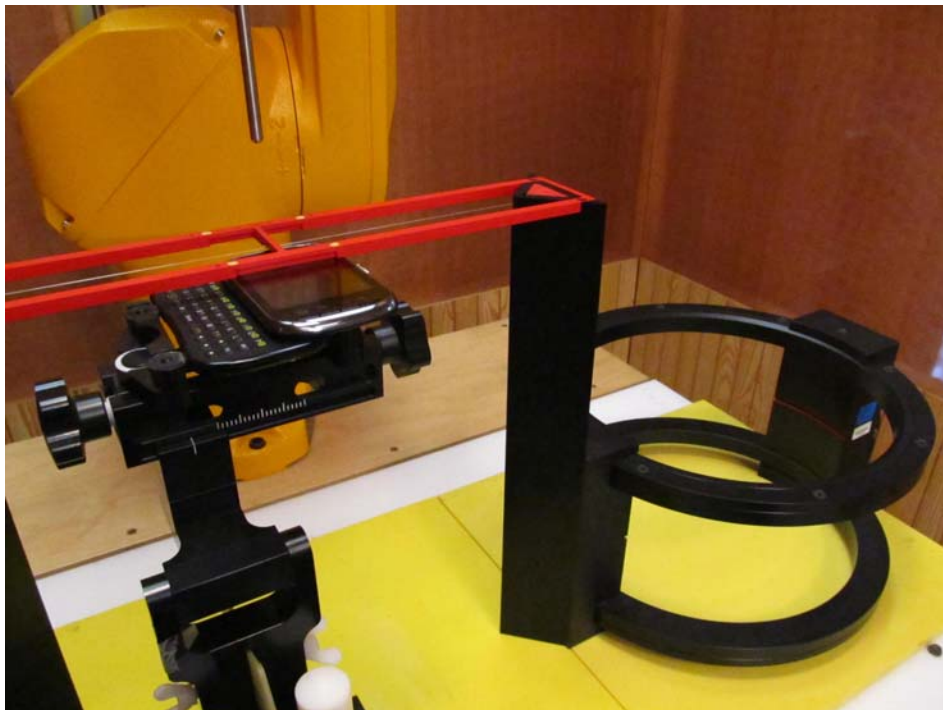
Figure 1b – HAC T-Coil Test Setup, Phone Slide Open
