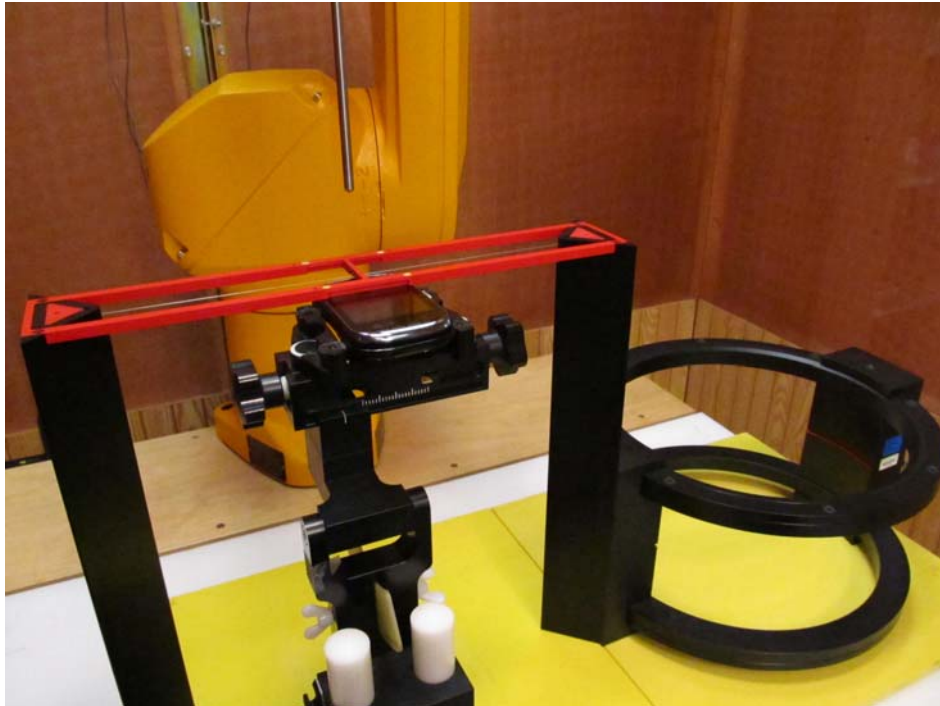
Figure 1a – HAC T-Coil Test Setup, Phone Slide Close
