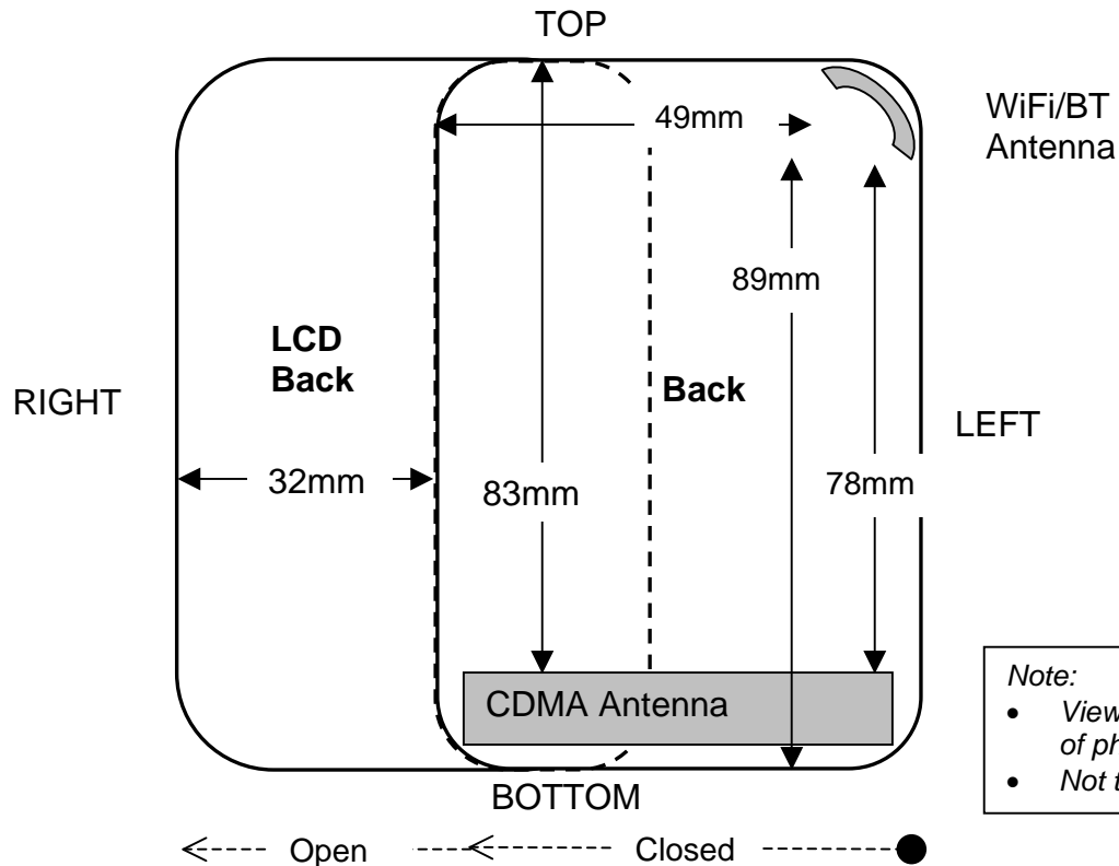
Figure 4.7 Antenna Distance to device edges
