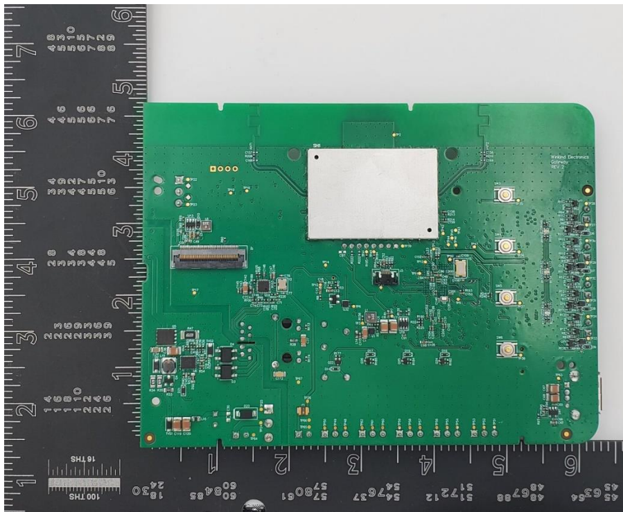
EA Pro Gateway PCB Top (Shield will normally be installed)
