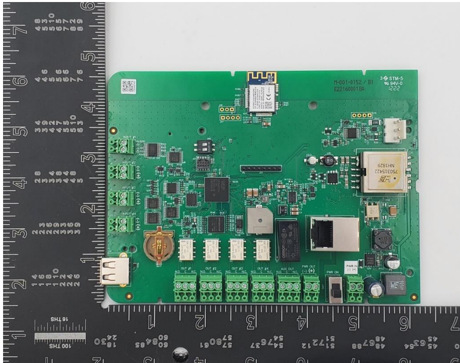
EA Pro Gateway PCB Bottom
